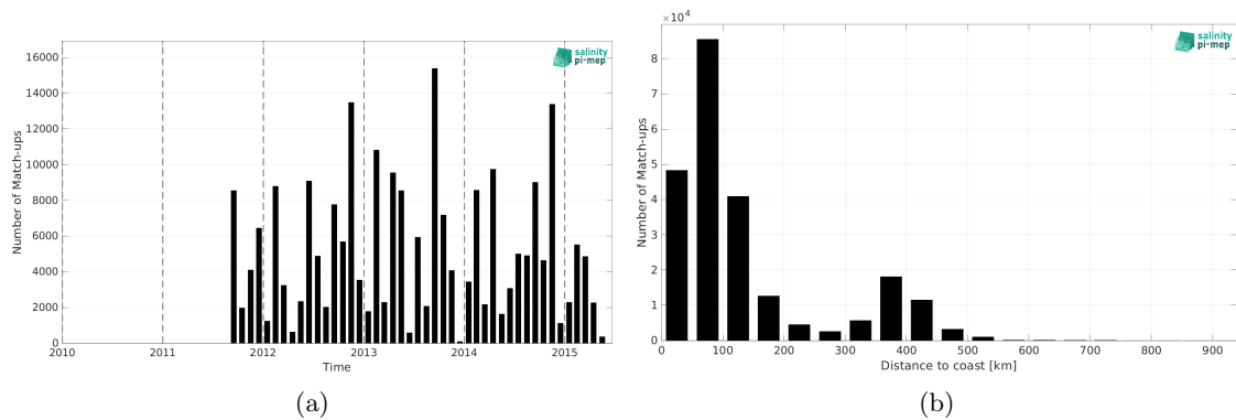
Figure 1: Number of match-ups between ICES and Aquarius SSS L4 OI v5 - Monthly (IPRC) SSS as a function of time (a) and as function of the distance to coast (b) over the SMOS coastal zone (<800km) 60N-60S Pi-MEP region and for the full satellite product period.
