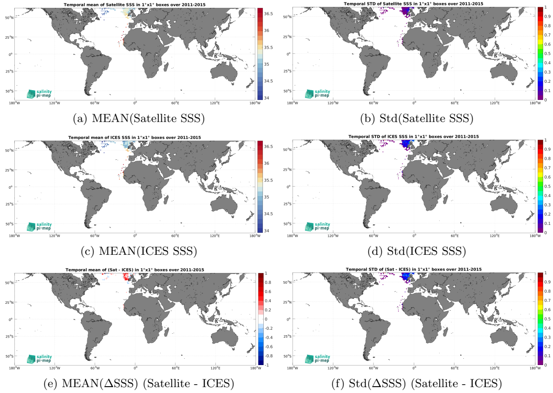
Figure 6: Temporal mean (left) and Std (right) of SSS from Aquarius SSS L4 OI v5 - Monthly (IPRC) (top), ICES (middle), and of \Delta SSS (Satellite - ICES). Only match-up pairs are used to generate these maps.
