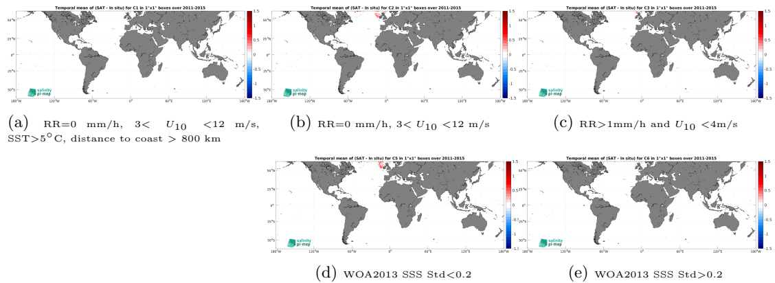
Figure 12: Temporal mean gridded over spatial boxes of size 1^\circ \times 1^\circ of \Delta\text{SSS} (Aquarius SSS L4 OI v5 - Monthly (IPRC) - ICES) for 5 different subdatasets corresponding to:RR=0 mm/h, 3 < U_{10} < 12 m/s, SST >5^\circ\text{C} , distance to coast > 800 km (a), RR=0 mm/h, 3 < U_{10} < 12 m/s (b), RR >1 mm/h and U_{10} < 4 m/s (c), WOA2013 SSS Std <0.2 (d), WOA2013 SSS Std >0.2 (e).
