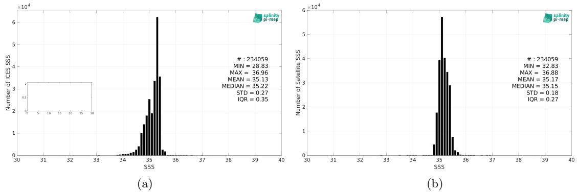
Figure 2: Histograms of SSS from ICES (a) and Aquarius SSS L4 OI v5 - Monthly (IPRC) (b) considering all match-up pairs per bins of 0.1 over the SMOS coastal zone (<800km) 60N-60S Pi-MEP region and for the full satellite product period.
