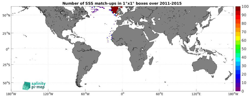
Figure 4: Number of SSS match-ups between ICES SSS and the Aquarius SSS L4 OI v5 - Monthly (IPRC) SSS product for the SMOS coastal zone ( <800\text{km} ) 60N-60S Pi-MEP region over 1^\circ \times 1^\circ boxes and for the full satellite product period.
