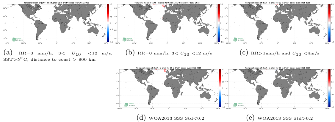
Figure 12: Temporal mean gridded over spatial boxes of size 1^\circ \times 1^\circ of \Delta SSS (Aquarius SSS L4 OI v5 - Monthly (IPRC) - ICES) for 5 different subdatasets corresponding to:RR=0 mm/h, 3 < U_{10} < 12 m/s, SST >5^\circ\text{C} , distance to coast > 800 km (a), RR=0 mm/h, 3 < U_{10} < 12 m/s (b), RR >1 mm/h and U_{10} < 4 m/s (c), WOA2013 SSS Std <0.2 (d), WOA2013 SSS Std >0.2 (e).
