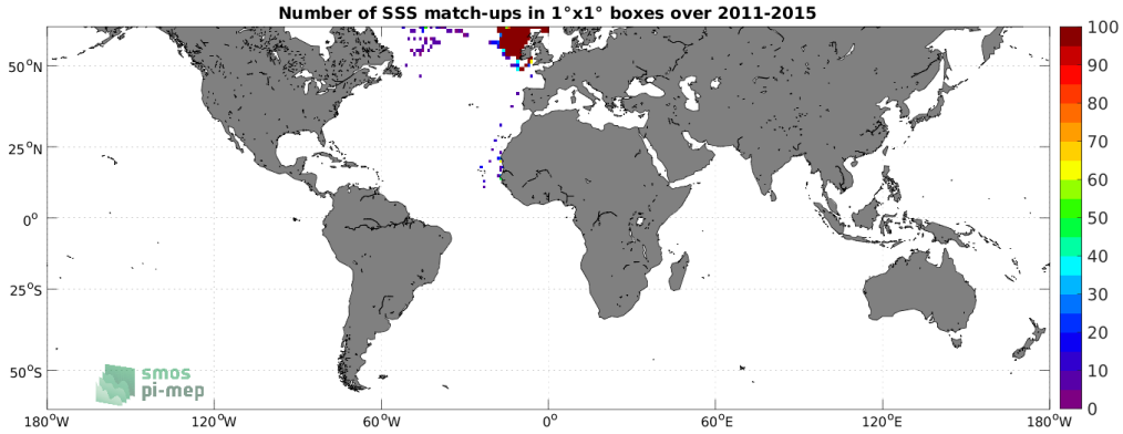
Figure 4: Number of SSS match-ups between ICES SSS and the Aquarius SSS L4 OI v5 - Monthly (IPRC) SSS product for the SMOS coastal zone (<800km) 60N-60S Pi-MEP region over 1^\circ \times 1^\circ boxes and for the full satellite product period.
