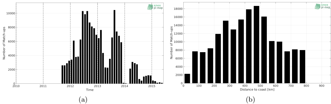
Figure 1: Number of match-ups between Surface drifters and Aquarius-L4-IPRC-V5-MONTHLY SSS as a function of time (a) and as function of the distance to coast (b) over the SMOS coastal zone (<800km) 60N-60S Pi-MEP region and for the full satellite product period.
