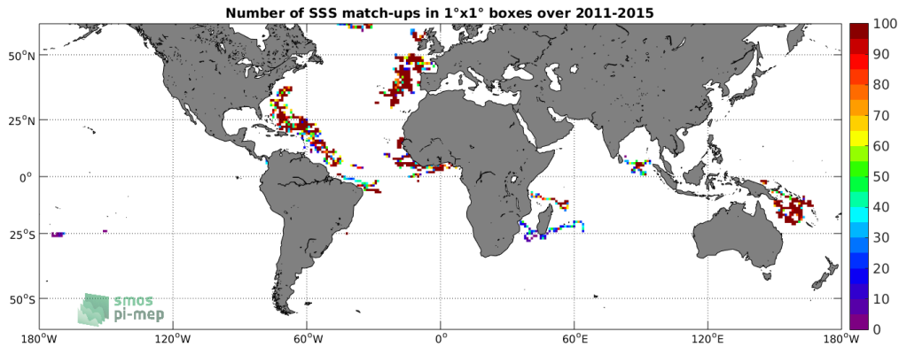
Figure 3: Number of SSS match-ups between Surface drifters SSS and the Aquarius-L4-IPRC-V5-MONTHLY SSS product for the SMOS coastal zone (<800km) 60N-60S Pi-MEP region over 1°x1° boxes and for the full satellite product period.
