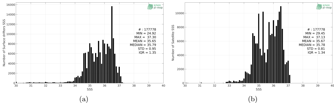
Figure 2: Histograms of SSS from Surface drifters (a) and Aquarius-L4-IPRC-V5-MONTHLY (b) considering all match-up pairs per bins of 0.1 over the SMOS coastal zone (<800km) 60N-60S Pi-MEP region and for the full satellite product period.
