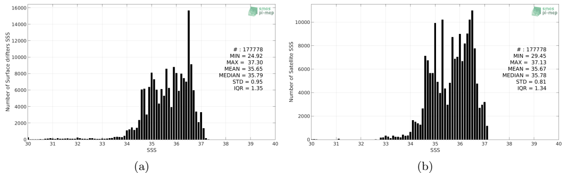
Figure 2: Histograms of SSS from Surface drifters (a) and Aquarius-L4-IPRC-V5-MONTHLY (b) considering all match-up pairs per bins of 0.1 over the SMOS coastal zone ( \geq 800 km) 60N-60S Pi-MEP region and for the full satellite product period.
