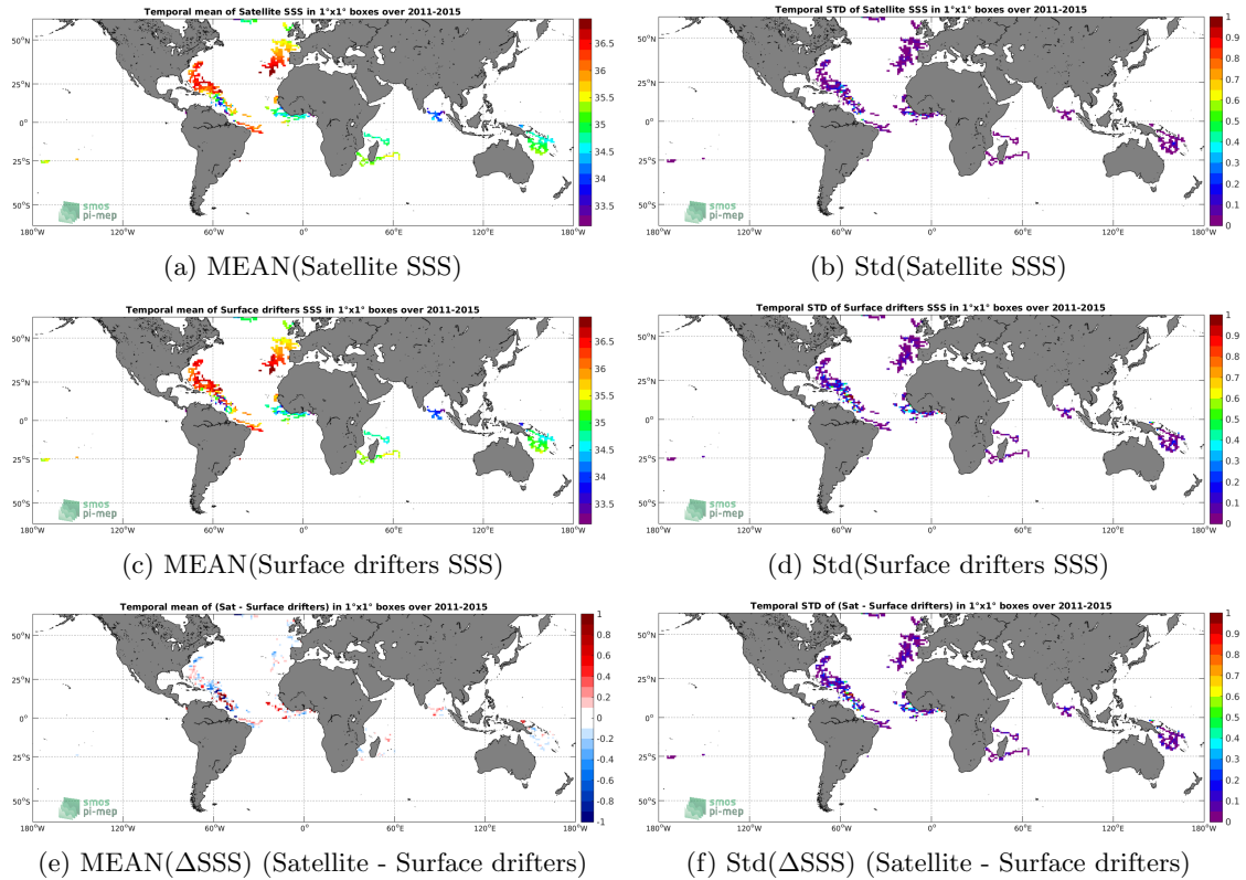
Figure 5: Temporal mean (left) and Std (right) of SSS from Aquarius-L4-IPRC-V5-MONTHLY (top), Surface drifters (middle), and of \Delta SSS (Satellite - Surface drifters). Only match-up pairs are used to generate these maps.
