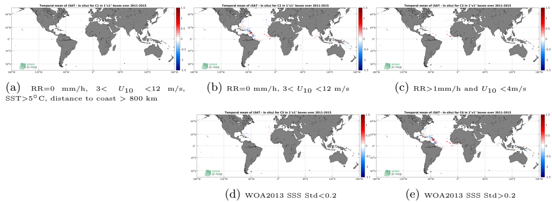
Figure 11: Temporal mean gridded over spatial boxes of size 1^\circ \times 1^\circ of \Delta SSS (Aquarius-L4-IPRC-V5-MONTHLY - Surface drifters) for 5 different subdatasets corresponding to:RR=0 mm/h, 3 < U_{10} < 12 m/s, SST >5^\circ\text{C} , distance to coast > 800 km (a), RR=0 mm/h, 3 < U_{10} < 12 m/s (b), RR >1 mm/h and U_{10} < 4 m/s (c), WOA2013 SSS Std <0.2 (d), WOA2013 SSS Std >0.2 (e).
