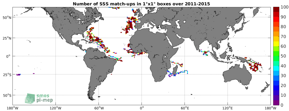
Figure 3: Number of SSS match-ups between Surface drifters SSS and the Aquarius-L4-IPRC-V5-MONTHLY SSS product for the SMOS coastal zone ( \geq 800\text{km} ) 60N-60S Pi-MEP region over 1^\circ \times 1^\circ boxes and for the full satellite product period.
