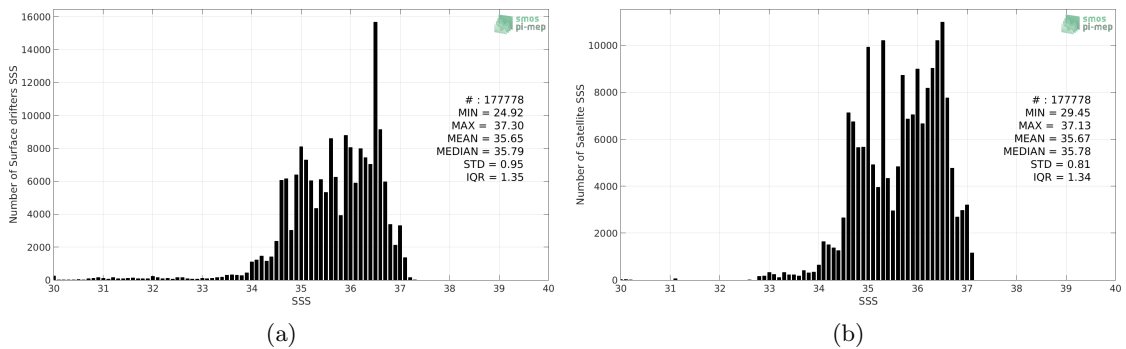
Figure 2: Histograms of SSS from Surface drifters (a) and Aquarius-L4-IPRC-V5-MONTHLY (b) considering all match-up pairs per bins of 0.1 over the SMOS coastal zone ( \geq 800 km) 60N-60S Pi-MEP region and for the full satellite product period.
