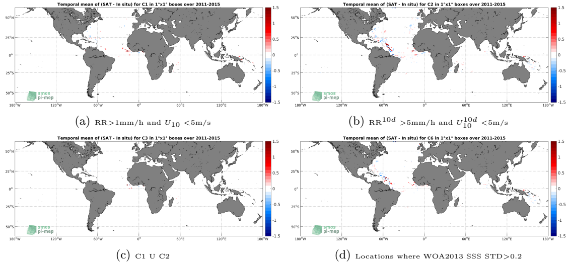
Figure 11: Temporal mean gridded over spatial boxes of size 1^\circ \times 1^\circ of \Delta SSS (Aquarius-L4-IPRC-V5-MONTHLY - Surface drifters) for 4 different subdatasets corresponding to: RR > 1mm/h and U_{10} < 5\text{m/s} (a), RR^{10d} > 5\text{mm/h} and U_{10}^{10d} < 5\text{m/s} (b), C1 U C2 (c), Locations where WOA2013 SSS STD > 0.2 (d).
