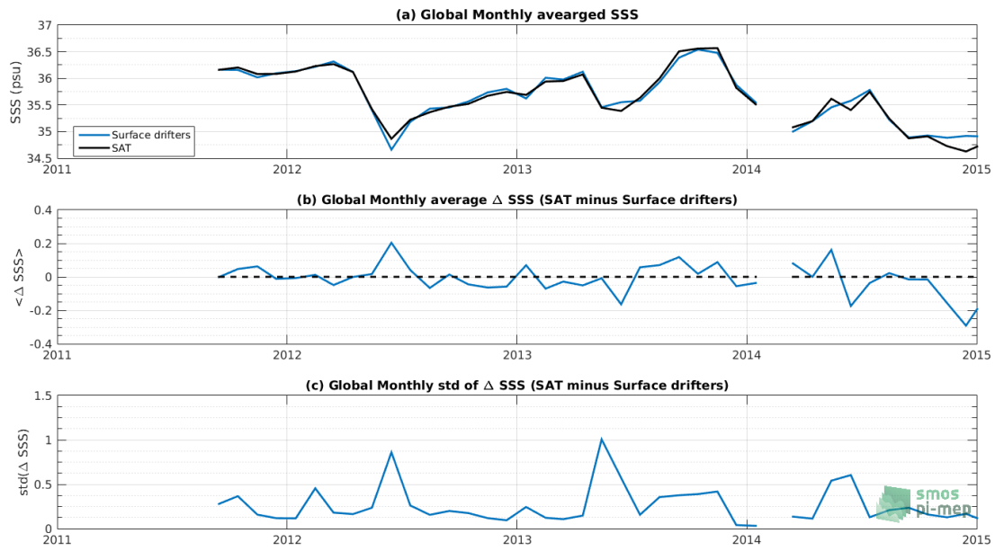
Figure 6: Time series of the monthly averaged mean SSS (top), mean \Delta SSS (Satellite - Surface drifters) and STD of \Delta SSS (Satellite - Surface drifters) over the SMOS coastal zone ( \pm 800\text{km} ) 60N-60S Pi-MEP region considering all match-ups collected by the Pi-MEP platform.
