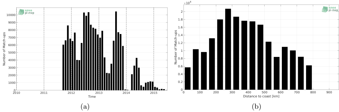
Figure 1: Number of match-ups between Surface drifters and Aquarius-L4-IPRC-V5-MONTHLY SSS as a function of time (a) and as function of the distance to coast (b) over the SMOS coastal zone ( \approx 800 km) 60N-60S Pi-MEP region and for the full satellite product period.
