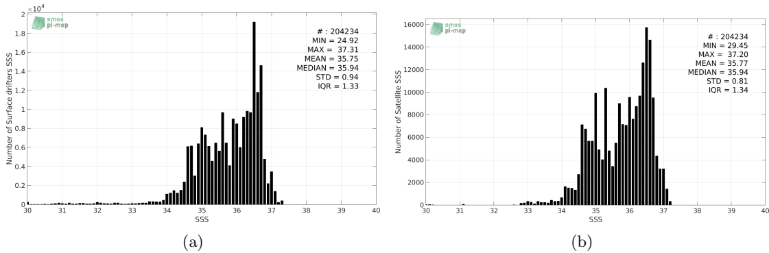
Figure 2: Histograms of SSS from Surface drifters (a) and Aquarius-L4-IPRC-V5-MONTHLY (b) considering all match-up pairs per bins of 0.1 over the SMOS coastal zone ( \approx 800 km) 60N-60S Pi-MEP region and for the full satellite product period.
