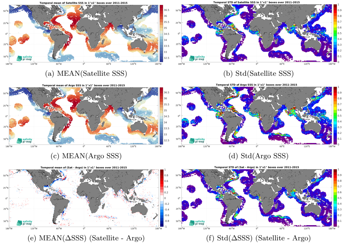
Figure 7: Temporal mean (left) and Std (right) of SSS from Aquarius SSS L4 OI v5 - Monthly (IPRC) (top), Argo (middle), and of \Delta SSS (Satellite - Argo). Only match-up pairs are used to generate these maps.
