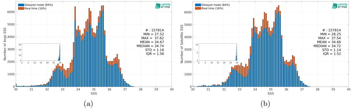
Figure 3: Histograms of SSS from Argo (a) and Aquarius SSS L4 OI v5 - Monthly (IPRC) (b) considering all match-up pairs per bins of 0.1 over the SMOS coastal zone (<800km) 60N-60S Pi-MEP region and for the full satellite product period.
