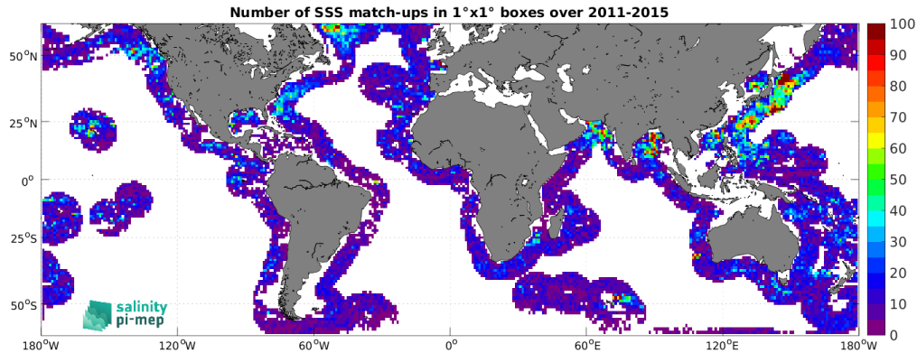
Figure 5: Number of SSS match-ups between Argo SSS and the Aquarius SSS L4 OI v5 - Monthly (IPRC) SSS product for the SMOS coastal zone (<800km) 60N-60S Pi-MEP region over 1^\circ \times 1^\circ boxes and for the full satellite product period.
