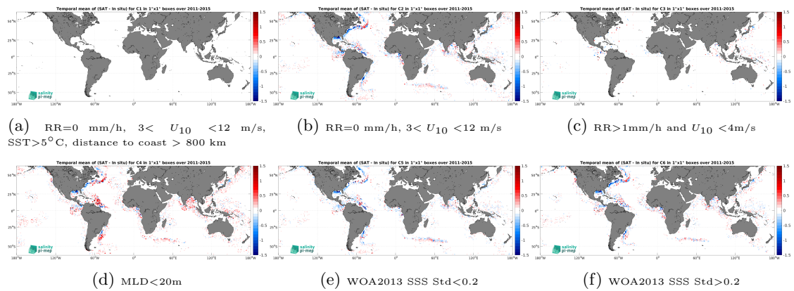
Figure 14: Temporal mean gridded over spatial boxes of size 1^\circ \times 1^\circ of \Delta SSS (Aquarius SSS L4 OI v5 - Monthly (IPRC) - Argo) for 6 different subdatasets corresponding to:RR=0 mm/h, 3 < U_{10} < 12 m/s, SST > 5^\circ\text{C} , distance to coast > 800 km (a), RR=0 mm/h, 3 < U_{10} < 12 m/s (b), RR > 1 mm/h and U_{10} < 4 m/s (c),MLD < 20 m (d),WOA2013 SSS Std < 0.2 (e),WOA2013 SSS Std > 0.2 (f).
