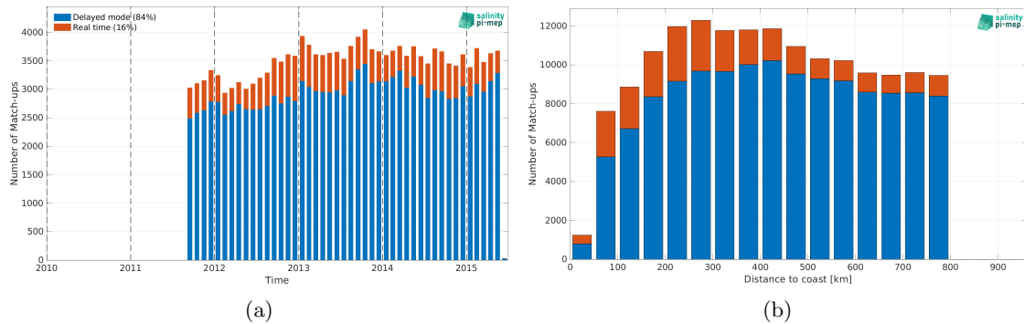
Figure 2: Number of match-ups between Argo and Aquarius SSS L4 OI v5 - Monthly (IPRC) SSS as a function of time (a) and as function of the distance to coast (b) over the SMOS coastal zone (<800km) 60N-60S Pi-MEP region and for the full satellite product period.
