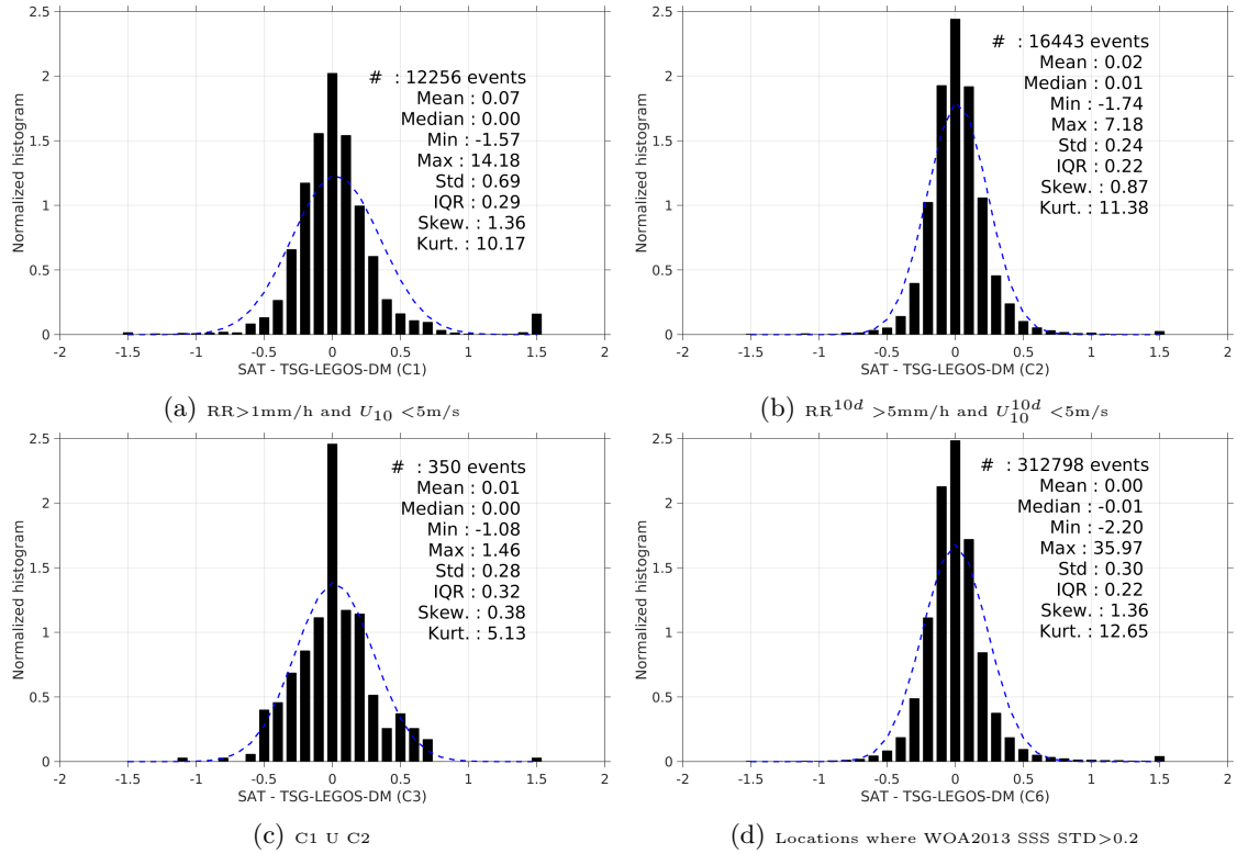
Figure 13: Normalized histogram of \Delta\text{SSS} (Aquarius-L4-IPRC-V4-WEEKLY - TSG-LEGOS-DM) for 6 different subdatasets corresponding to: RR > 1mm/h and U_{10} < 5\text{m/s} (a), \text{RR}^{10d} > 5\text{mm/h} and U_{10}^{10d} < 5\text{m/s} (b), C1 U C2 (c), Locations where WOA2013 SSS STD > 0.2 (d).
