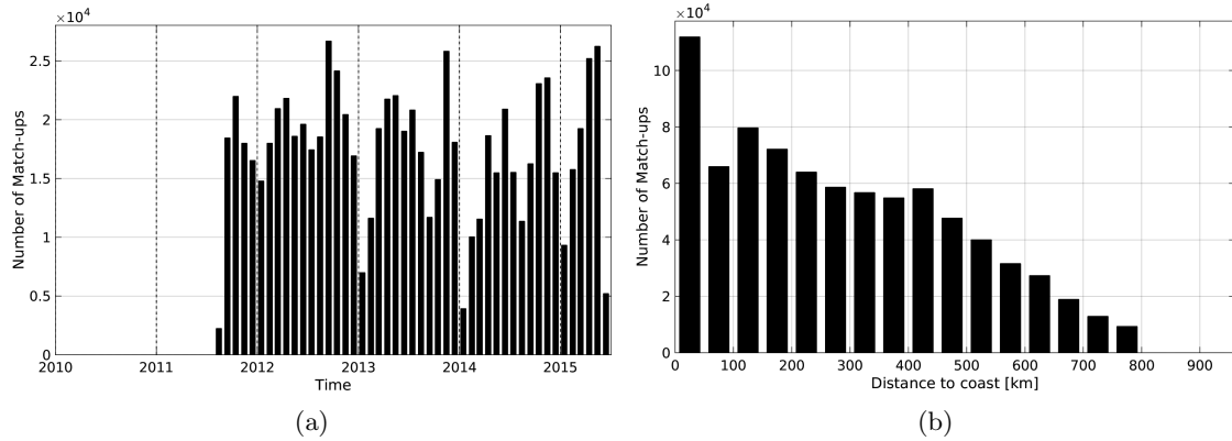
Figure 1: Number of match-ups between TSG-LEGOS-DM and Aquarius-L4-IPRC-V4-WEEKLY SSS as a function of time (a) and as function of the distance to coast (b) over the SMOS coastal zone ( \approx 800 km) 60N-60S Pi-MEP region and for the full satellite product period.
