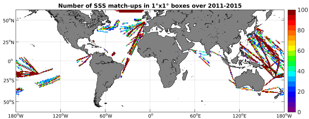
Figure 4: Number of SSS match-ups between TSG-LEGOS-DM SSS and the Aquarius-L4-IPRC-V4-WEEKLY SSS product for the SMOS coastal zone ( \pm 800\text{km} ) 60N-60S Pi-MEP region over 1^\circ \times 1^\circ boxes and for the full satellite product period.
