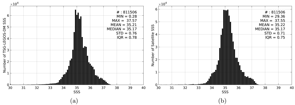
Figure 2: Histograms of SSS from TSG-LEGOS-DM (a) and Aquarius-L4-IPRC-V4-WEEKLY (b) considering all match-up pairs per bins of 0.1 over the SMOS coastal zone ( \approx 800 km) 60N-60S Pi-MEP region and for the full satellite product period.
