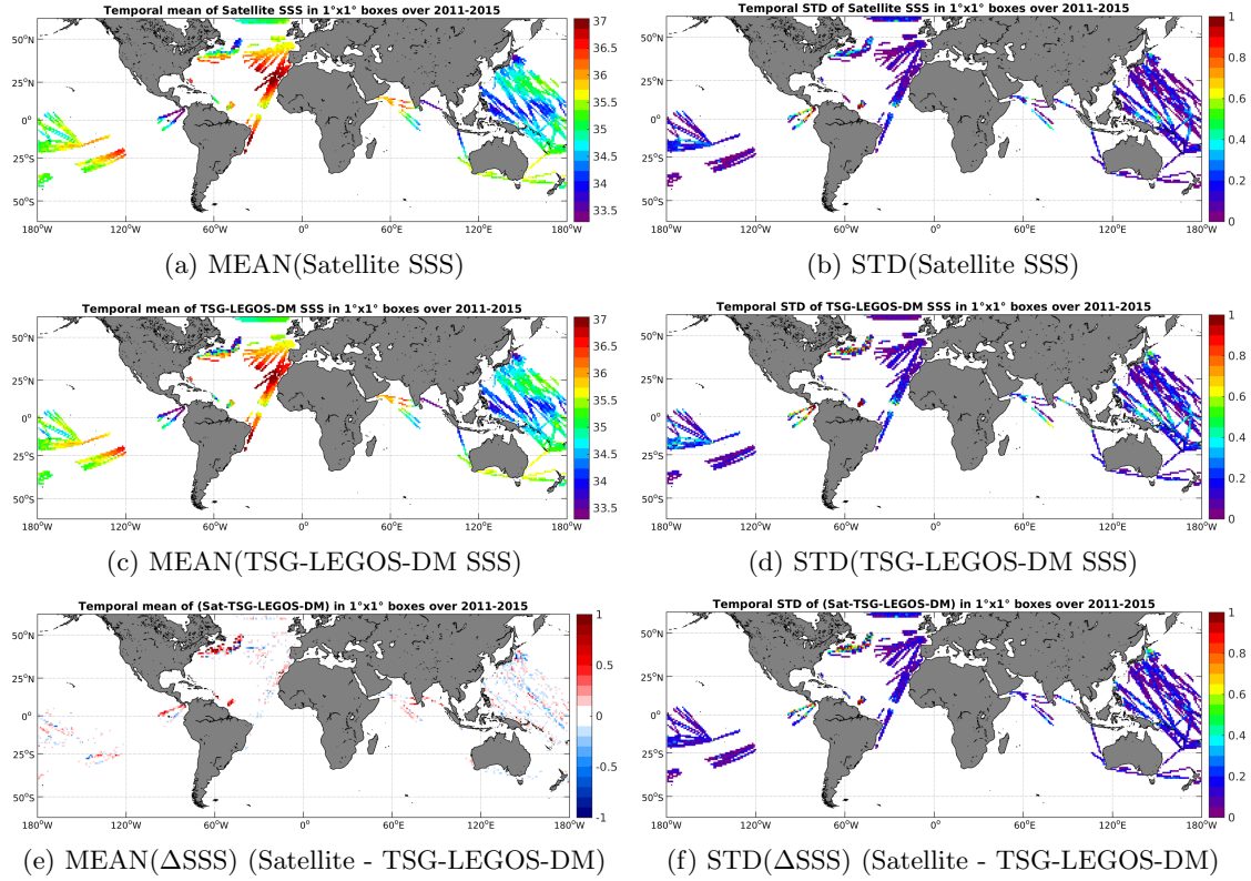
Figure 6: Temporal mean (left) and STD (right) of SSS from Aquarius-L4-IPRC-V4-WEEKLY (top), TSG-LEGOS-DM (middle), and of \Delta SSS (Satellite - TSG-LEGOS-DM). Only match-up pairs are used to generate these maps.
