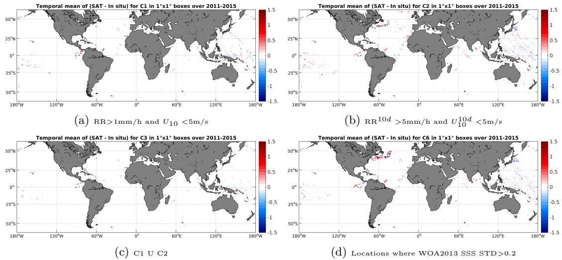
Figure 12: Temporal mean gridded over spatial boxes of size 1^\circ \times 1^\circ of \Delta SSS (Aquarius-L4-IPRC-V4-WEEKLY - TSG-LEGOS-DM) for 4 different subdatasets corresponding to: RR > 1\text{mm/h} and U_{10} < 5\text{m/s} (a), RR^{10d} > 5\text{mm/h} and U_{10}^{10d} < 5\text{m/s} (b), C1 U C2 (c), Locations where WOA2013 SSS STD > 0.2 (d).
