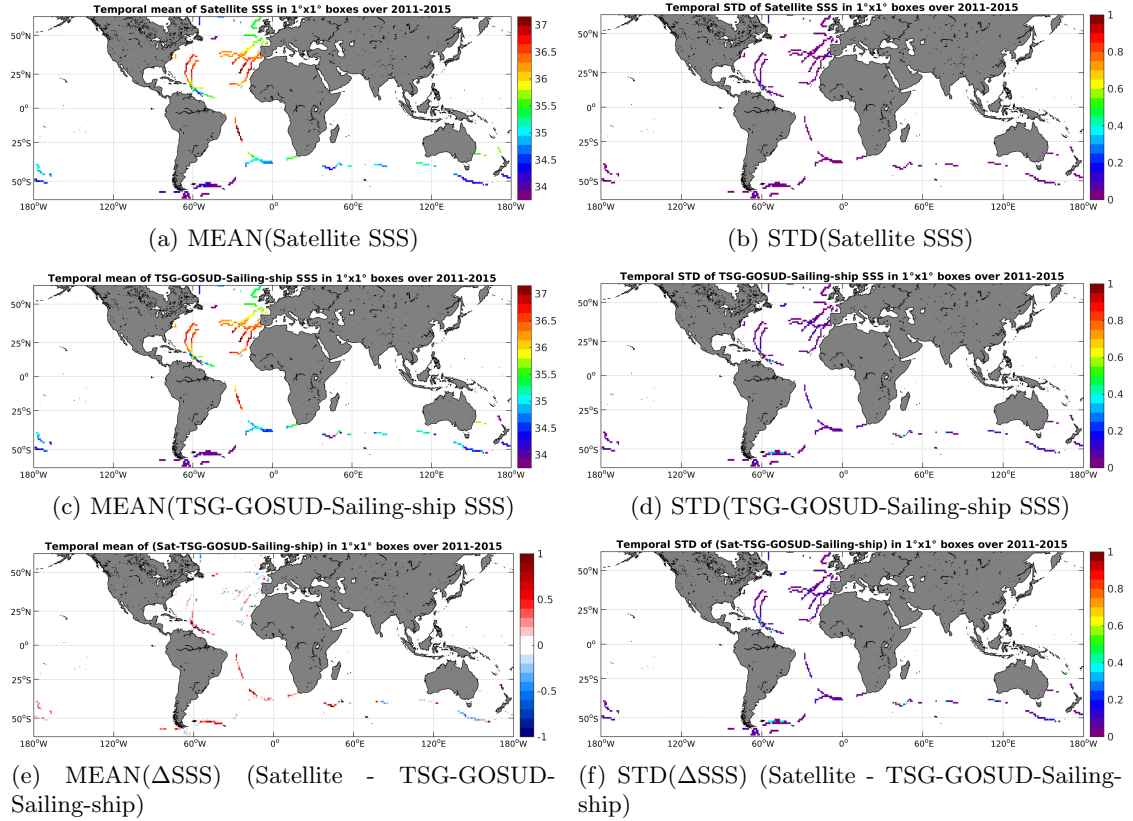
Figure 6: Temporal mean (left) and STD (right) of SSS from Aquarius-L4-IPRC-V4-WEEKLY (top), TSG-GOSUD-Sailing-ship (middle), and of \Delta SSS (Satellite - TSG-GOSUD-Sailing-ship). Only match-up pairs are used to generate these maps.
