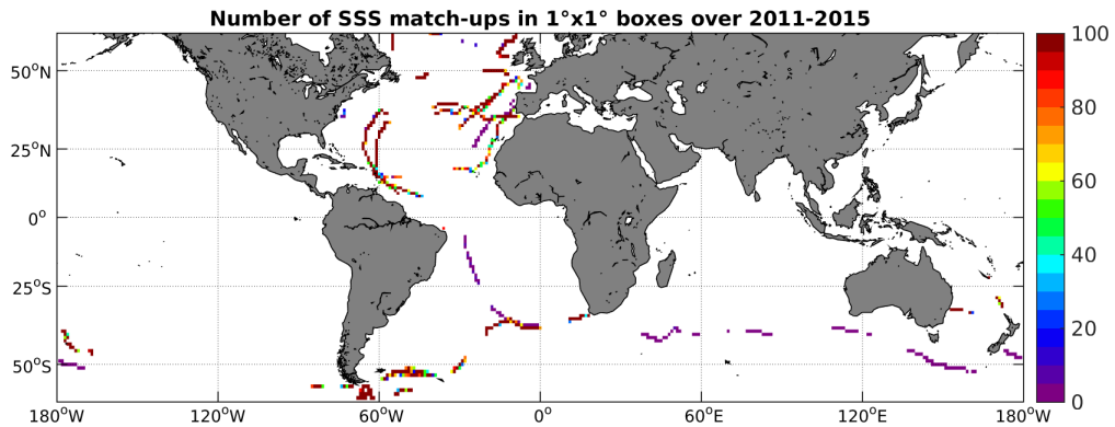
Figure 4: Number of SSS match-ups between TSG-GOSUD-Sailing-ship SSS and the Aquarius-L4-IPRC-V4-WEEKLY SSS product for the SMOS coastal zone ( \pm 800\text{km} ) 60N-60S Pi-MEP region over 1^\circ \times 1^\circ boxes and for the full satellite product period.
