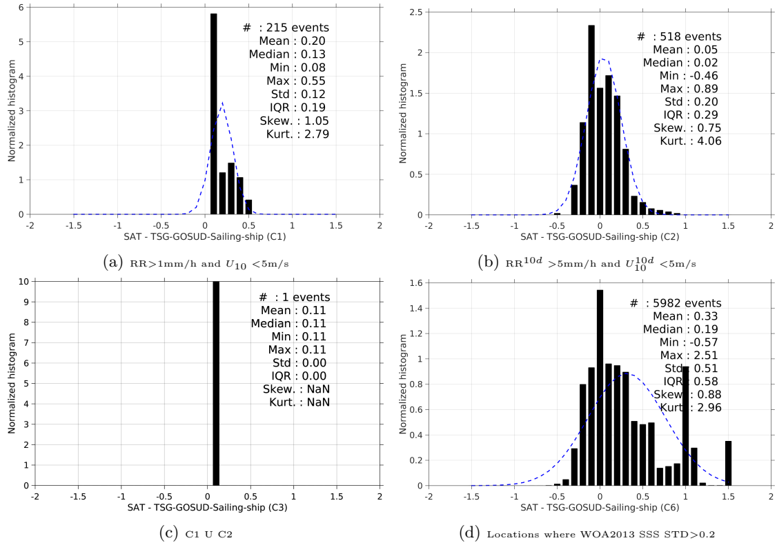
Figure 13: Normalized histogram of \Delta\text{SSS} (Aquarius-L4-IPRC-V4-WEEKLY - TSG-GOSUD-Sailing-ship) for 6 different subdatasets corresponding to: RR > 1mm/h and U_{10} < 5\text{m/s} (a), RR^{10d} > 5\text{mm/h} and U_{10}^{10d} < 5\text{m/s} (b), C1 U C2 (c), Locations where WOA2013 SSS STD > 0.2 (d).
