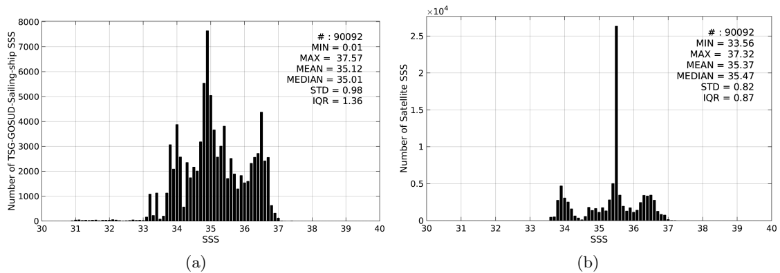
Figure 2: Histograms of SSS from TSG-GOSUD-Sailing-ship (a) and Aquarius-L4-IPRC-V4-WEEKLY (b) considering all match-up pairs per bins of 0.1 over the SMOS coastal zone ( \leq 800 km) 60N-60S Pi-MEP region and for the full satellite product period.
