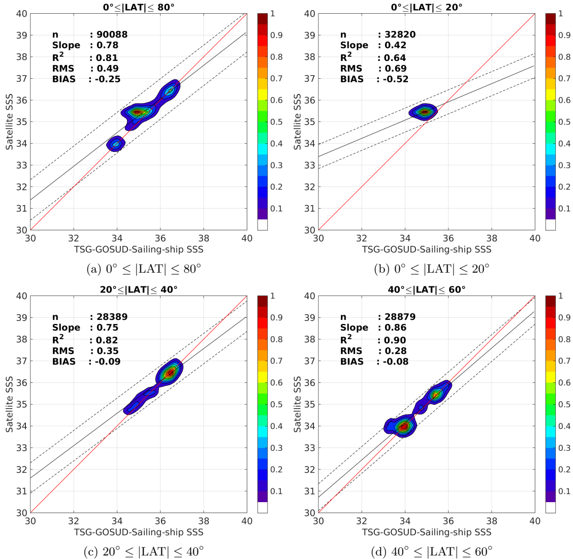
Figure 9: Contour maps of the concentration of Aquarius-L4-IPRC-V4-WEEKLY SSS (y-axis) versus TSG-GOSUD-Sailing-ship SSS (x-axis) at match-up pairs for different latitude bands. For each plot, the red line shows x=y . The black thin and dashed lines indicate a linear fit through the data cloud and the \pm 95\% confidence levels, respectively. The number match-up pairs n , the slope and R^2 coefficient of the linear fit, the root mean square (RMS) and the mean bias between satellite and in situ data are indicated for each latitude band in each plots.
