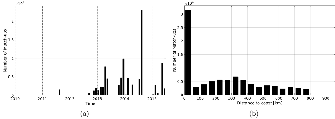
Figure 1: Number of match-ups between TSG-GOSUD-Sailing-ship and Aquarius-L4-IPRC-V4-WEEKLY SSS as a function of time (a) and as function of the distance to coast (b) over the SMOS coastal zone ( \leq 800 km) 60N-60S Pi-MEP region and for the full satellite product period.
