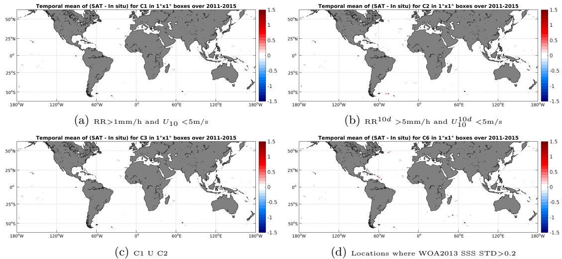
Figure 12: Temporal mean gridded over spatial boxes of size 1^\circ \times 1^\circ of \Delta SSS (Aquarius-L4-IPRC-V4-WEEKLY - TSG-GOSUD-Sailing-ship) for 4 different subdatasets corresponding to: RR > 1\text{mm/h} and U_{10} < 5\text{m/s} (a), RR^{10d} > 5\text{mm/h} and U_{10}^{10d} < 5\text{m/s} (b), C1 U C2 (c), Locations where WOA2013 SSS STD > 0.2 (d).
