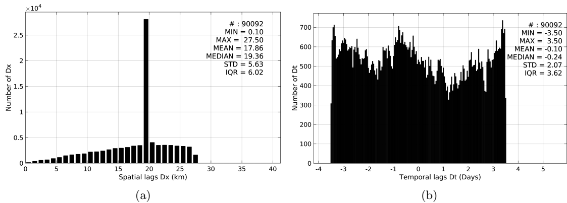
Figure 5: Histograms of the spatial (a) and temporal (b) lags between the time of the TSG-GOSUD-Sailing-ship measurements and the date of the corresponding Aquarius-L4-IPRC-V4-WEEKLY SSS product.
