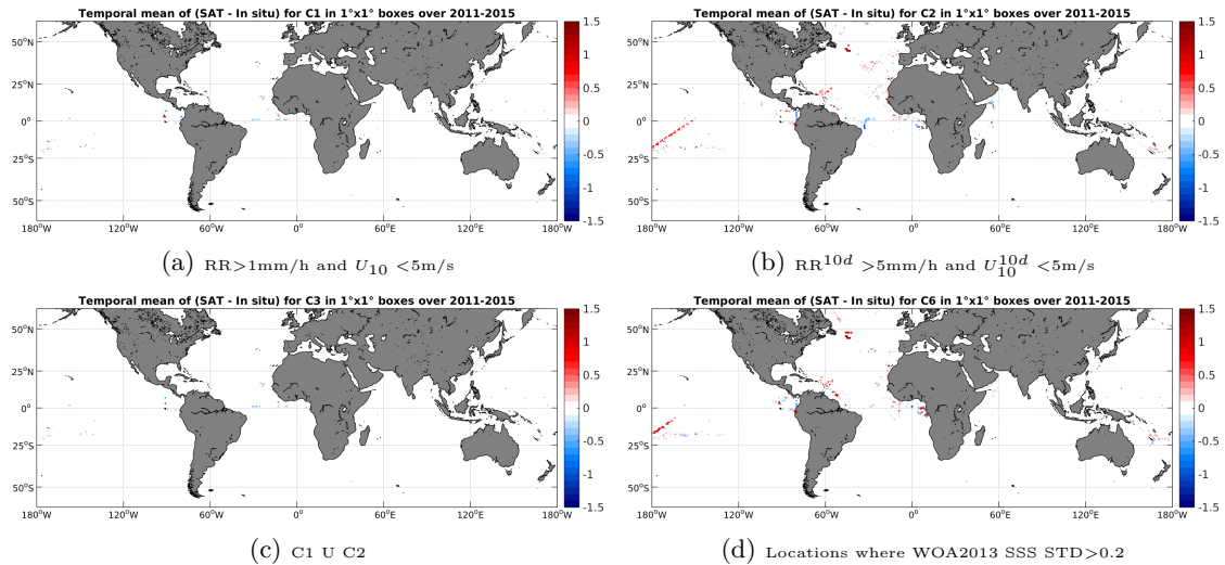
Figure 12: Temporal mean gridded over spatial boxes of size 1^\circ \times 1^\circ of \Delta SSS (Aquarius-L4-IPRC-V4-WEEKLY - TSG-GOSUD-Research-vessel) for 4 different subdatasets corresponding to: RR > 1\text{mm/h} and U_{10} < 5\text{m/s} (a), RR^{10d} > 5\text{mm/h} and U_{10}^{10d} < 5\text{m/s} (b), C1 U C2 (c), Locations where WOA2013 SSS STD > 0.2 (d).
