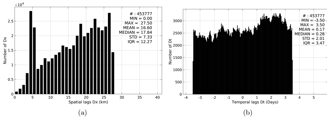
Figure 5: Histograms of the spatial (a) and temporal (b) lags between the time of the TSG-GOSUD-Research-vessel measurements and the date of the corresponding Aquarius-L4-IPRC-V4-WEEKLY SSS product.
