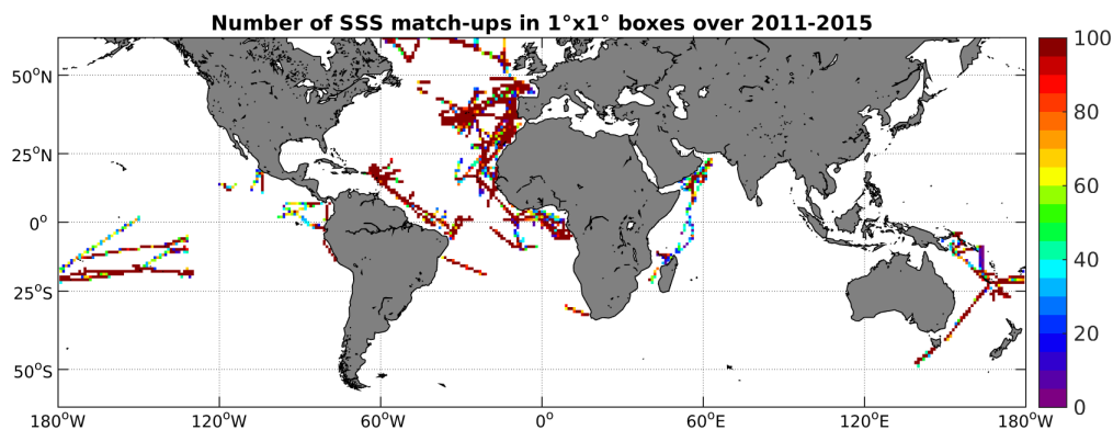
Figure 4: Number of SSS match-ups between TSG-GOSUD-Research-vessel SSS and the Aquarius-L4-IPRC-V4-WEEKLY SSS product for the SMOS coastal zone ( \pm 800\text{km} ) 60N-60S Pi-MEP region over 1^\circ \times 1^\circ boxes and for the full satellite product period.
