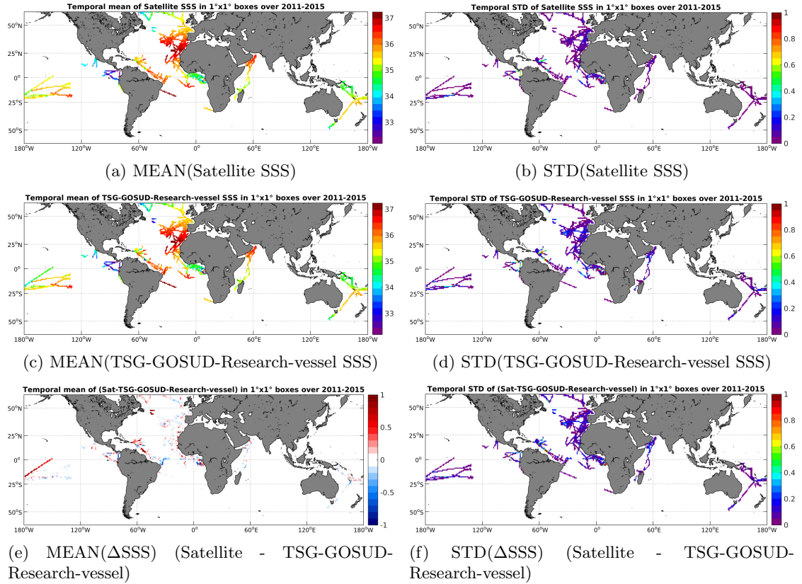
Figure 6: Temporal mean (left) and STD (right) of SSS from Aquarius-L4-IPRC-V4-WEEKLY (top), TSG-GOSUD-Research-vessel (middle), and of \Delta SSS (Satellite - TSG-GOSUD-Research-vessel). Only match-up pairs are used to generate these maps.
