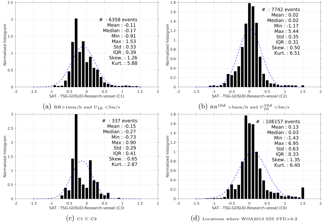
Figure 13: Normalized histogram of \Delta\text{SSS} (Aquarius-L4-IPRC-V4-WEEKLY - TSG-GOSUD-Research-vessel) for 6 different subdatasets corresponding to: \text{RR} > 1\text{mm/h} and U_{10} < 5\text{m/s} (a), \text{RR}^{10d} > 5\text{mm/h} and U_{10}^{10d} < 5\text{m/s} (b), C1 U C2 (c), Locations where WOA2013 SSS STD > 0.2 (d).
