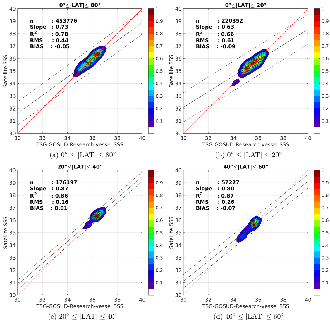
Figure 9: Contour maps of the concentration of Aquarius-L4-IPRC-V4-WEEKLY SSS (y-axis) versus TSG-GOSUD-Research-vessel SSS (x-axis) at match-up pairs for different latitude bands. For each plot, the red line shows x=y . The black thin and dashed lines indicate a linear fit through the data cloud and the \pm 95\% confidence levels, respectively. The number match-up pairs n , the slope and R^2 coefficient of the linear fit, the root mean square (RMS) and the mean bias between satellite and in situ data are indicated for each latitude band in each plots.
