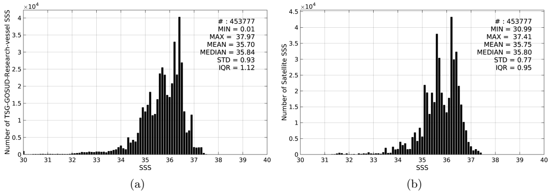
Figure 2: Histograms of SSS from TSG-GOSUD-Research-vessel (a) and Aquarius-L4-IPRC-V4-WEEKLY (b) considering all match-up pairs per bins of 0.1 over the SMOS coastal zone ( \geq 800\text{km} ) 60N-60S Pi-MEP region and for the full satellite product period.
