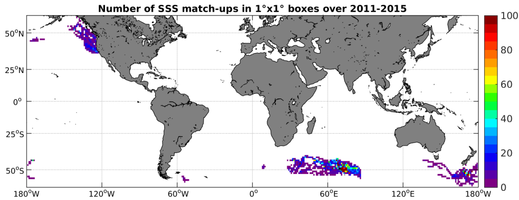
Figure 4: Number of SSS match-ups between Sea mammals SSS and the Aquarius-L4-IPRC-V4-WEEKLY SSS product for the SMOS coastal zone ( \approx 800\text{km} ) 60N-60S Pi-MEP region over 1^\circ \times 1^\circ boxes and for the full satellite product period.
