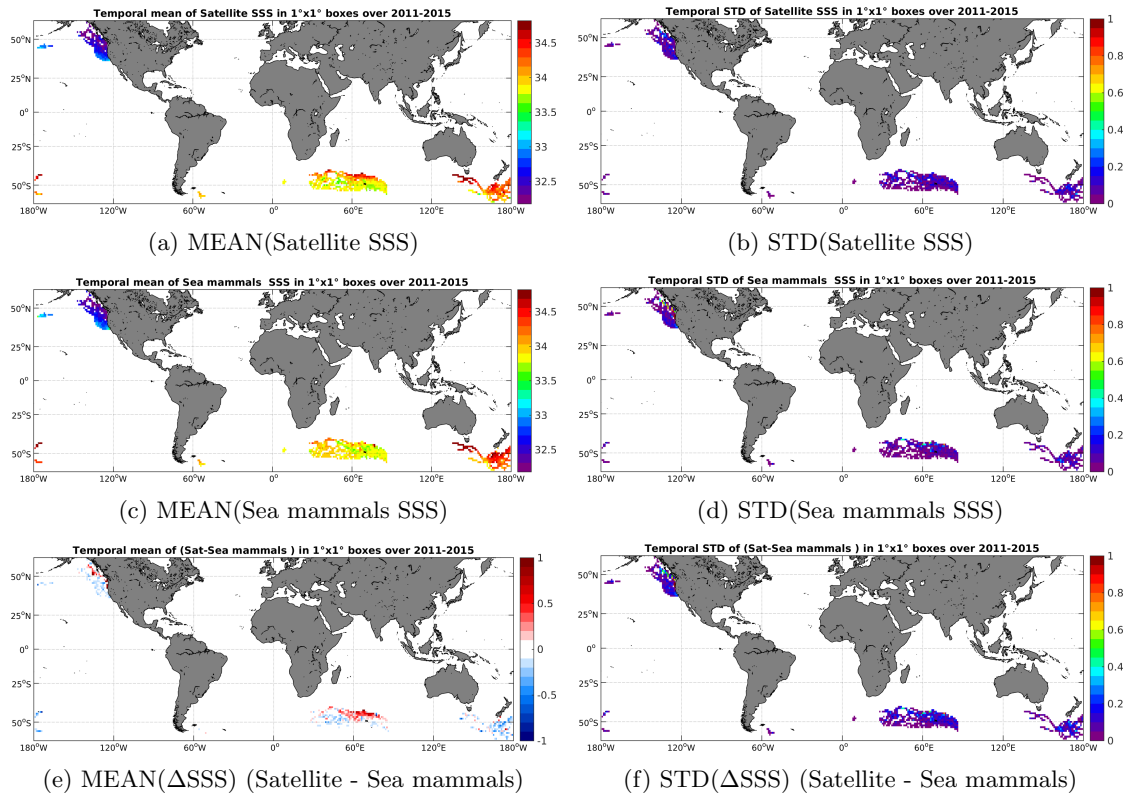
Figure 6: Temporal mean (left) and STD (right) of SSS from Aquarius-L4-IPRC-V4-WEEKLY (top), Sea mammals (middle), and of \Delta SSS (Satellite - Sea mammals). Only match-up pairs are used to generate these maps.
