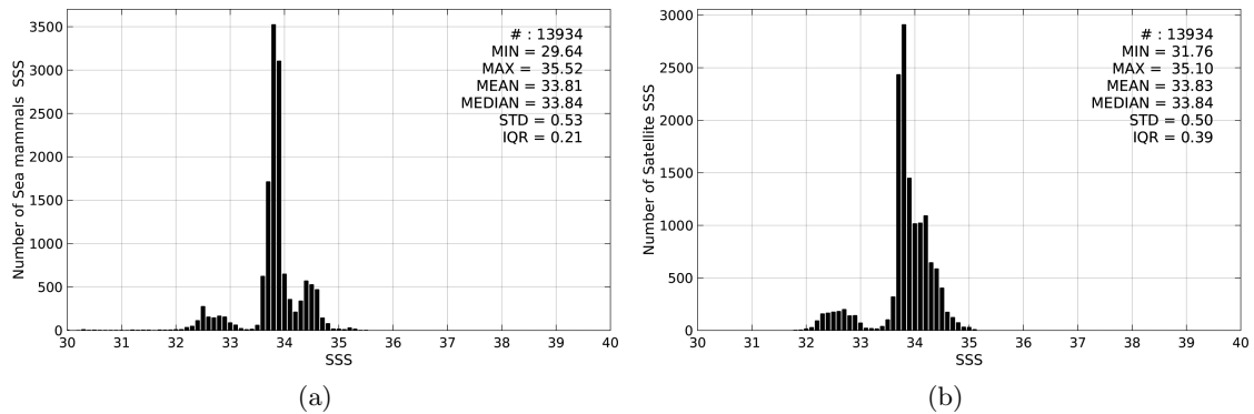
Figure 2: Histograms of SSS from Sea mammals (a) and Aquarius-L4-IPRC-V4-WEEKLY (b) considering all match-up pairs per bins of 0.1 over the SMOS coastal zone ( \pm 800\text{km} ) 60N-60S Pi-MEP region and for the full satellite product period.
