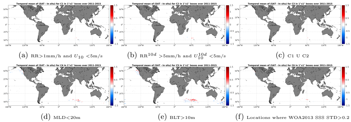
Figure 12: Temporal mean gridded over spatial boxes of size 1^\circ \times 1^\circ of \Delta SSS (Aquarius-L4-IPRC-V4-WEEKLY - Sea mammals) for 6 different subdatasets corresponding to:RR>1mm/h and U_{10} < 5\text{m/s} (a), RR^{10d} > 5\text{mm/h} and U_{10}^{10d} < 5\text{m/s} (b), C1 U C2 (c),MLD<20m (d),BLT>10m (e),Locations where WOA2013 SSS STD>0.2 (f).
