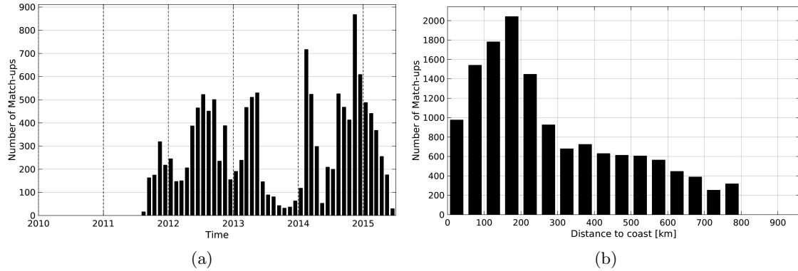
Figure 1: Number of match-ups between Sea mammals and Aquarius-L4-IPRC-V4-WEEKLY SSS as a function of time (a) and as function of the distance to coast (b) over the SMOS coastal zone ( \pm 800\text{km} ) 60N-60S Pi-MEP region and for the full satellite product period.
