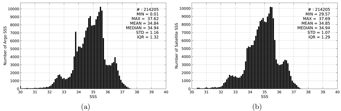
Figure 2: Histograms of SSS from Argo (a) and Aquarius-L4-IPRC-V4-WEEKLY (b) considering all match-up pairs per bins of 0.1 over the SMOS coastal zone ( \pm 800\text{km} ) 60N-60S Pi-MEP region and for the full satellite product period.
