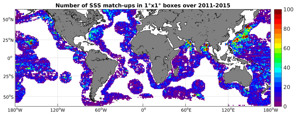
Figure 4: Number of SSS match-ups between Argo SSS and the Aquarius-L4-IPRC-V4-WEEKLY SSS product for the SMOS coastal zone ( \approx 800\text{km} ) 60N-60S Pi-MEP region over 1^\circ \times 1^\circ boxes and for the full satellite product period.
