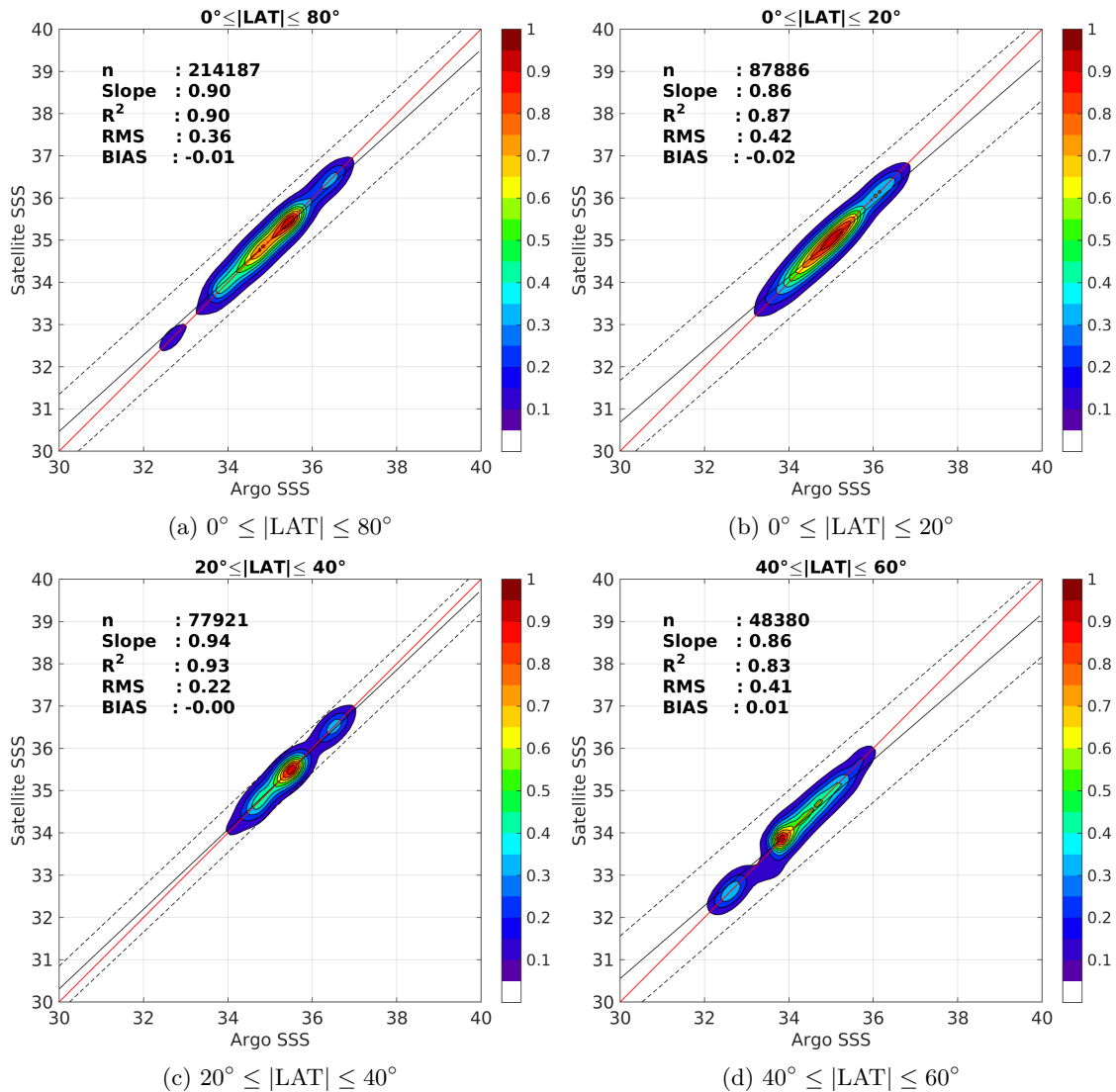
Figure 9: Contour maps of the concentration of Aquarius-L4-IPRC-V4-WEEKLY SSS (y-axis) versus Argo SSS (x-axis) at match-up pairs for different latitude bands. For each plot, the red line shows x=y . The black thin and dashed lines indicate a linear fit through the data cloud and the \pm 95\% confidence levels, respectively. The number match-up pairs n , the slope and R 2 coefficient of the linear fit, the root mean square (RMS) and the mean bias between satellite and in situ data are indicated for each latitude band in each plots.
