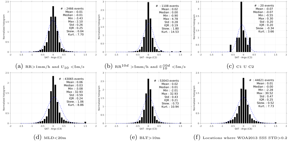
Figure 13: Normalized histogram of \Delta SSS (Aquarius-L4-IPRC-V4-WEEKLY - Argo) for 6 different subdatasets corresponding to: RR>1mm/h and U_{10} <5m/s (a), RR 10d >5mm/h and U_{10}^{10d} <5m/s (b), C1 U C2 (c),MLD<20m (d),BLT>10m (e),Locations where WOA2013 SSS STD>0.2 (f).
