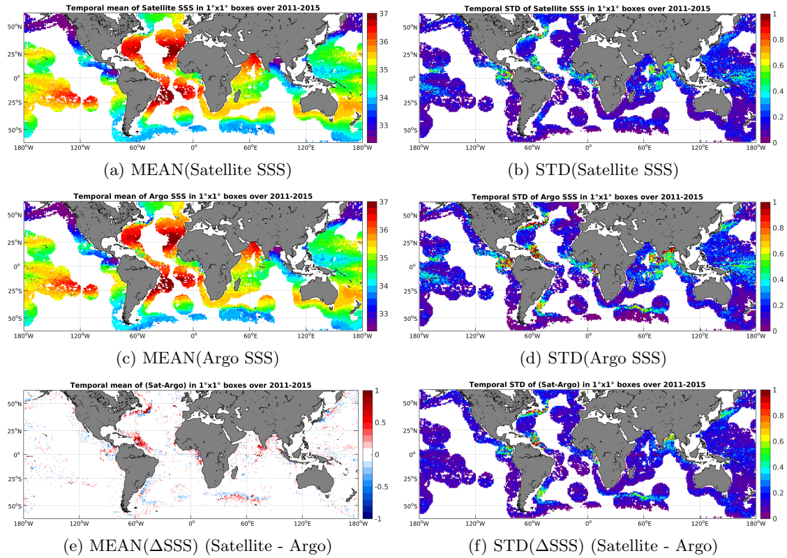
Figure 6: Temporal mean (left) and STD (right) of SSS from Aquarius-L4-IPRC-V4-WEEKLY (top), Argo (middle), and of \Delta SSS (Satellite - Argo). Only match-up pairs are used to generate these maps.
