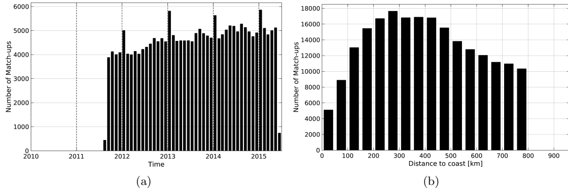
Figure 1: Number of match-ups between Argo and Aquarius-L4-IPRC-V4-WEEKLY SSS as a function of time (a) and as function of the distance to coast (b) over the SMOS coastal zone ( \pm 800\text{km} ) 60N-60S Pi-MEP region and for the full satellite product period.
