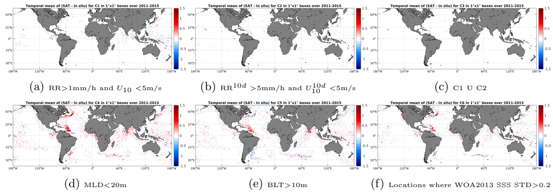
Figure 12: Temporal mean gridded over spatial boxes of size 1^\circ \times 1^\circ of \Delta SSS (Aquarius-L4-IPRC-V4-WEEKLY - Argo) for 6 different subdatasets corresponding to: RR > 1\text{mm/h} and U_{10} < 5\text{m/s} (a), RR^{10d} > 5\text{mm/h} and U_{10}^{10d} < 5\text{m/s} (b), C1 U C2 (c), MLD < 20\text{m} (d), BLT > 10\text{m} (e), Locations where WOA2013 SSS STD > 0.2 (f).
