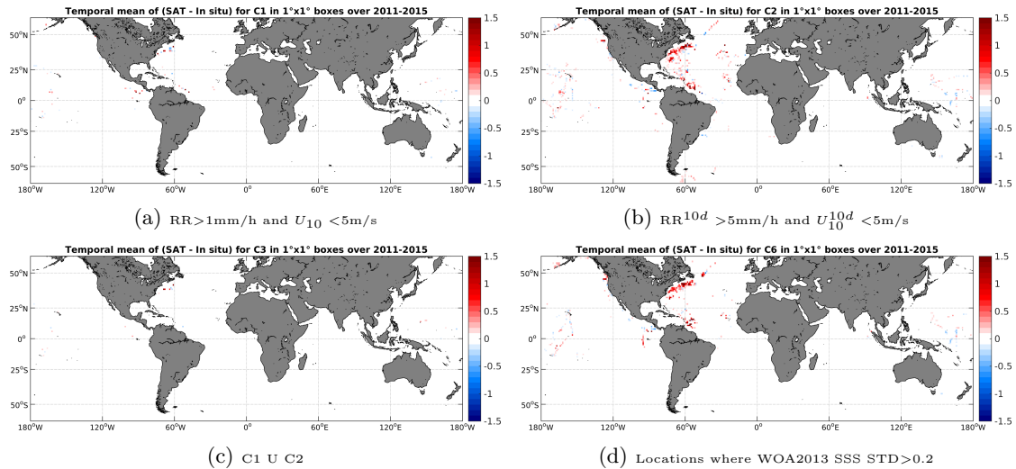
Figure 12: Temporal mean gridded over spatial boxes of size 1^\circ \times 1^\circ of \Delta SSS (Aquarius-L4-IPRC-V4-MONTHLY - TSG-SAMOS) for 4 different subdatasets corresponding to:RR >1 mm/h and U_{10} < 5 m/s (a), RR 10d > 5 mm/h and U_{10}^{10d} < 5 m/s (b), C1 U C2 (c),Locations where WOA2013 SSS STD >0.2 (d).
