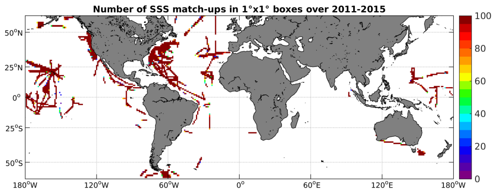
Figure 4: Number of SSS match-ups between TSG-SAMOS SSS and the Aquarius-L4-IPRC-V4-MONTHLY SSS product for the SMOS coastal zone ( \approx 800\text{km} ) 60N-60S Pi-MEP region over 1^\circ \times 1^\circ boxes and for the full satellite product period.
