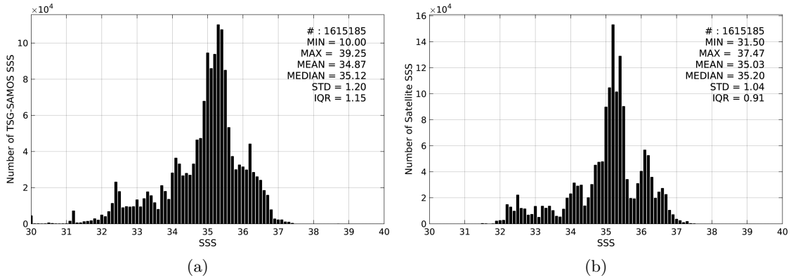
Figure 2: Histograms of SSS from TSG-SAMOS (a) and Aquarius-L4-IPRC-V4-MONTHLY (b) considering all match-up pairs per bins of 0.1 over the SMOS coastal zone ( \geq 800 km) 60N-60S Pi-MEP region and for the full satellite product period.
