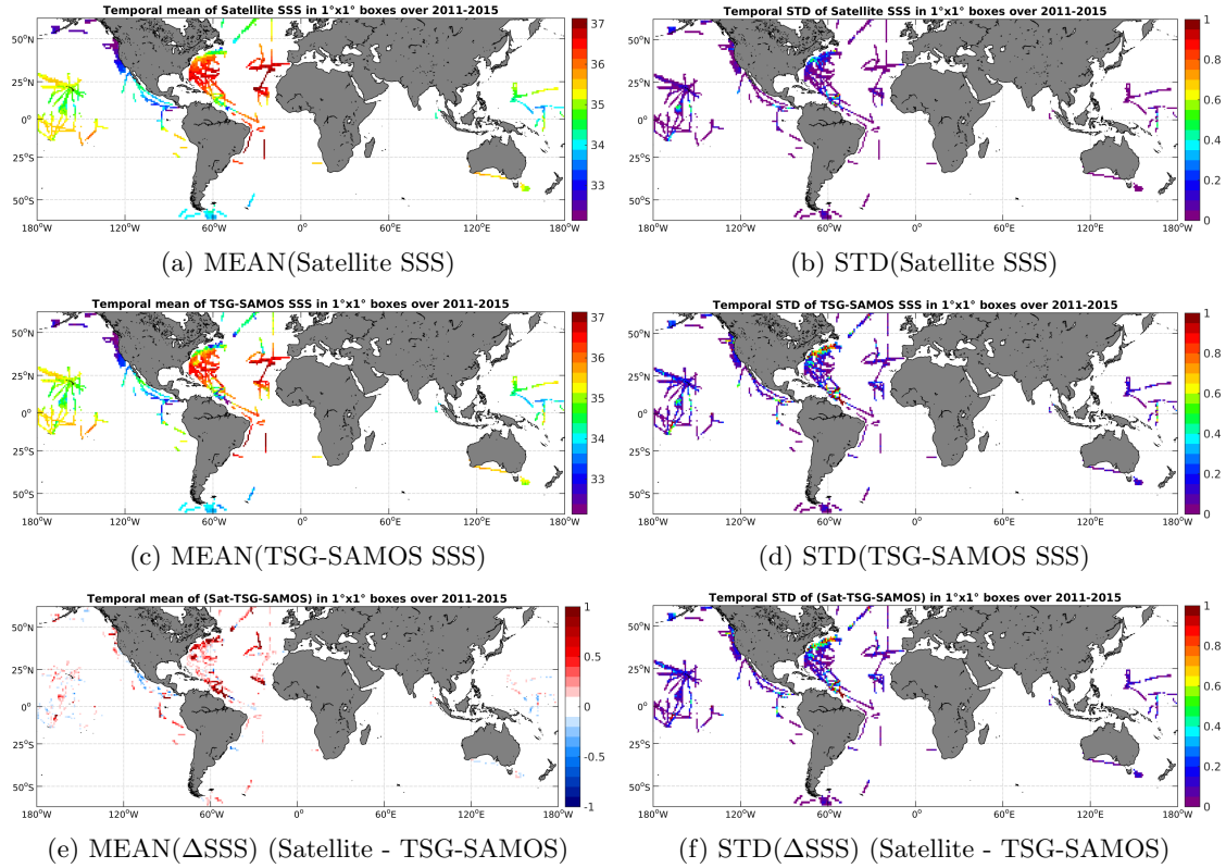
Figure 6: Temporal mean (left) and STD (right) of SSS from Aquarius-L4-IPRC-V4-MONTHLY (top), TSG-SAMOS (middle), and of \Delta SSS (Satellite - TSG-SAMOS). Only match-up pairs are used to generate these maps.
