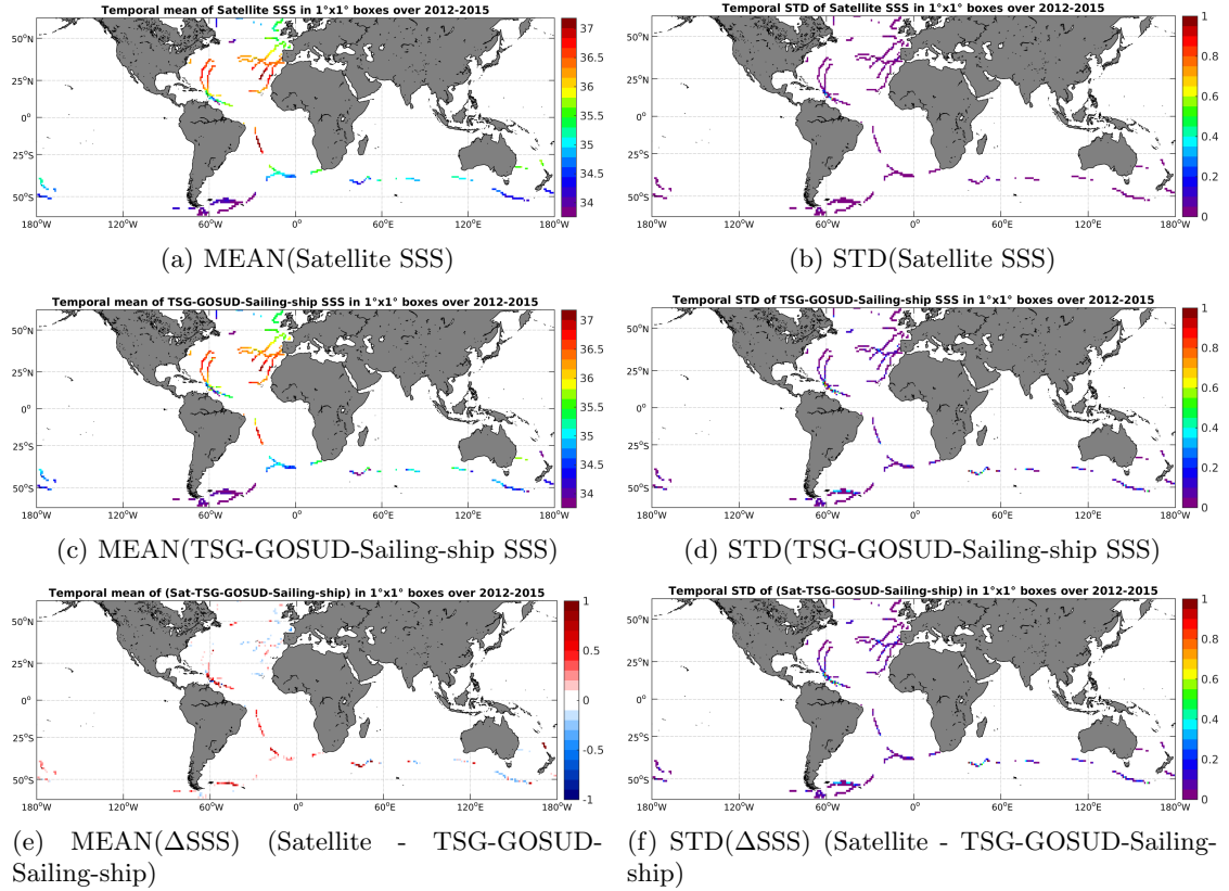
Figure 6: Temporal mean (left) and STD (right) of SSS from Aquarius-L4-IPRC-V4-MONTHLY (top), TSG-GOSUD-Sailing-ship (middle), and of \Delta SSS (Satellite - TSG-GOSUD-Sailing-ship). Only match-up pairs are used to generate these maps.
