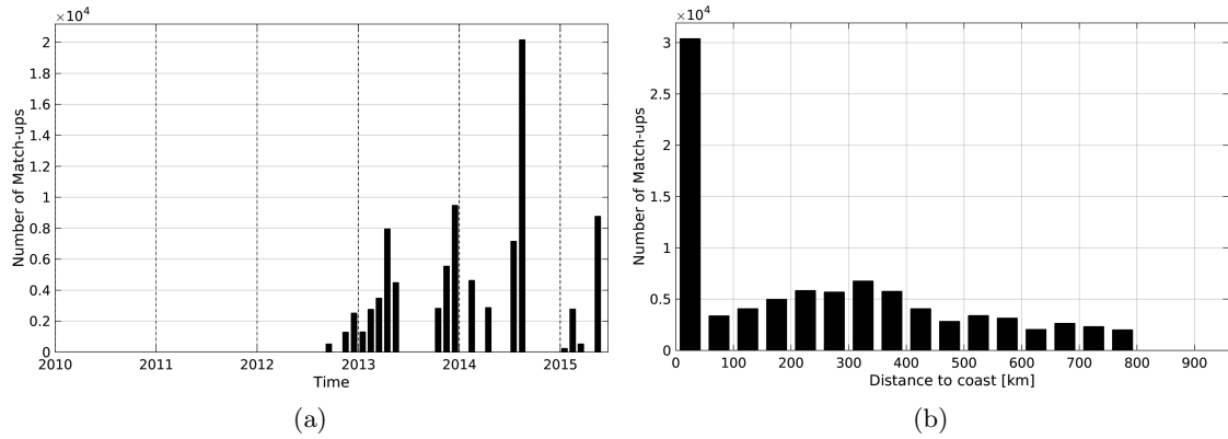
Figure 1: Number of match-ups between TSG-GOSUD-Sailing-ship and Aquarius-L4-IPRC-V4-MONTHLY SSS as a function of time (a) and as function of the distance to coast (b) over the SMOS coastal zone ( \leq 800 km) 60N-60S Pi-MEP region and for the full satellite product period.
