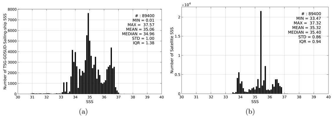
Figure 2: Histograms of SSS from TSG-GOSUD-Sailing-ship (a) and Aquarius-L4-IPRC-V4-MONTHLY (b) considering all match-up pairs per bins of 0.1 over the SMOS coastal zone ( \leq 800 km) 60N-60S Pi-MEP region and for the full satellite product period.
