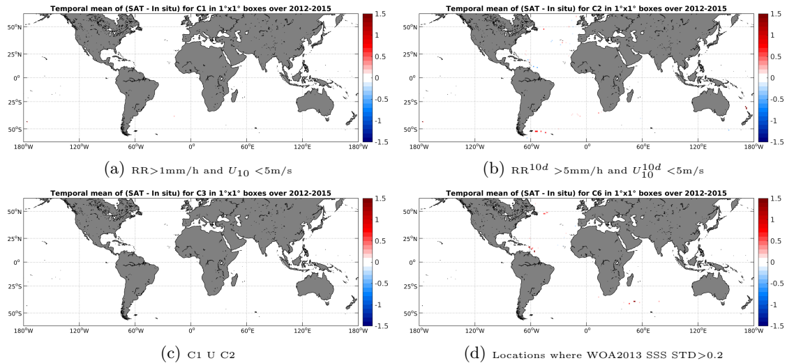
Figure 12: Temporal mean gridded over spatial boxes of size 1^\circ \times 1^\circ of \Delta SSS (Aquarius-L4-IPRC-V4-MONTHLY - TSG-GOSUD-Sailing-ship) for 4 different subdatasets corresponding to: RR > 1\text{mm/h} and U_{10} < 5\text{m/s} (a), RR^{10d} > 5\text{mm/h} and U_{10}^{10d} < 5\text{m/s} (b), C1 U C2 (c), Locations where WOA2013 SSS STD > 0.2 (d).
