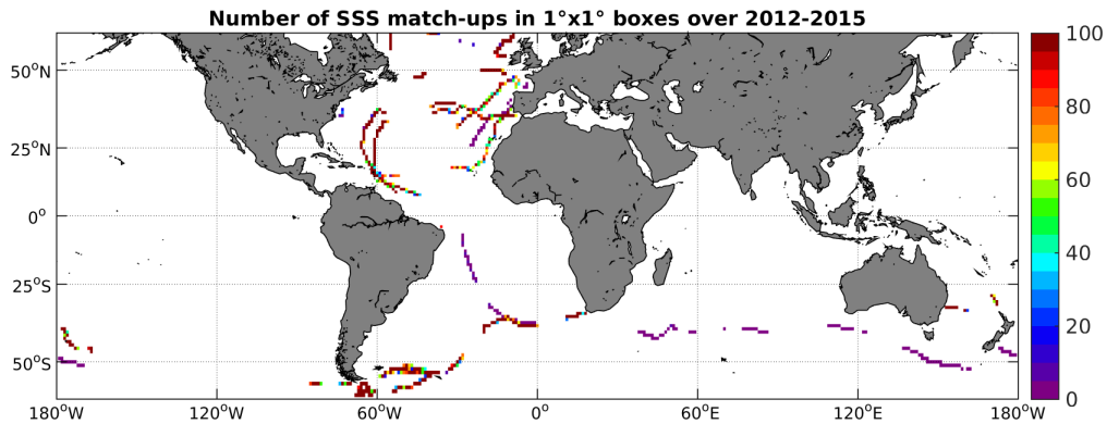
Figure 4: Number of SSS match-ups between TSG-GOSUD-Sailing-ship SSS and the Aquarius-L4-IPRC-V4-MONTHLY SSS product for the SMOS coastal zone ( \pm 800\text{km} ) 60N-60S Pi-MEP region over 1^\circ \times 1^\circ boxes and for the full satellite product period.
