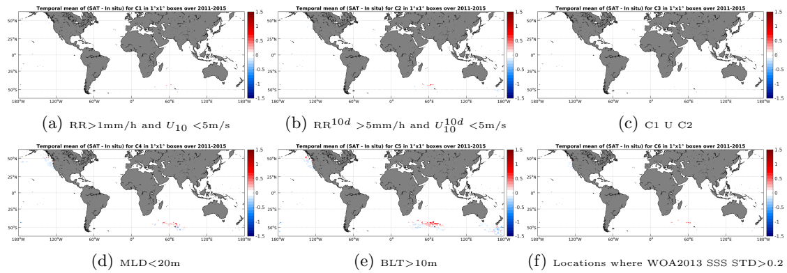
Figure 12: Temporal mean gridded over spatial boxes of size 1^\circ \times 1^\circ of \Delta SSS (Aquarius-L4-IPRC-V4-MONTHLY - Sea mammals) for 6 different subdatasets corresponding to:RR>1mm/h and U_{10} < 5\text{m/s} (a), RR^{10d} > 5\text{mm/h} and U_{10}^{10d} < 5\text{m/s} (b), C1 U C2 (c),MLD<20m (d),BLT>10m (e),Locations where WOA2013 SSS STD>0.2 (f).
