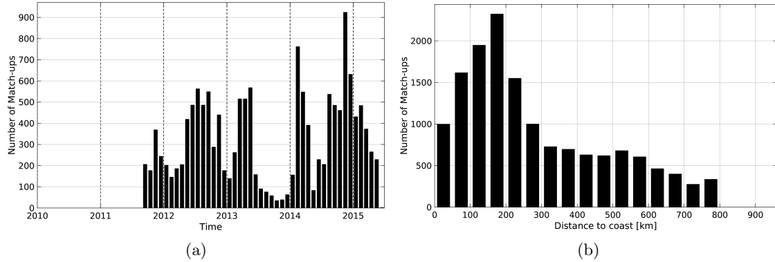
Figure 1: Number of match-ups between Sea mammals and Aquarius-L4-IPRC-V4-MONTHLY SSS as a function of time (a) and as function of the distance to coast (b) over the SMOS coastal zone ( \pm 800\text{km} ) 60N-60S Pi-MEP region and for the full satellite product period.
