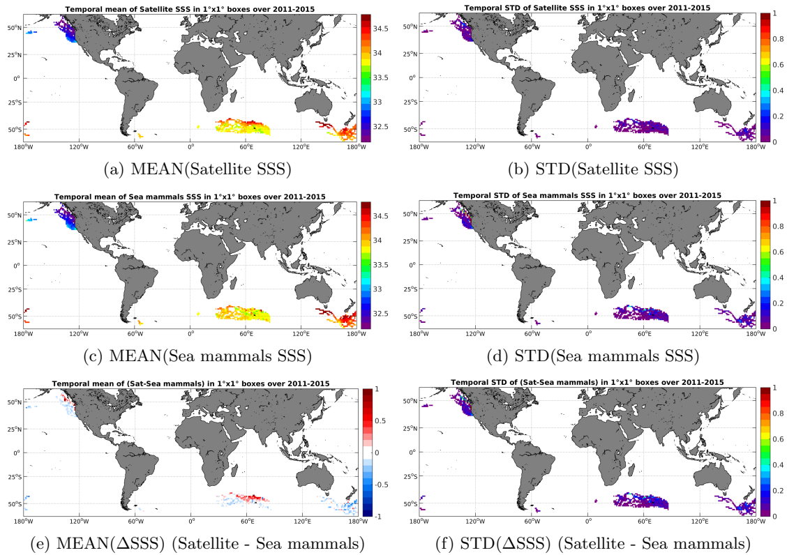
Figure 6: Temporal mean (left) and STD (right) of SSS from Aquarius-L4-IPRC-V4-MONTHLY (top), Sea mammals (middle), and of \Delta SSS (Satellite - Sea mammals). Only match-up pairs are used to generate these maps.
