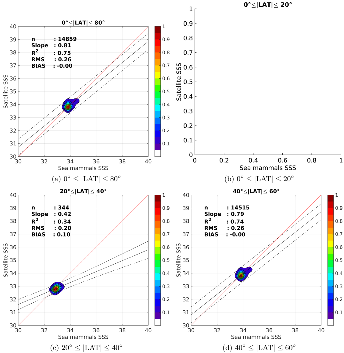
Figure 9: Contour maps of the concentration of Aquarius-L4-IPRC-V4-MONTHLY SSS (y-axis) versus Sea mammals SSS (x-axis) at match-up pairs for different latitude bands. For each plot, the red line shows x=y . The black thin and dashed lines indicate a linear fit through the data cloud and the \pm 95\% confidence levels, respectively. The number match-up pairs n , the slope and R^2 coefficient of the linear fit, the root mean square (RMS) and the mean bias between satellite and in situ data are indicated for each latitude band in each plots.
