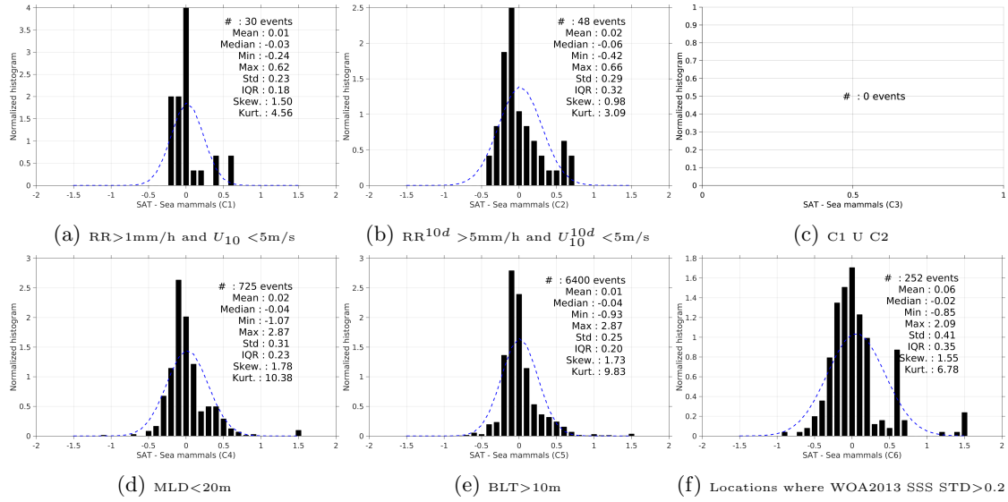
Figure 13: Normalized histogram of \Delta SSS (Aquarius-L4-IPRC-V4-MONTHLY - Sea mammals) for 6 different subdatasets corresponding to: RR > 1mm/h and U_{10} < 5 m/s (a), RR 10d > 5mm/h and U_{10}^{10d} < 5 m/s (b), C1 U C2 (c), MLD < 20m (d), BLT > 10m (e), Locations where WOA2013 SSS STD > 0.2 (f).
