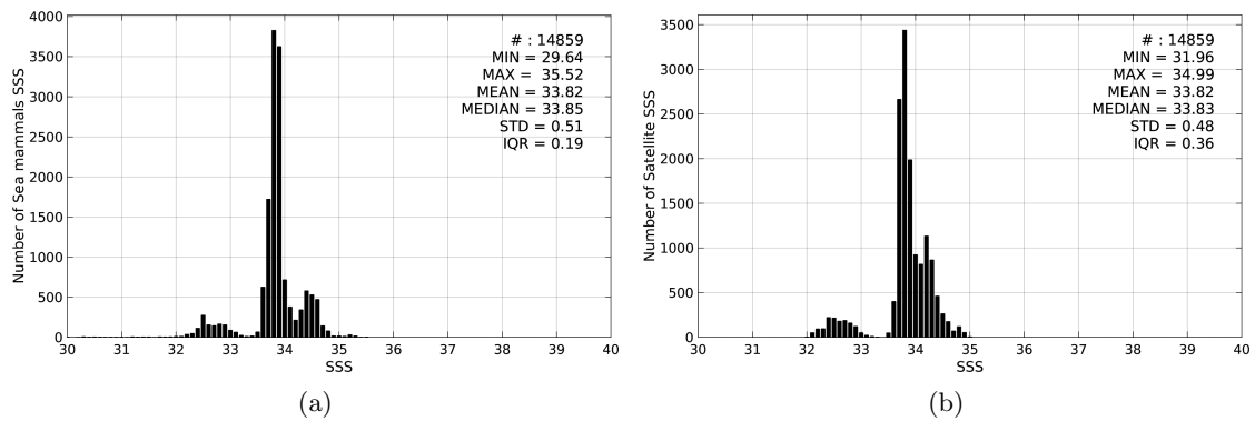
Figure 2: Histograms of SSS from Sea mammals (a) and Aquarius-L4-IPRC-V4-MONTHLY (b) considering all match-up pairs per bins of 0.1 over the SMOS coastal zone ( \pm 800\text{km} ) 60N-60S Pi-MEP region and for the full satellite product period.
