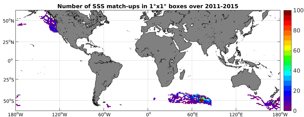
Figure 4: Number of SSS match-ups between Sea mammals SSS and the Aquarius-L4-IPRC-V4-MONTHLY SSS product for the SMOS coastal zone ( \pm 800\text{km} ) 60N-60S Pi-MEP region over 1^\circ \times 1^\circ boxes and for the full satellite product period.
