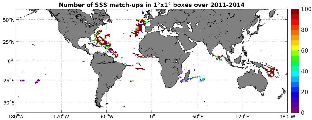
Figure 3: Number of SSS match-ups between Surface drifters SSS and the Aquarius-L4-IPRC-V4-MONTHLY SSS product for the SMOS coastal zone ( \approx 800\text{km} ) 60N-60S Pi-MEP region over 1^\circ \times 1^\circ boxes and for the full satellite product period.
