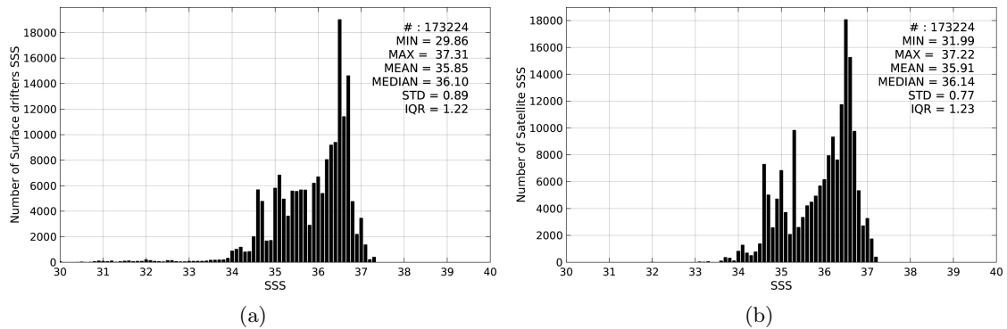
Figure 2: Histograms of SSS from Surface drifters (a) and Aquarius-L4-IPRC-V4-MONTHLY (b) considering all match-up pairs per bins of 0.1 over the SMOS coastal zone ( \approx 800 km) 60N-60S Pi-MEP region and for the full satellite product period.
