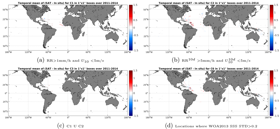
Figure 11: Temporal mean gridded over spatial boxes of size 1^\circ \times 1^\circ of \Delta SSS (Aquarius-L4-IPRC-V4-MONTHLY - Surface drifters) for 4 different subdatasets corresponding to: RR > 1\text{mm/h} and U_{10} < 5\text{m/s} (a), RR^{10d} > 5\text{mm/h} and U_{10}^{10d} < 5\text{m/s} (b), C1 U C2 (c), Locations where WOA2013 SSS STD > 0.2 (d).
