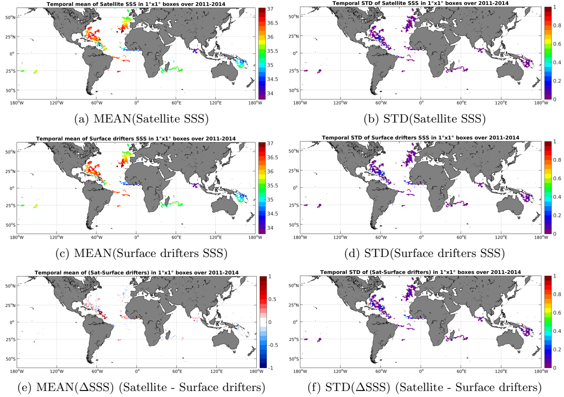
Figure 5: Temporal mean (left) and STD (right) of SSS from Aquarius-L4-IPRC-V4-MONTHLY (top), Surface drifters (middle), and of \Delta SSS (Satellite - Surface drifters). Only match-up pairs are used to generate these maps.
