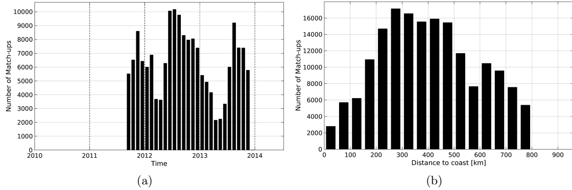
Figure 1: Number of match-ups between Surface drifters and Aquarius-L4-IPRC-V4-MONTHLY SSS as a function of time (a) and as function of the distance to coast (b) over the SMOS coastal zone ( \approx 800 km) 60N-60S Pi-MEP region and for the full satellite product period.
