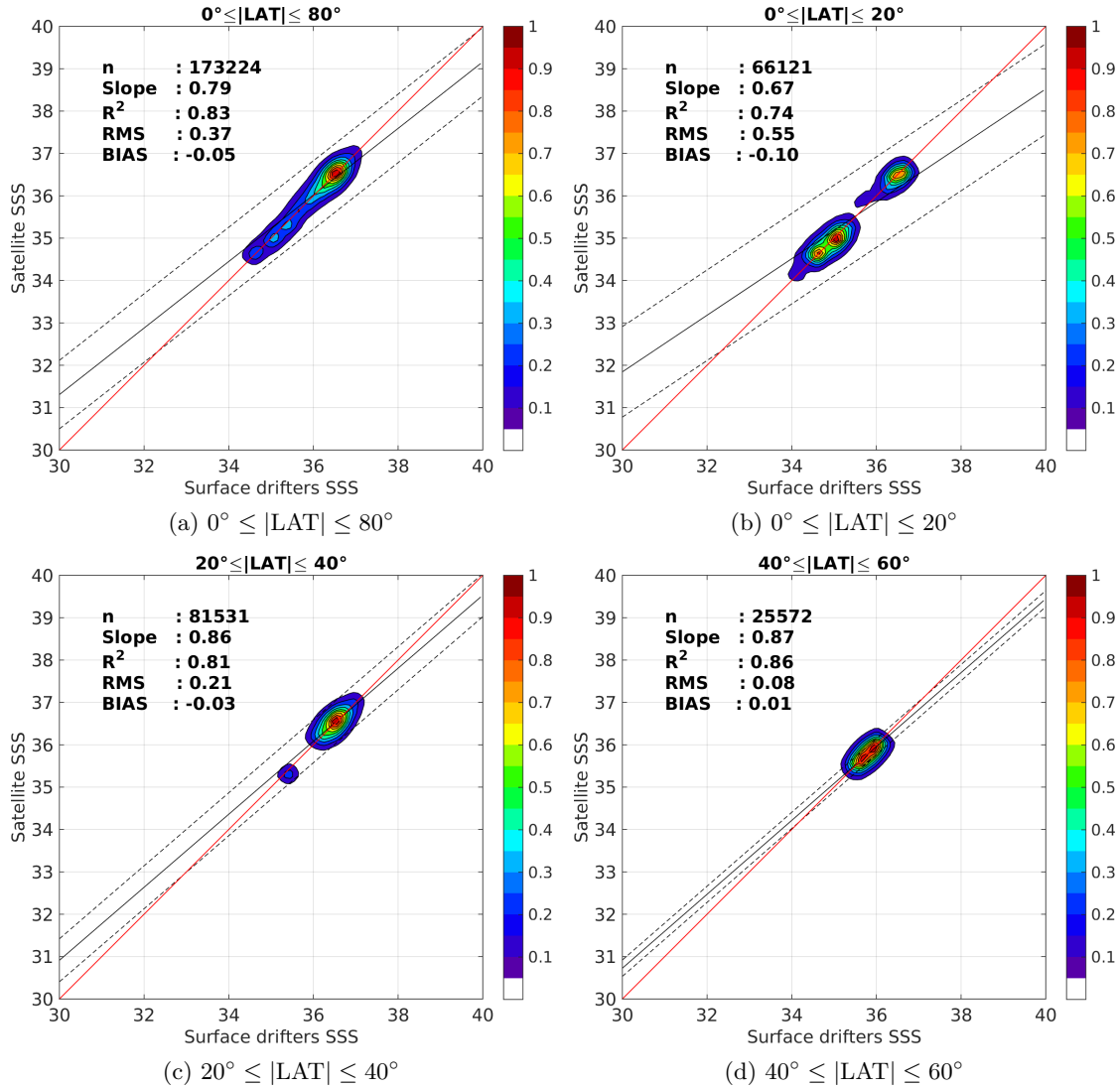
Figure 8: Contour maps of the concentration of Aquarius-L4-IPRC-V4-MONTHLY SSS (y-axis) versus Surface drifters SSS (x-axis) at match-up pairs for different latitude bands. For each plot, the red line shows x=y . The black thin and dashed lines indicate a linear fit through the data cloud and the \pm 95\% confidence levels, respectively. The number match-up pairs n , the slope and R^2 coefficient of the linear fit, the root mean square (RMS) and the mean bias between satellite and in situ data are indicated for each latitude band in each plots.
