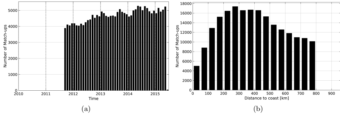
Figure 1: Number of match-ups between Argo and Aquarius-L4-IPRC-V4-MONTHLY SSS as a function of time (a) and as function of the distance to coast (b) over the SMOS coastal zone ( \pm 800\text{km} ) 60N-60S Pi-MEP region and for the full satellite product period.
