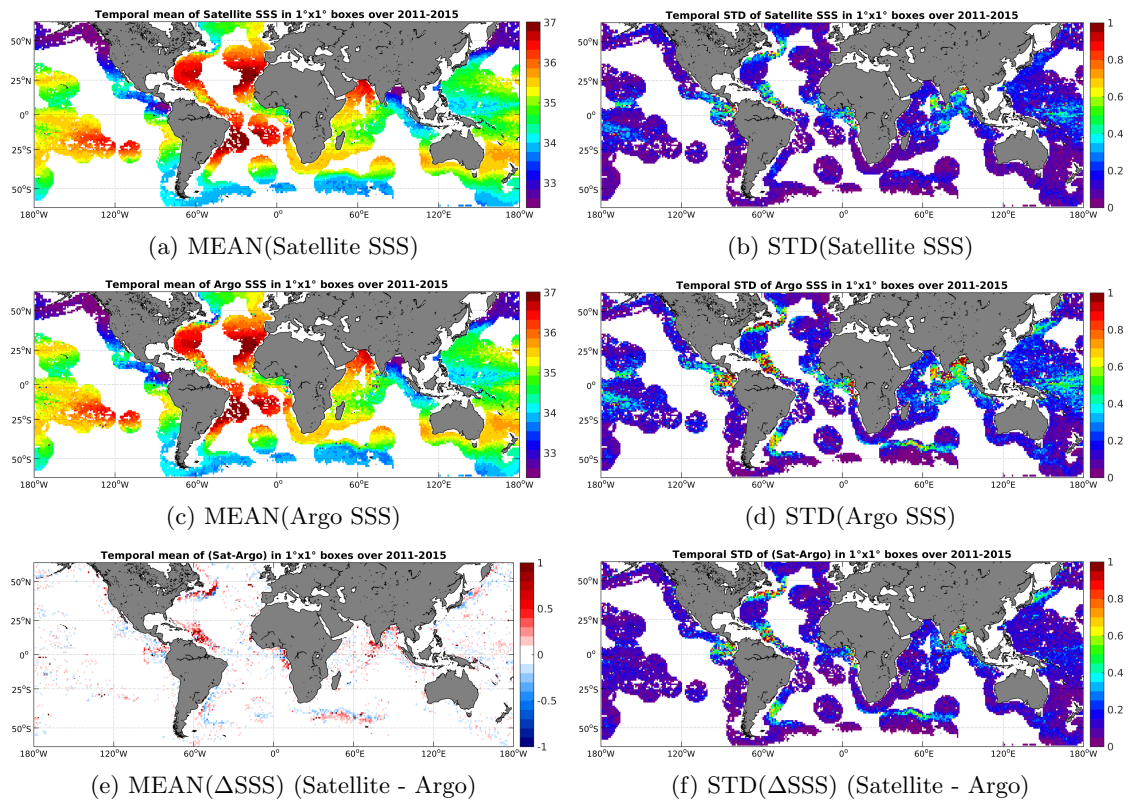
Figure 6: Temporal mean (left) and STD (right) of SSS from Aquarius-L4-IPRC-V4-MONTHLY (top), Argo (middle), and of \Delta SSS (Satellite - Argo). Only match-up pairs are used to generate these maps.
