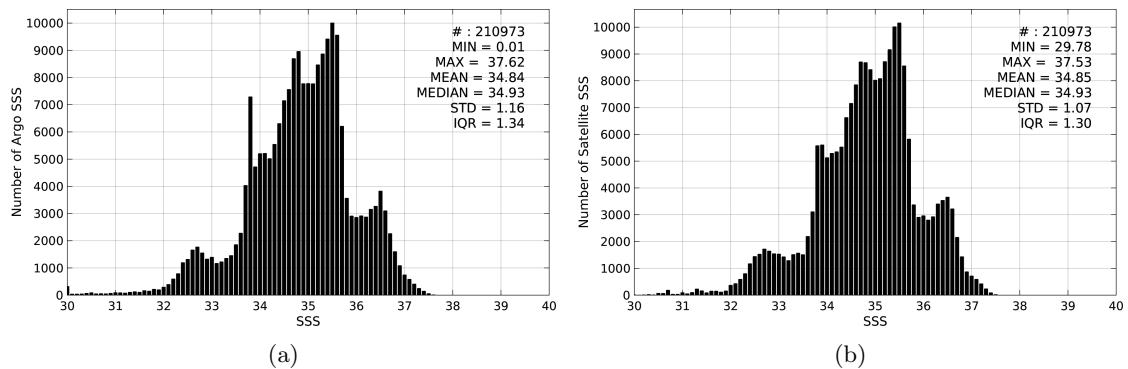
Figure 2: Histograms of SSS from Argo (a) and Aquarius-L4-IPRC-V4-MONTHLY (b) considering all match-up pairs per bins of 0.1 over the SMOS coastal zone ( \pm 800\text{km} ) 60N-60S Pi-MEP region and for the full satellite product period.
