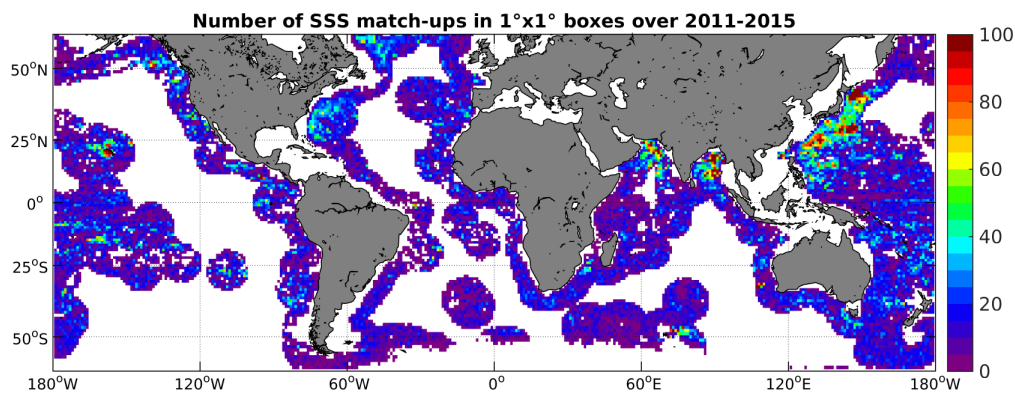
Figure 4: Number of SSS match-ups between Argo SSS and the Aquarius-L4-IPRC-V4-MONTHLY SSS product for the SMOS coastal zone ( \approx 800\text{km} ) 60N-60S Pi-MEP region over 1^\circ \times 1^\circ boxes and for the full satellite product period.
