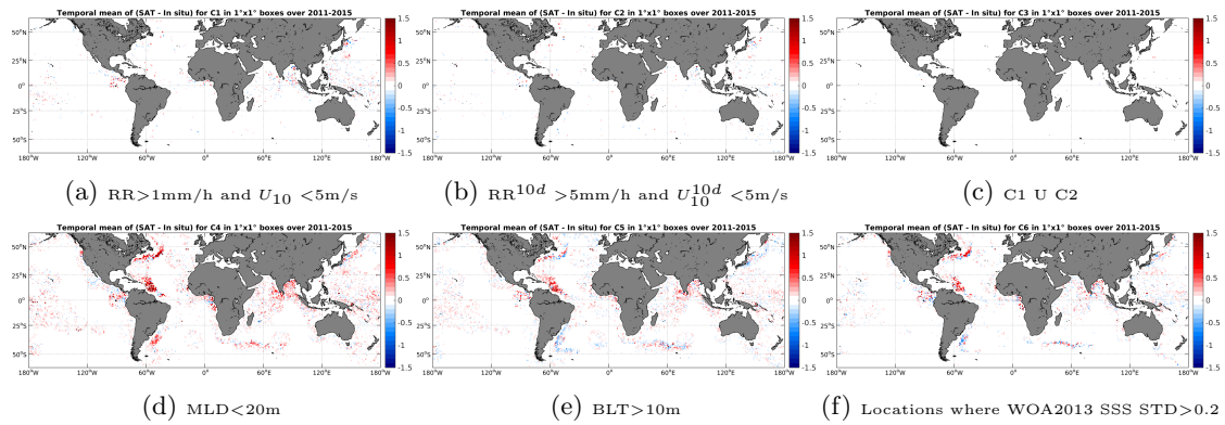
Figure 12: Temporal mean gridded over spatial boxes of size 1^\circ \times 1^\circ of \Delta SSS (Aquarius-L4-IPRC-V4-MONTHLY - Argo) for 6 different subdatasets corresponding to: RR > 1\text{mm/h} and U_{10} < 5\text{m/s} (a), RR^{10d} > 5\text{mm/h} and U_{10}^{10d} < 5\text{m/s} (b), C1 \cup C2 (c), MLD < 20\text{m} (d), BLT > 10\text{m} (e), Locations where WOA2013 SSS STD > 0.2 (f).
