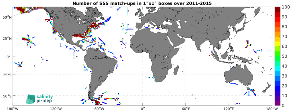
Figure 5: Number of SSS match-ups between TSG (SAMOS) SSS and the Aquarius SSS L3 OR v5 - 7-Day running (NASA-GSFC) SSS product for the SMOS coastal zone (<800km) 60N-60S Pi-MEP region over 1^\circ \times 1^\circ boxes and for the full satellite product period.
