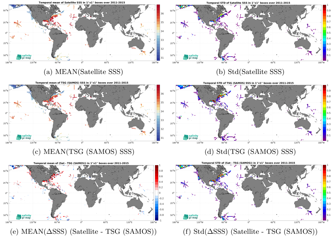
Figure 7: Temporal mean (left) and Std (right) of SSS from Aquarius SSS L3 OR v5 - 7-Day running (NASA-GSFC) (top), TSG (SAMOS) (middle), and of \Delta SSS (Satellite - TSG (SAMOS)). Only match-up pairs are used to generate these maps.
