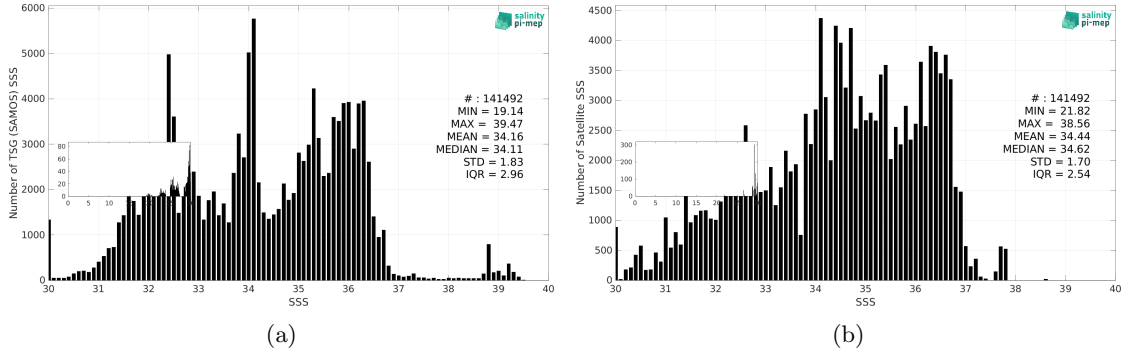
Figure 3: Histograms of SSS from TSG (SAMOS) (a) and Aquarius SSS L3 OR v5 - 7-Day running (NASA-GSFC) (b) considering all match-up pairs per bins of 0.1 over the SMOS coastal zone (<800km) 60N-60S Pi-MEP region and for the full satellite product period.
