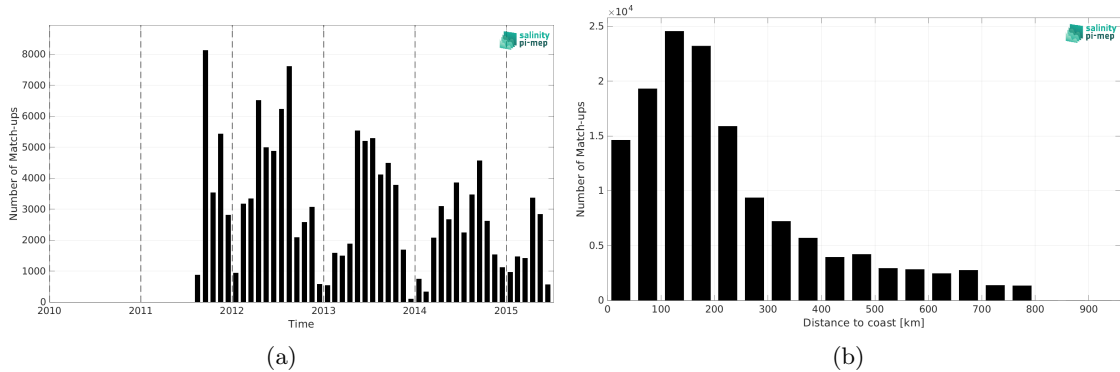
Figure 2: Number of match-ups between TSG (SAMOS) and Aquarius SSS L3 OR v5 - 7-Day running (NASA-GSFC) SSS as a function of time (a) and as function of the distance to coast (b) over the SMOS coastal zone (<800km) 60N-60S Pi-MEP region and for the full satellite product period.
