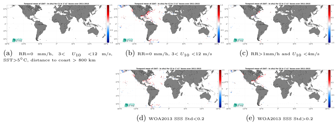
Figure 14: Temporal mean gridded over spatial boxes of size 1^\circ \times 1^\circ of \Delta\text{SSS} (Aquarius SSS L3 OR v5 - 7-Day running (NASA-GSFC) - TSG (SAMOS)) for 5 different subdatasets corresponding to:RR=0 mm/h, 3 < U_{10} < 12 m/s, SST>5°C, distance to coast > 800 km (a), RR=0 mm/h, 3 < U_{10} < 12 m/s (b), RR>1mm/h and U_{10} < 4 m/s (c), WOA2013 SSS Std<0.2 (d), WOA2013 SSS Std>0.2 (e).
