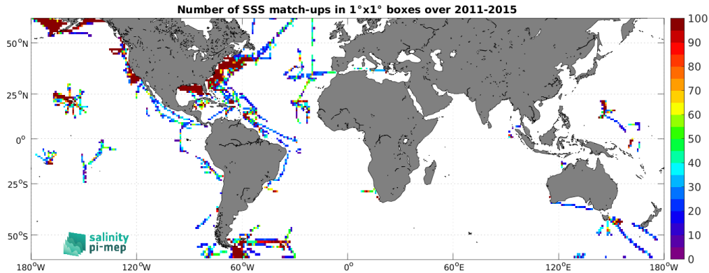
Figure 4: Number of SSS match-ups between TSG (SAMOS) SSS and the Aquarius SSS L3 OR v5 - 7-Day running (NASA-GSFC) SSS product for the SMOS coastal zone (<800km) 60N-60S Pi-MEP region over 1^{\circ} \times 1^{\circ} boxes and for the full satellite product period.
