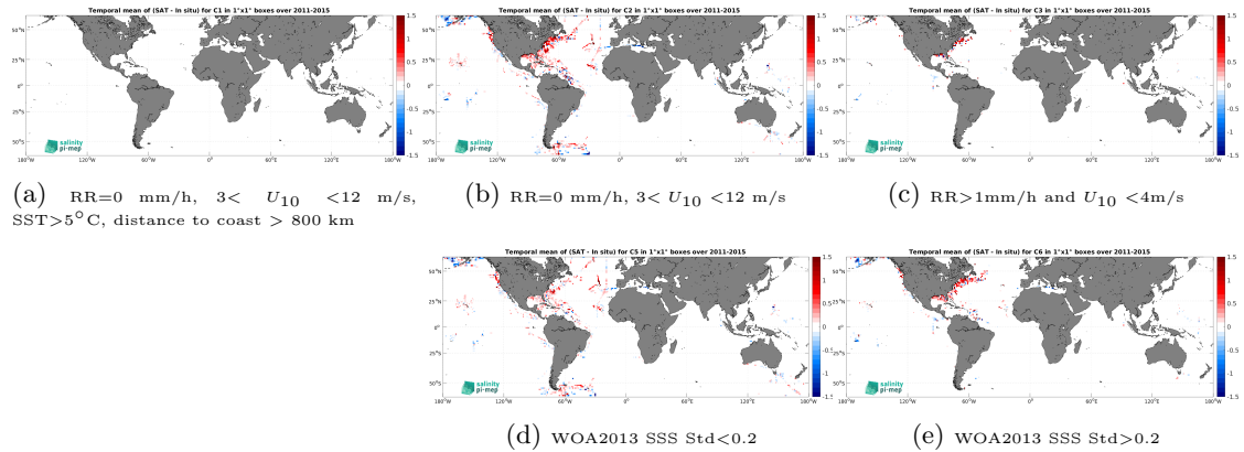
Figure 12: Temporal mean gridded over spatial boxes of size 1^\circ \times 1^\circ of \Delta SSS (Aquarius SSS L3 OR v5 - 7-Day running (NASA-GSFC) - TSG (SAMOS)) for 5 different subdatasets corresponding to:RR=0 mm/h, 3 < U_{10} < 12 m/s, SST >5^\circ\text{C} , distance to coast > 800 km (a), RR=0 mm/h, 3 < U_{10} < 12 m/s (b), RR >1 mm/h and U_{10} < 4 m/s (c), WOA2013 SSS Std <0.2 (d), WOA2013 SSS Std >0.2 (e).
