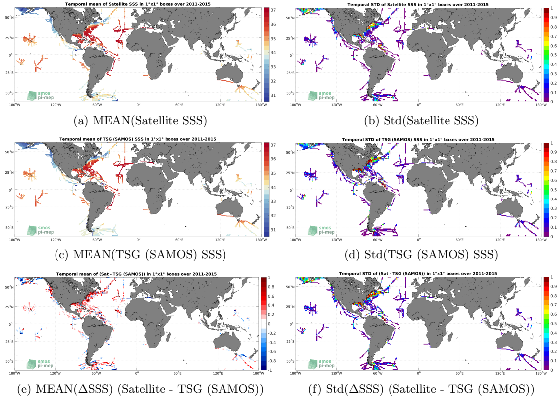
Figure 6: Temporal mean (left) and Std (right) of SSS from Aquarius SSS L3 OR v5 - 7-Day running (NASA-GSFC) (top), TSG (SAMOS) (middle), and of \Delta SSS (Satellite - TSG (SAMOS)). Only match-up pairs are used to generate these maps.
