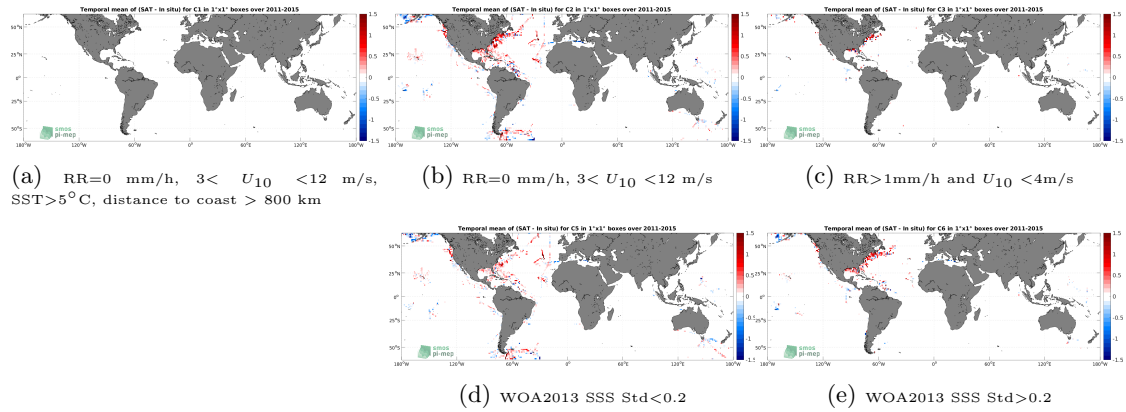
Figure 12: Temporal mean gridded over spatial boxes of size 1^\circ \times 1^\circ of \Delta\text{SSS} (Aquarius SSS L3 OR v5 - 7-Day running (NASA-GSFC) - TSG (SAMOS)) for 5 different subdatasets corresponding to:RR=0 mm/h, 3 < U_{10} < 12 m/s, SST >5^\circ\text{C} , distance to coast > 800 km (a), RR=0 mm/h, 3 < U_{10} < 12 m/s (b), RR >1 mm/h and U_{10} < 4 m/s (c), WOA2013 SSS Std <0.2 (d), WOA2013 SSS Std >0.2 (e).
