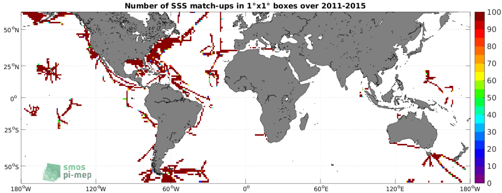
Figure 4: Number of SSS match-ups between TSG (SAMOS) SSS and the Aquarius SSS L3 OR v5 - 7-Day running (NASA-GSFC) SSS product for the SMOS coastal zone (<800km) 60N-60S Pi-MEP region over 1^\circ \times 1^\circ boxes and for the full satellite product period.
