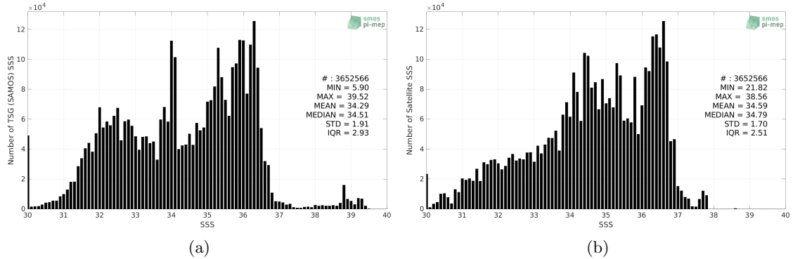
Figure 2: Histograms of SSS from TSG (SAMOS) (a) and Aquarius SSS L3 OR v5 - 7-Day running (NASA-GSFC) (b) considering all match-up pairs per bins of 0.1 over the SMOS coastal zone (<800km) 60N-60S Pi-MEP region and for the full satellite product period.
