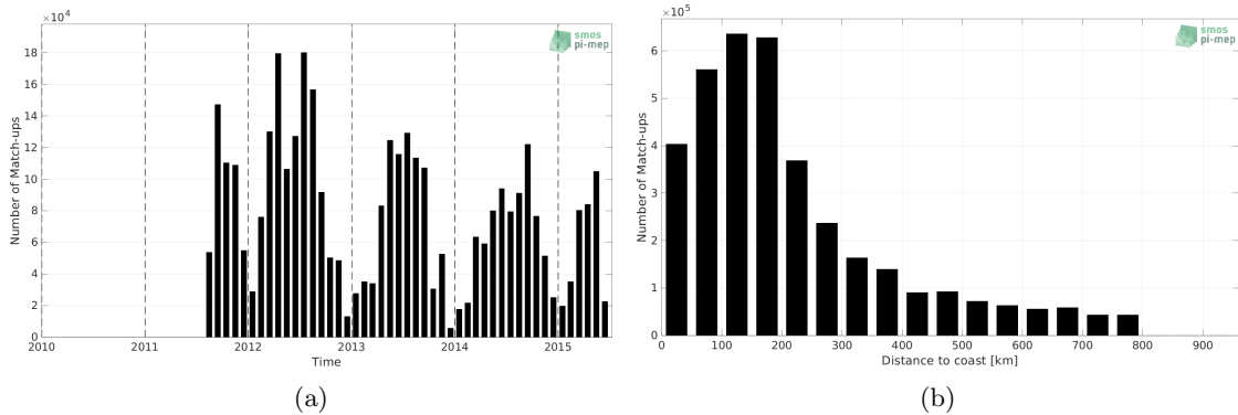
Figure 1: Number of match-ups between TSG (SAMOS) and Aquarius SSS L3 OR v5 - 7-Day running (NASA-GSFC) SSS as a function of time (a) and as function of the distance to coast (b) over the SMOS coastal zone (<800km) 60N-60S Pi-MEP region and for the full satellite product period.
