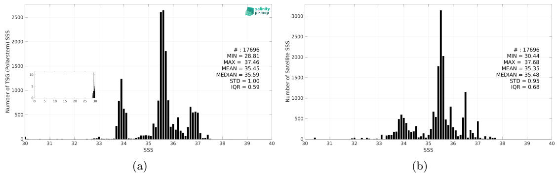
Figure 3: Histograms of SSS from TSG (Polarstern) (a) and Aquarius SSS L3 OR v5 - 7-Day running (NASA-GSFC) (b) considering all match-up pairs per bins of 0.1 over the SMOS coastal zone (<800km) 60N-60S Pi-MEP region and for the full satellite product period.
