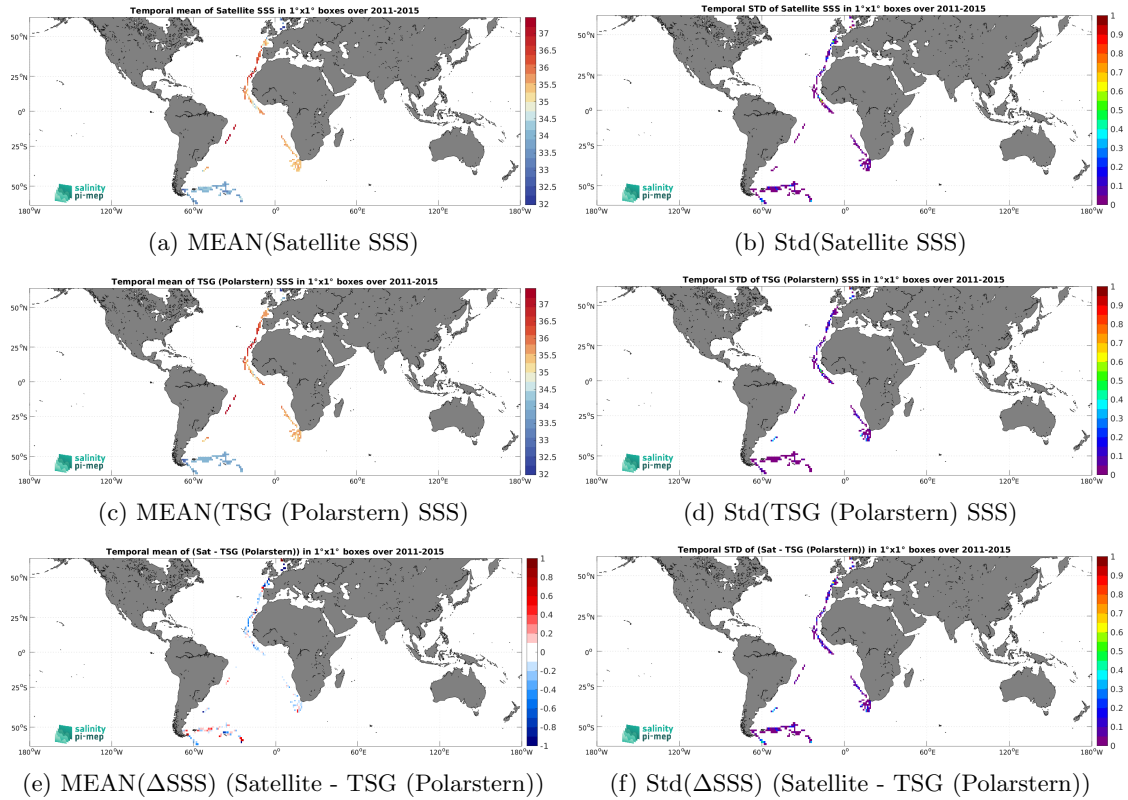
Figure 7: Temporal mean (left) and Std (right) of SSS from Aquarius SSS L3 OR v5 - 7-Day running (NASA-GSFC) (top), TSG (Polarstern) (middle), and of \Delta SSS (Satellite - TSG (Polarstern)). Only match-up pairs are used to generate these maps.
