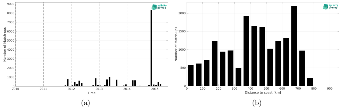
Figure 2: Number of match-ups between TSG (Polarstern) and Aquarius SSS L3 OR v5 - 7-Day running (NASA-GSFC) SSS as a function of time (a) and as function of the distance to coast (b) over the SMOS coastal zone (<800km) 60N-60S Pi-MEP region and for the full satellite product period.
