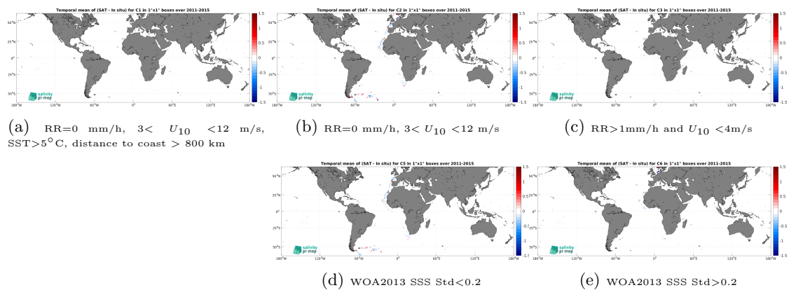
Figure 14: Temporal mean gridded over spatial boxes of size 1^\circ \times 1^\circ of \Delta\text{SSS} (Aquarius SSS L3 OR v5 - 7-Day running (NASA-GSFC) - TSG (Polarstern)) for 5 different subdatasets corresponding to:RR=0 mm/h, 3 < U_{10} < 12 m/s, SST>5°C, distance to coast > 800 km (a), RR=0 mm/h, 3 < U_{10} < 12 m/s (b), RR>1mm/h and U_{10} < 4 m/s (c), WOA2013 SSS Std<0.2 (d), WOA2013 SSS Std>0.2 (e).
