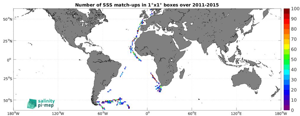
Figure 5: Number of SSS match-ups between TSG (Polarstern) SSS and the Aquarius SSS L3 OR v5 - 7-Day running (NASA-GSFC) SSS product for the SMOS coastal zone (<800km) 60N-60S Pi-MEP region over 1^\circ \times 1^\circ boxes and for the full satellite product period.
