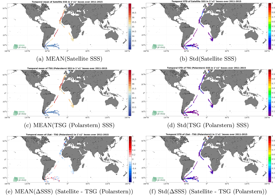
Figure 6: Temporal mean (left) and Std (right) of SSS from Aquarius SSS L3 OR v5 - 7-Day running (NASA-GSFC) (top), TSG (Polarstern) (middle), and of \Delta SSS (Satellite - TSG (Polarstern)). Only match-up pairs are used to generate these maps.
