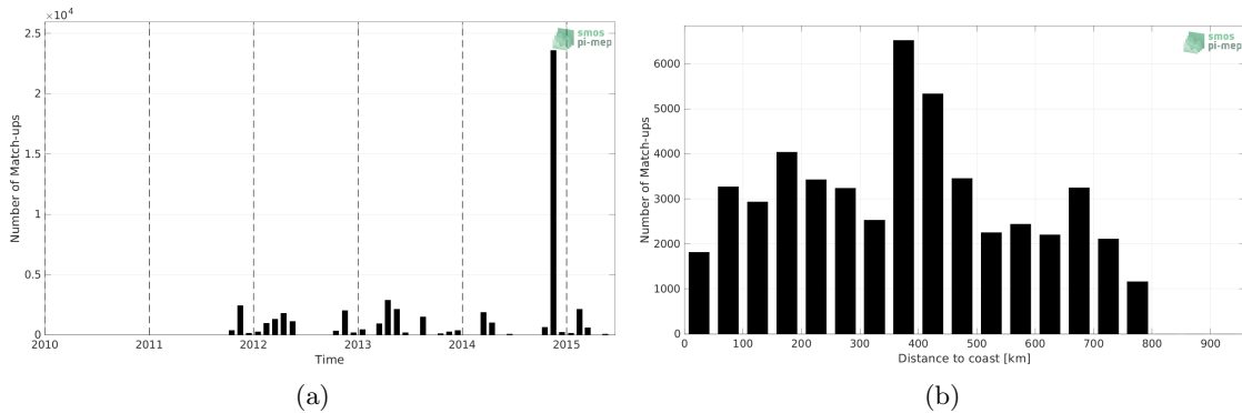
Figure 1: Number of match-ups between TSG (Polarstern) and Aquarius SSS L3 OR v5 - 7-Day running (NASA-GSFC) SSS as a function of time (a) and as function of the distance to coast (b) over the SMOS coastal zone (<800km) 60N-60S Pi-MEP region and for the full satellite product period.
