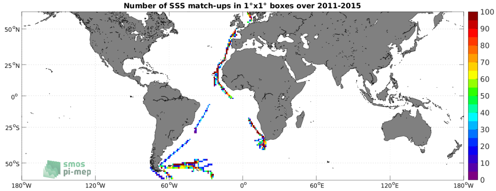
Figure 4: Number of SSS match-ups between TSG (Polarstern) SSS and the Aquarius SSS L3 OR v5 - 7-Day running (NASA-GSFC) SSS product for the SMOS coastal zone (<800km) 60N-60S Pi-MEP region over 1^\circ \times 1^\circ boxes and for the full satellite product period.
