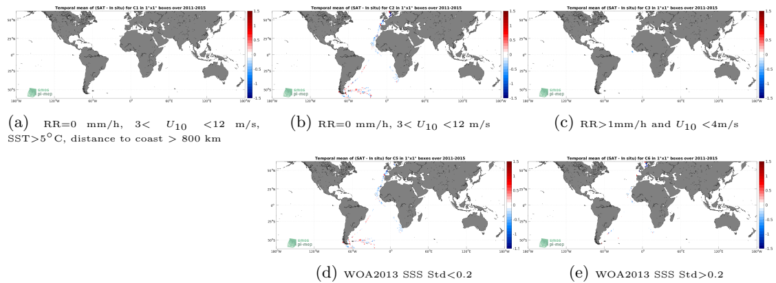
Figure 12: Temporal mean gridded over spatial boxes of size 1^\circ \times 1^\circ of \Delta SSS (Aquarius SSS L3 OR v5 - 7-Day running (NASA-GSFC) - TSG (Polarstern)) for 5 different subdatasets corresponding to:RR=0 mm/h, 3 < U_{10} < 12 m/s, SST >5^\circ C, distance to coast > 800 km (a), RR=0 mm/h, 3 < U_{10} < 12 m/s (b), RR >1 mm/h and U_{10} < 4 m/s (c), WOA2013 SSS Std <0.2 (d), WOA2013 SSS Std >0.2 (e).
