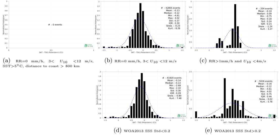
Figure 13: Normalized histogram of \Delta SSS (Aquarius SSS L3 OR v5 - 7-Day running (NASA-GSFC) - TSG (Polarstern)) for 5 different subdatasets corresponding to: RR=0 mm/h, 3 < U_{10} < 12 m/s, SST > 5°C, distance to coast > 800 km (a), RR=0 mm/h, 3 < U_{10} < 12 m/s (b), RR > 1mm/h and U_{10} < 4 m/s (c), WOA2013 SSS Std < 0.2 (d), WOA2013 SSS Std > 0.2 (e).
