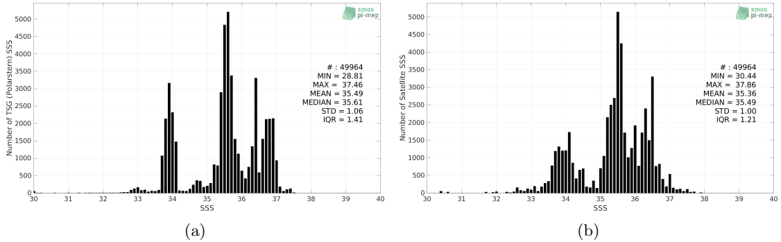
Figure 2: Histograms of SSS from TSG (Polarstern) (a) and Aquarius SSS L3 OR v5 - 7-Day running (NASA-GSFC) (b) considering all match-up pairs per bins of 0.1 over the SMOS coastal zone (<800km) 60N-60S Pi-MEP region and for the full satellite product period.
