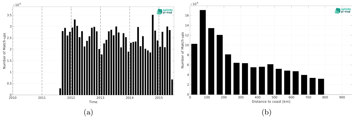
Figure 1: Number of match-ups between TSG (LEGOS-DM) and Aquarius SSS L3 OR v5 - 7-Day running (NASA-GSFC) SSS as a function of time (a) and as function of the distance to coast (b) over the SMOS coastal zone (<800km) 60N-60S Pi-MEP region and for the full satellite product period.
