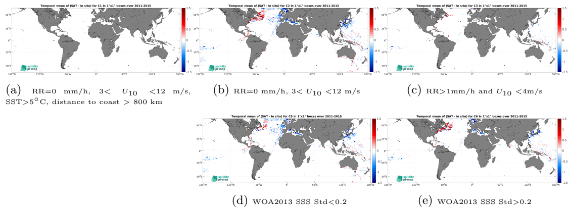
Figure 12: Temporal mean gridded over spatial boxes of size 1^\circ \times 1^\circ of \Delta\text{SSS} (Aquarius SSS L3 OR v5 - 7-Day running (NASA-GSFC) - TSG (LEGOS-DM)) for 5 different subdatasets corresponding to:RR=0 mm/h, 3 < U_{10} < 12 m/s, SST >5^\circ\text{C} , distance to coast > 800 km (a), RR=0 mm/h, 3 < U_{10} < 12 m/s (b), RR >1 mm/h and U_{10} < 4 m/s (c), WOA2013 SSS Std <0.2 (d), WOA2013 SSS Std >0.2 (e).
