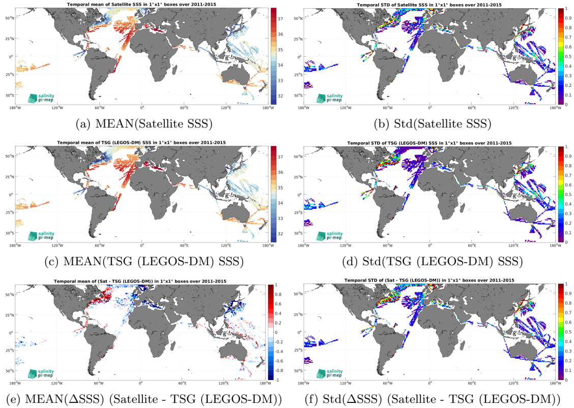
Figure 6: Temporal mean (left) and Std (right) of SSS from Aquarius SSS L3 OR v5 - 7-Day running (NASA-GSFC) (top), TSG (LEGOS-DM) (middle), and of \Delta\text{SSS} (Satellite - TSG (LEGOS-DM)). Only match-up pairs are used to generate these maps.
