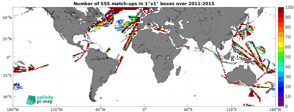
Figure 4: Number of SSS match-ups between TSG (LEGOS-DM) SSS and the Aquarius SSS L3 OR v5 - 7-Day running (NASA-GSFC) SSS product for the SMOS coastal zone ( <800\text{km} ) 60N-60S Pi-MEP region over 1^\circ \times 1^\circ boxes and for the full satellite product period.
