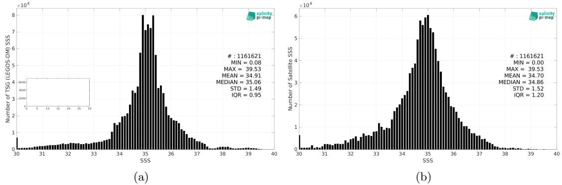
Figure 2: Histograms of SSS from TSG (LEGOS-DM) (a) and Aquarius SSS L3 OR v5 - 7-Day running (NASA-GSFC) (b) considering all match-up pairs per bins of 0.1 over the SMOS coastal zone (<800km) 60N-60S Pi-MEP region and for the full satellite product period.
