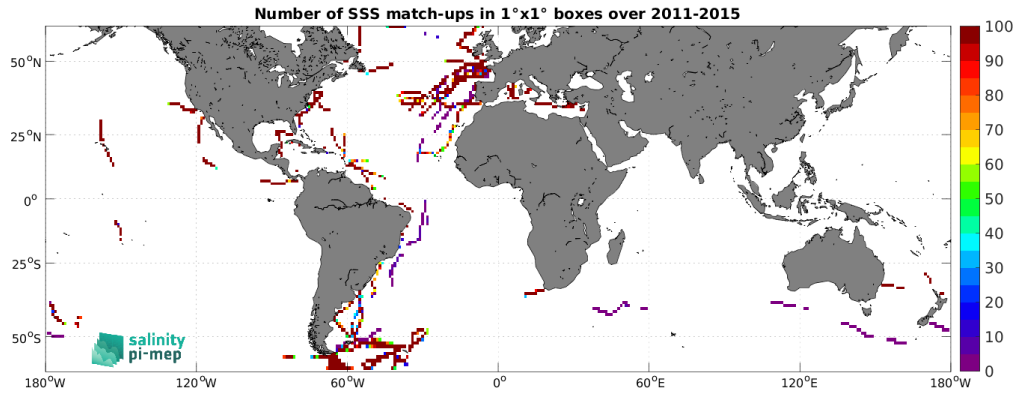
Figure 4: Number of SSS match-ups between TSG (GOSUD-Sailing-ship) SSS and the Aquarius SSS L3 OR v5 - 7-Day running (NASA-GSFC) SSS product for the SMOS coastal zone ( <800\text{km} ) 60N-60S Pi-MEP region over 1^\circ \times 1^\circ boxes and for the full satellite product period.
