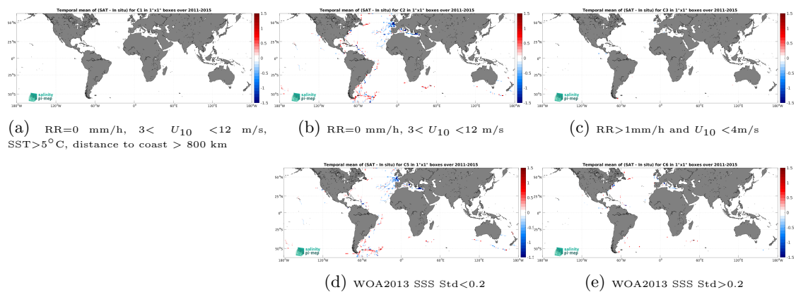
Figure 12: Temporal mean gridded over spatial boxes of size 1^\circ \times 1^\circ of \Delta\text{SSS} (Aquarius SSS L3 OR v5 - 7-Day running (NASA-GSFC) - TSG (GOSUD-Sailing-ship)) for 5 different subdatasets corresponding to: RR=0 mm/h, 3 < U_{10} < 12 m/s, SST > 5^\circ\text{C} , distance to coast > 800 km (a), RR=0 mm/h, 3 < U_{10} < 12 m/s (b), RR > 1 mm/h and U_{10} < 4 m/s (c), WOA2013 SSS Std < 0.2 (d), WOA2013 SSS Std > 0.2 (e).
