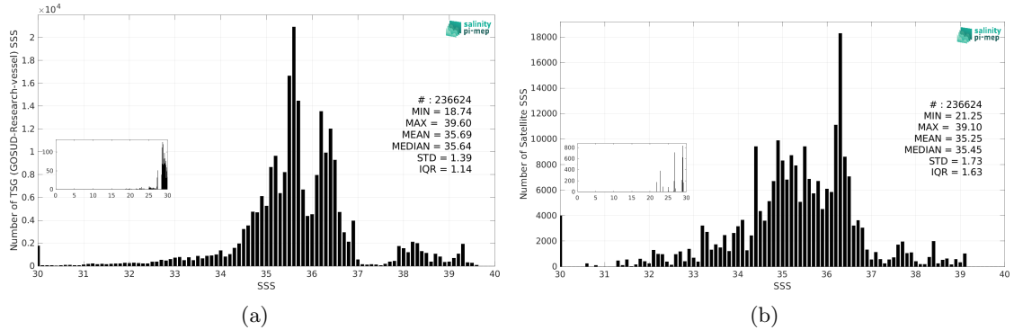
Figure 3: Histograms of SSS from TSG (GOSUD-Research-vessel) (a) and Aquarius SSS L3 OR v5 - 7-Day running (NASA-GSFC) (b) considering all match-up pairs per bins of 0.1 over the SMOS coastal zone (<800km) 60N-60S Pi-MEP region and for the full satellite product period.
