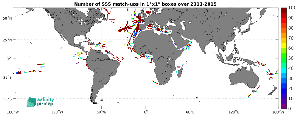
Figure 5: Number of SSS match-ups between TSG (GOSUD-Research-vessel) SSS and the Aquarius SSS L3 OR v5 - 7-Day running (NASA-GSFC) SSS product for the SMOS coastal zone (<800km) 60N-60S Pi-MEP region over 1^\circ \times 1^\circ boxes and for the full satellite product period.
