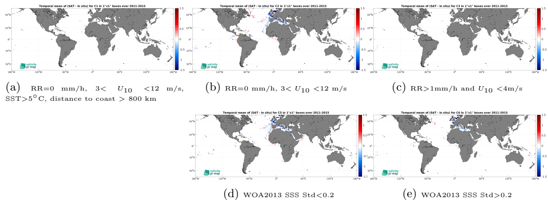
Figure 14: Temporal mean gridded over spatial boxes of size 1^\circ \times 1^\circ of \Delta SSS (Aquarius SSS L3 OR v5 - 7-Day running (NASA-GSFC) - TSG (GOSUD-Research-vessel)) for 5 different subdatasets corresponding to:RR=0 mm/h, 3 < U_{10} < 12 m/s, SST > 5^\circ\text{C} , distance to coast > 800 km (a), RR=0 mm/h, 3 < U_{10} < 12 m/s (b), RR > 1 mm/h and U_{10} < 4 m/s (c), WOA2013 SSS Std < 0.2 (d), WOA2013 SSS Std > 0.2 (e).
