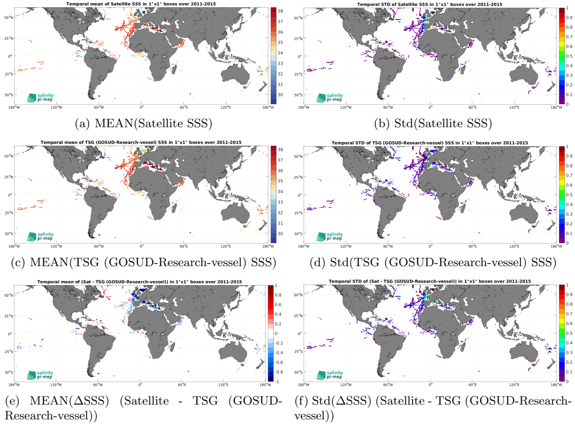
Figure 7: Temporal mean (left) and Std (right) of SSS from Aquarius SSS L3 OR v5 - 7-Day running (NASA-GSFC) (top), TSG (GOSUD-Research-vessel) (middle), and of \Delta\text{SSS} (Satellite - TSG (GOSUD-Research-vessel)). Only match-up pairs are used to generate these maps.
