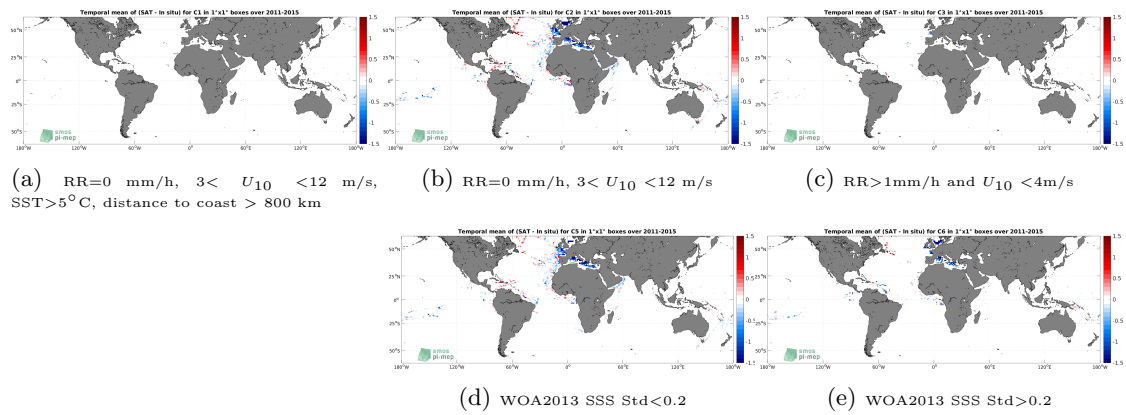
Figure 12: Temporal mean gridded over spatial boxes of size 1^\circ \times 1^\circ of \Delta SSS (Aquarius SSS L3 OR v5 - 7-Day running (NASA-GSFC) - TSG (GOSUD-Research-vessel)) for 5 different subdatasets corresponding to:RR=0 mm/h, 3 < U_{10} < 12 m/s, SST > 5^\circ\text{C} , distance to coast > 800 km (a), RR=0 mm/h, 3 < U_{10} < 12 m/s (b), RR > 1 mm/h and U_{10} < 4 m/s (c), WOA2013 SSS Std < 0.2 (d), WOA2013 SSS Std > 0.2 (e).
