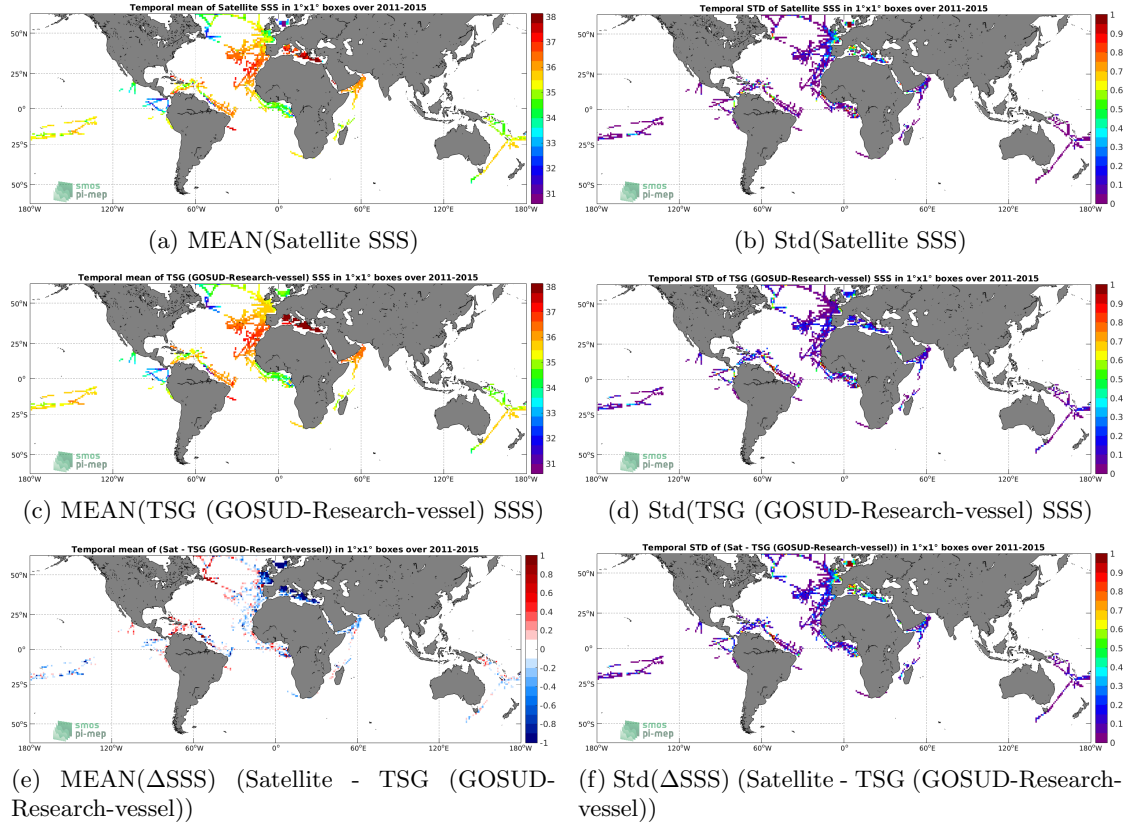
Figure 6: Temporal mean (left) and Std (right) of SSS from Aquarius SSS L3 OR v5 - 7-Day running (NASA-GSFC) (top), TSG (GOSUD-Research-vessel) (middle), and of \Delta SSS (Satellite - TSG (GOSUD-Research-vessel)). Only match-up pairs are used to generate these maps.
