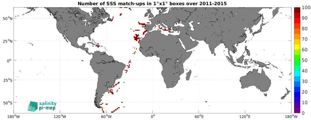
Figure 5: Number of SSS match-ups between TSG (CSIC-UTM) SSS and the Aquarius SSS L3 OR v5 - 7-Day running (NASA-GSFC) SSS product for the SMOS coastal zone (<800km) 60N-60S Pi-MEP region over 1^\circ \times 1^\circ boxes and for the full satellite product period.
