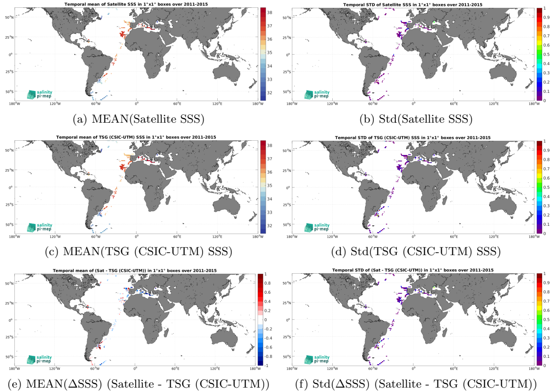
Figure 7: Temporal mean (left) and Std (right) of SSS from Aquarius SSS L3 OR v5 - 7-Day running (NASA-GSFC) (top), TSG (CSIC-UTM) (middle), and of \Delta SSS (Satellite - TSG (CSIC-UTM)). Only match-up pairs are used to generate these maps.
