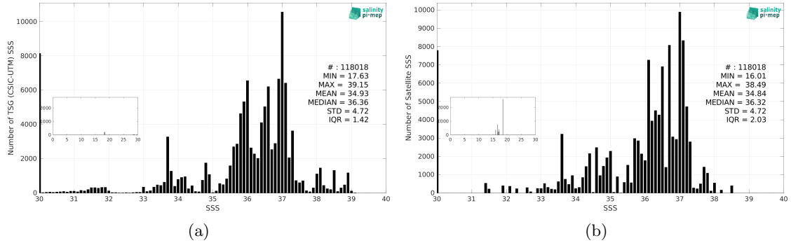
Figure 3: Histograms of SSS from TSG (CSIC-UTM) (a) and Aquarius SSS L3 OR v5 - 7-Day running (NASA-GSFC) (b) considering all match-up pairs per bins of 0.1 over the SMOS coastal zone (<800km) 60N-60S Pi-MEP region and for the full satellite product period.
