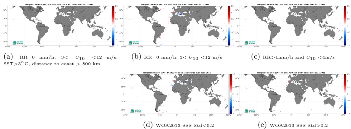
Figure 14: Temporal mean gridded over spatial boxes of size 1^\circ \times 1^\circ of \Delta\text{SSS} (Aquarius SSS L3 OR v5 - 7-Day running (NASA-GSFC) - TSG (CSIC-UTM)) for 5 different subdatasets corresponding to: RR=0 mm/h, 3 < U_{10} < 12 m/s, SST > 5^\circ\text{C} , distance to coast > 800 km (a), RR=0 mm/h, 3 < U_{10} < 12 m/s (b), RR > 1 mm/h and U_{10} < 4 m/s (c), WOA2013 SSS Std < 0.2 (d), WOA2013 SSS Std > 0.2 (e).
