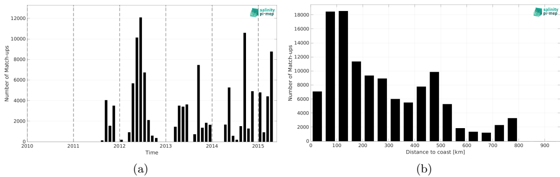
Figure 2: Number of match-ups between TSG (CSIC-UTM) and Aquarius SSS L3 OR v5 - 7-Day running (NASA-GSFC) SSS as a function of time (a) and as function of the distance to coast (b) over the SMOS coastal zone (<800km) 60N-60S Pi-MEP region and for the full satellite product period.
