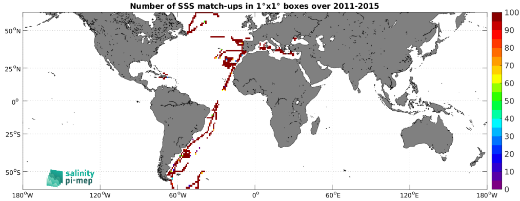
Figure 4: Number of SSS match-ups between TSG (CSIC-UTM) SSS and the Aquarius SSS L3 OR v5 - 7-Day running (NASA-GSFC) SSS product for the SMOS coastal zone (<800km) 60N-60S Pi-MEP region over 1^\circ \times 1^\circ boxes and for the full satellite product period.
