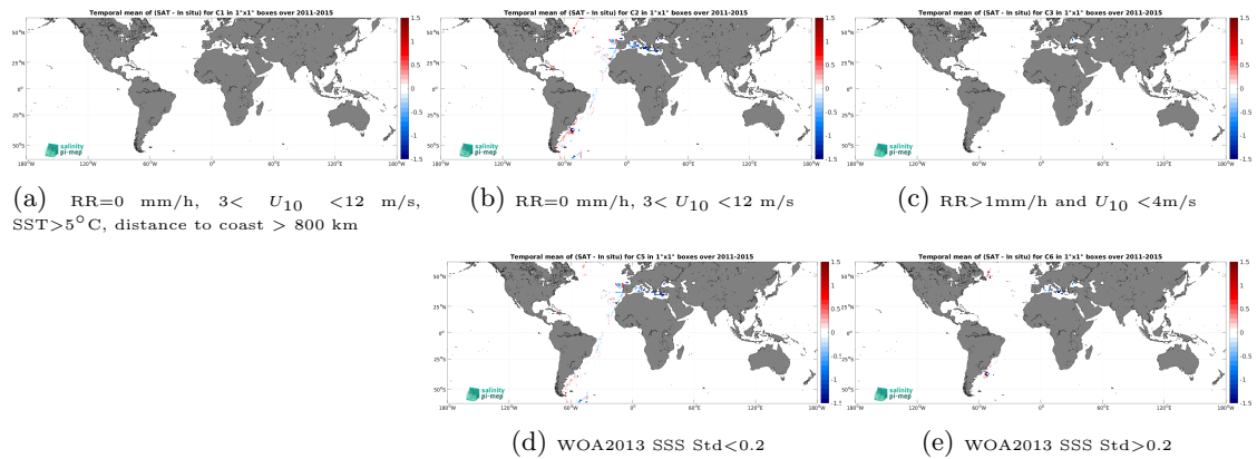
Figure 12: Temporal mean gridded over spatial boxes of size 1^\circ \times 1^\circ of \Delta\text{SSS} (Aquarius SSS L3 OR v5 - 7-Day running (NASA-GSFC) - TSG (CSIC-UTM)) for 5 different subdatasets corresponding to: RR=0 mm/h, 3 < U_{10} < 12 m/s, SST > 5^\circ\text{C} , distance to coast > 800 km (a), RR=0 mm/h, 3 < U_{10} < 12 m/s (b), RR > 1 mm/h and U_{10} < 4 m/s (c), WOA2013 SSS Std < 0.2 (d), WOA2013 SSS Std > 0.2 (e).
