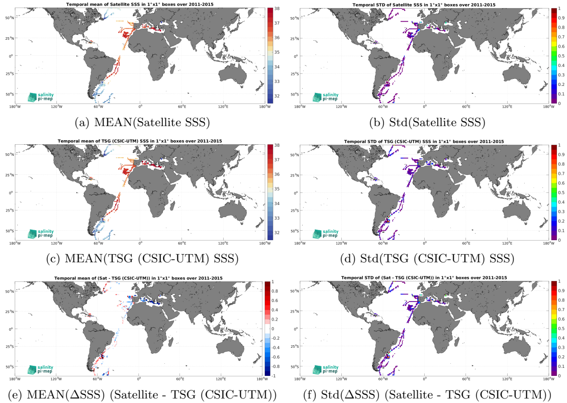
Figure 6: Temporal mean (left) and Std (right) of SSS from Aquarius SSS L3 OR v5 - 7-Day running (NASA-GSFC) (top), TSG (CSIC-UTM) (middle), and of \Delta SSS (Satellite - TSG (CSIC-UTM)). Only match-up pairs are used to generate these maps.
