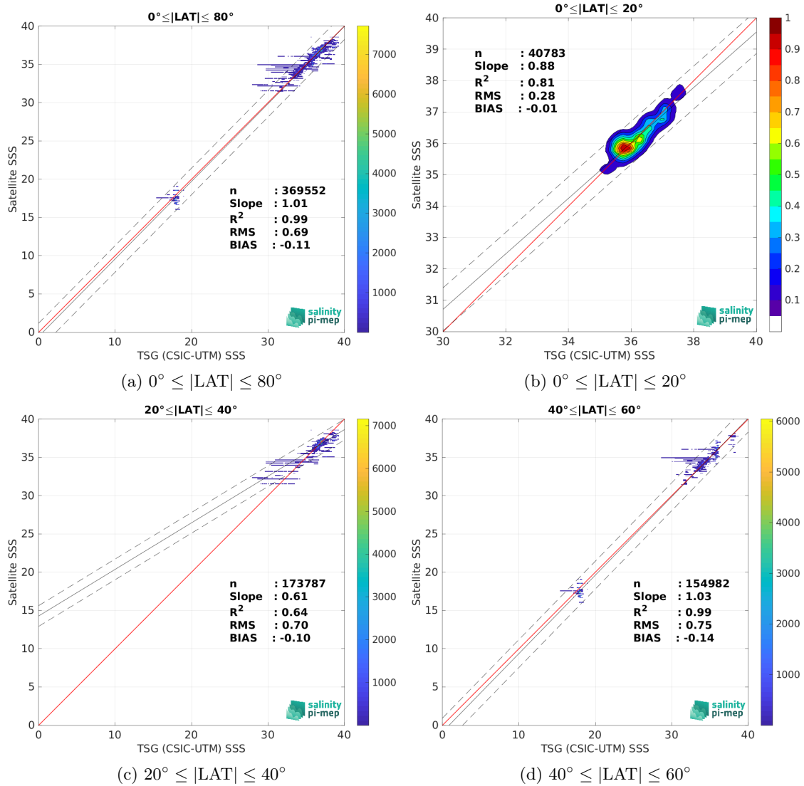
Figure 9: Contour maps of the concentration of Aquarius SSS L3 OR v5 - 7-Day running (NASA-GSFC) SSS (y-axis) versus TSG (CSIC-UTM) SSS (x-axis) at match-up pairs for different latitude bands. For each plot, the red line shows x=y . The black thin and dashed lines indicate a linear fit through the data cloud and the \pm 95\% confidence levels, respectively. The number match-up pairs n , the slope and R^2 coefficient of the linear fit, the root mean square (RMS) and the mean bias between satellite and in situ data are indicated for each latitude band in each plots.
