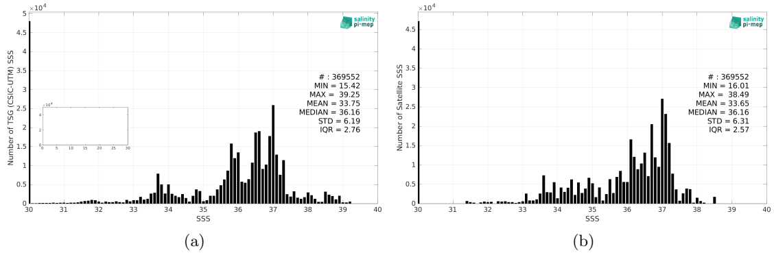
Figure 2: Histograms of SSS from TSG (CSIC-UTM) (a) and Aquarius SSS L3 OR v5 - 7-Day running (NASA-GSFC) (b) considering all match-up pairs per bins of 0.1 over the SMOS coastal zone (<800km) 60N-60S Pi-MEP region and for the full satellite product period.
