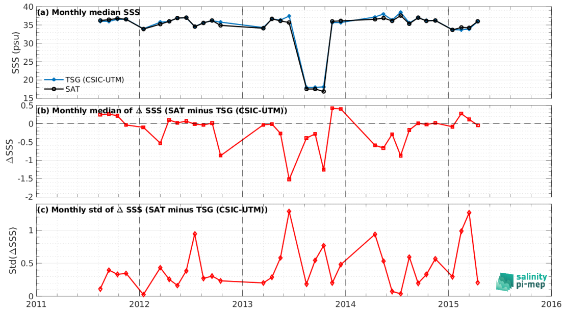
Figure 7: Time series of the monthly median SSS (top), median of \Delta SSS (Satellite - TSG (CSIC-UTM)) and Std of \Delta SSS (Satellite - TSG (CSIC-UTM)) over the SMOS coastal zone ( <800 km) 60N-60S Pi-MEP region considering all match-ups collected by the Pi-MEP.
