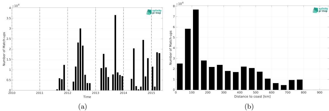
Figure 1: Number of match-ups between TSG (CSIC-UTM) and Aquarius SSS L3 OR v5 - 7-Day running (NASA-GSFC) SSS as a function of time (a) and as function of the distance to coast (b) over the SMOS coastal zone (<800km) 60N-60S Pi-MEP region and for the full satellite product period.
