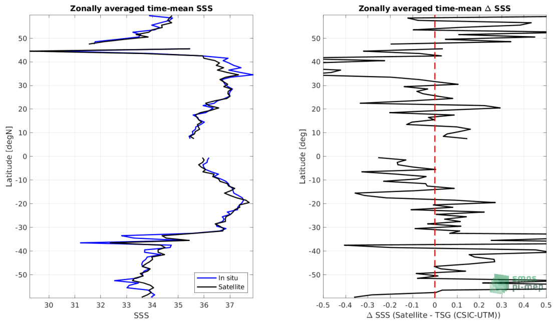
Figure 8: Left panel: Zonal mean SSS from Aquarius SSS L3 OR v5 - 7-Day running (NASA-GSFC) satellite product (black) and from TSG (CSIC-UTM) (blue). Right panel: Zonal mean of \Delta\text{SSS} (Satellite - TSG (CSIC-UTM)) for all the collected Pi-MEP match-up pairs estimated over the full satellite product period.
