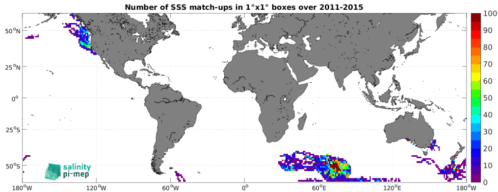
Figure 4: Number of SSS match-ups between Marine mammals SSS and the Aquarius SSS L3 OR v5 - 7-Day running (NASA-GSFC) SSS product for the SMOS coastal zone (<800km) 60N-60S Pi-MEP region over 1°x1° boxes and for the full satellite product period.
