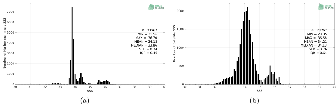
Figure 2: Histograms of SSS from Marine mammals (a) and Aquarius SSS L3 OR v5 - 7-Day running (NASA-GSFC) (b) considering all match-up pairs per bins of 0.1 over the SMOS coastal zone (<800km) 60N-60S Pi-MEP region and for the full satellite product period.
