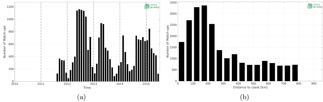
Figure 1: Number of match-ups between Marine mammals and Aquarius SSS L3 OR v5 - 7-Day running (NASA-GSFC) SSS as a function of time (a) and as function of the distance to coast (b) over the SMOS coastal zone (<800km) 60N-60S Pi-MEP region and for the full satellite product period.
