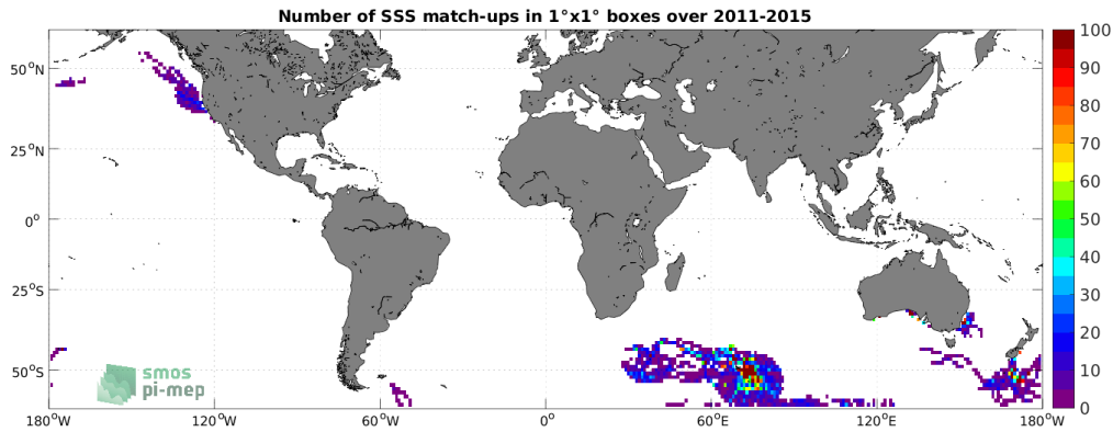
Figure 4: Number of SSS match-ups between Marine mammals SSS and the Aquarius SSS L3 OR v5 - 7-Day running (NASA-GSFC) SSS product for the SMOS coastal zone (<800km) 60N-60S Pi-MEP region over 1°×1° boxes and for the full satellite product period.
