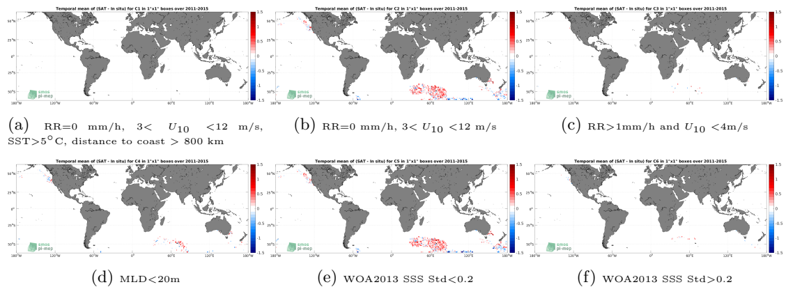
Figure 12: Temporal mean gridded over spatial boxes of size 1^\circ \times 1^\circ of \Delta SSS (Aquarius SSS L3 OR v5 - 7-Day running (NASA-GSFC) - Marine mammals) for 6 different subdatasets corresponding to:RR=0 mm/h, 3 < U_{10} < 12 m/s, SST > 5^\circ C, distance to coast > 800 km (a), RR=0 mm/h, 3 < U_{10} < 12 m/s (b), RR > 1 mm/h and U_{10} < 4 m/s (c),MLD < 20 m (d),WOA2013 SSS Std < 0.2 (e),WOA2013 SSS Std > 0.2 (f).
