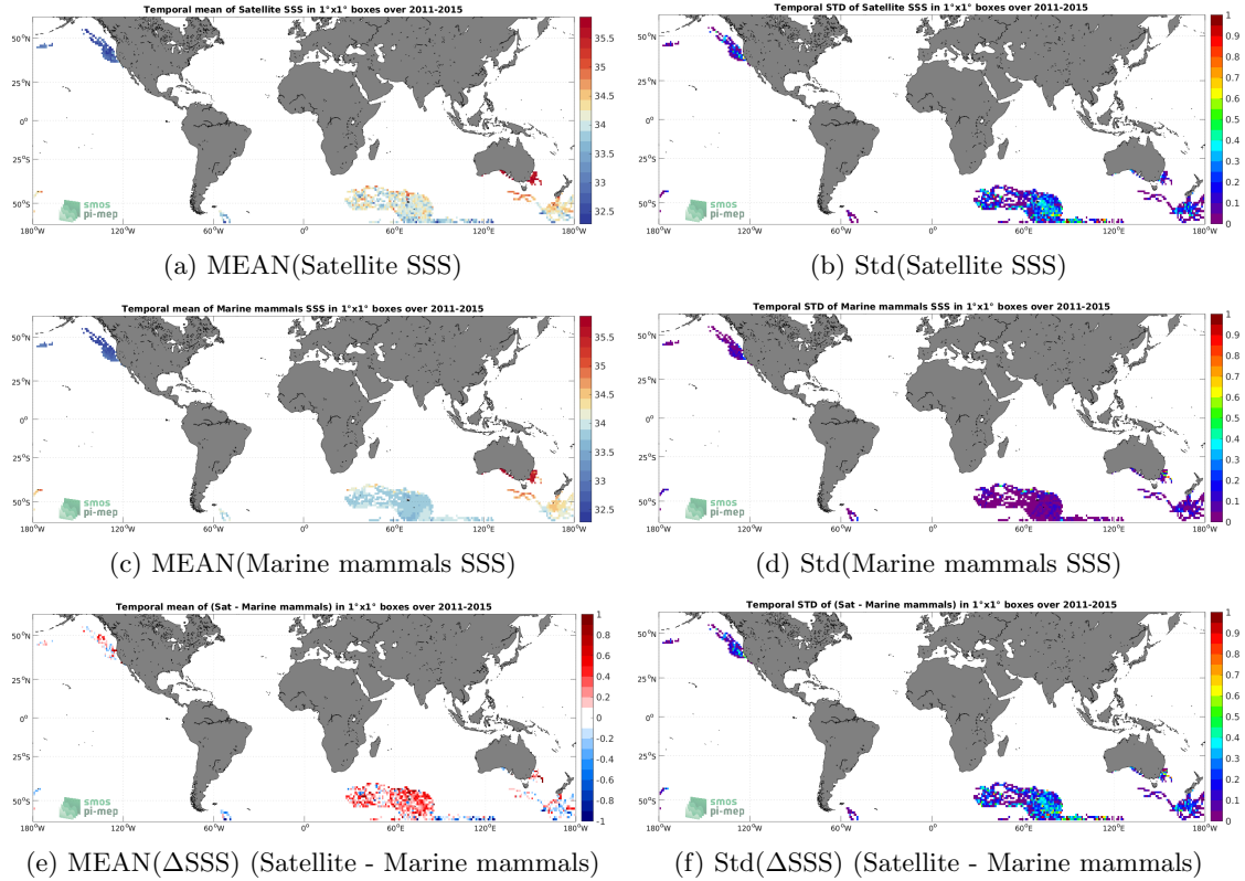
Figure 6: Temporal mean (left) and Std (right) of SSS from Aquarius SSS L3 OR v5 - 7-Day running (NASA-GSFC) (top), Marine mammals (middle), and of \Delta SSS (Satellite - Marine mammals). Only match-up pairs are used to generate these maps.
