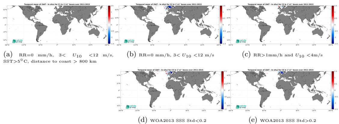
Figure 14: Temporal mean gridded over spatial boxes of size 1^\circ \times 1^\circ of \Delta SSS (Aquarius SSS L3 OR v5 - 7-Day running (NASA-GSFC) - ICES) for 5 different subdatasets corresponding to:RR=0 mm/h, 3 < U_{10} < 12 m/s, SST >5^\circ\text{C} , distance to coast > 800 km (a), RR=0 mm/h, 3 < U_{10} < 12 m/s (b), RR >1 mm/h and U_{10} < 4 m/s (c), WOA2013 SSS Std <0.2 (d), WOA2013 SSS Std >0.2 (e).
