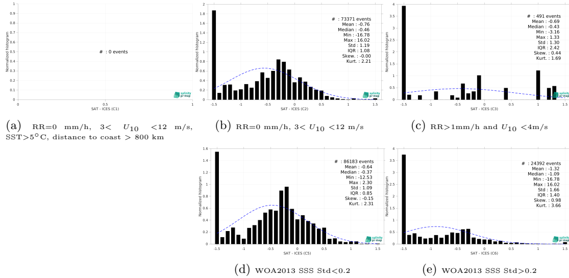
Figure 15: Normalized histogram of \Delta SSS (Aquarius SSS L3 OR v5 - 7-Day running (NASA-GSFC) - ICES) for 5 different subdatasets corresponding to: RR=0 mm/h, 3 < U_{10} < 12 m/s, SST > 5°C, distance to coast > 800 km (a), RR=0 mm/h, 3 < U_{10} < 12 m/s (b), RR > 1mm/h and U_{10} < 4 m/s (c), WOA2013 SSS Std < 0.2 (d), WOA2013 SSS Std > 0.2 (e).
