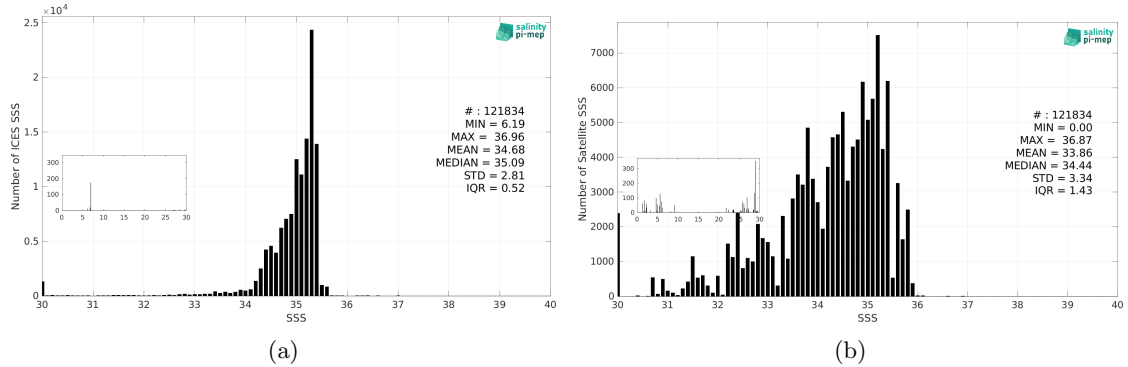
Figure 3: Histograms of SSS from ICES (a) and Aquarius SSS L3 OR v5 - 7-Day running (NASA-GSFC) (b) considering all match-up pairs per bins of 0.1 over the SMOS coastal zone (<800km) 60N-60S Pi-MEP region and for the full satellite product period.
