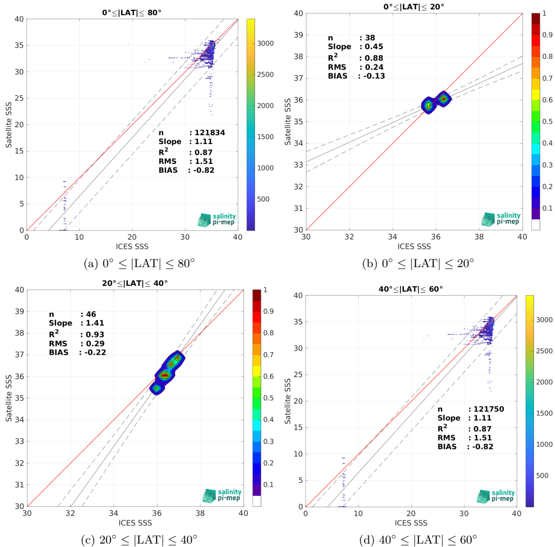
Figure 10: Contour maps of the concentration of Aquarius SSS L3 OR v5 - 7-Day running (NASA-GSFC) SSS (y-axis) versus ICES SSS (x-axis) at match-up pairs for different latitude bands. For each plot, the red line shows x=y . The black thin and dashed lines indicate a linear fit through the data cloud and the \pm 95\% confidence levels, respectively. The number match-up pairs n , the slope and R^2 coefficient of the linear fit, the root mean square (RMS) and the mean bias between satellite and in situ data are indicated for each latitude band in each plots.
