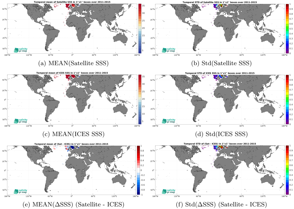
Figure 7: Temporal mean (left) and Std (right) of SSS from Aquarius SSS L3 OR v5 - 7-Day running (NASA-GSFC) (top), ICES (middle), and of \Delta SSS (Satellite - ICES). Only match-up pairs are used to generate these maps.
