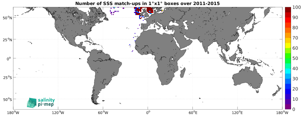
Figure 5: Number of SSS match-ups between ICES SSS and the Aquarius SSS L3 OR v5 - 7-Day running (NASA-GSFC) SSS product for the SMOS coastal zone (<800km) 60N-60S Pi-MEP region over 1^\circ \times 1^\circ boxes and for the full satellite product period.
