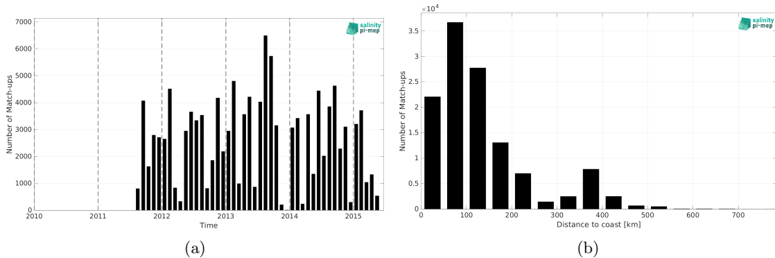
Figure 2: Number of match-ups between ICES and Aquarius SSS L3 OR v5 - 7-Day running (NASA-GSFC) SSS as a function of time (a) and as function of the distance to coast (b) over the SMOS coastal zone (<800km) 60N-60S Pi-MEP region and for the full satellite product period.
