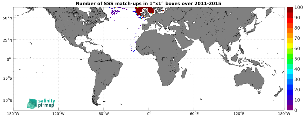
Figure 4: Number of SSS match-ups between ICES SSS and the Aquarius SSS L3 OR v5 - 7-Day running (NASA-GSFC) SSS product for the SMOS coastal zone (<800km) 60N-60S Pi-MEP region over 1^\circ \times 1^\circ boxes and for the full satellite product period.
