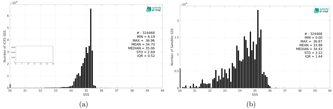
Figure 2: Histograms of SSS from ICES (a) and Aquarius SSS L3 OR v5 - 7-Day running (NASA-GSFC) (b) considering all match-up pairs per bins of 0.1 over the SMOS coastal zone (<800km) 60N-60S Pi-MEP region and for the full satellite product period.
