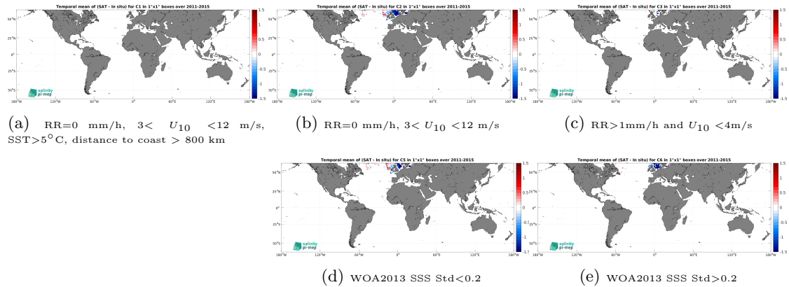
Figure 12: Temporal mean gridded over spatial boxes of size 1^\circ \times 1^\circ of \Delta SSS (Aquarius SSS L3 OR v5 - 7-Day running (NASA-GSFC) - ICES) for 5 different subdatasets corresponding to:RR=0 mm/h, 3 < U_{10} < 12 m/s, SST >5^\circ C, distance to coast > 800 km (a), RR=0 mm/h, 3 < U_{10} < 12 m/s (b), RR >1 mm/h and U_{10} < 4 m/s (c), WOA2013 SSS Std <0.2 (d), WOA2013 SSS Std >0.2 (e).
