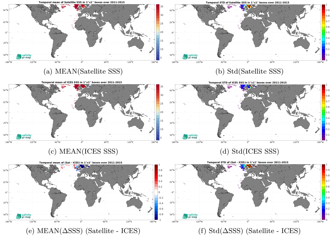
Figure 6: Temporal mean (left) and Std (right) of SSS from Aquarius SSS L3 OR v5 - 7-Day running (NASA-GSFC) (top), ICES (middle), and of \Delta SSS (Satellite - ICES). Only match-up pairs are used to generate these maps.
