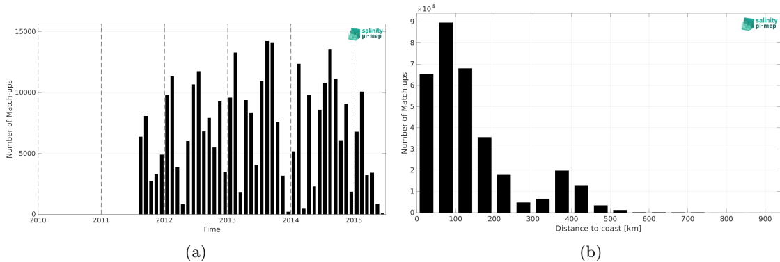
Figure 1: Number of match-ups between ICES and Aquarius SSS L3 OR v5 - 7-Day running (NASA-GSFC) SSS as a function of time (a) and as function of the distance to coast (b) over the SMOS coastal zone (<800km) 60N-60S Pi-MEP region and for the full satellite product period.
