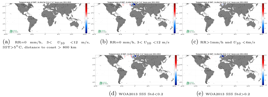
Figure 12: Temporal mean gridded over spatial boxes of size 1^\circ \times 1^\circ of \Delta\text{SSS} (Aquarius SSS L3 OR v5 - 7-Day running (NASA-GSFC) - ICES) for 5 different subdatasets corresponding to:RR=0 mm/h, 3 < U_{10} < 12 m/s, SST >5^\circ\text{C} , distance to coast > 800 km (a), RR=0 mm/h, 3 < U_{10} < 12 m/s (b), RR >1 mm/h and U_{10} < 4 m/s (c), WOA2013 SSS Std <0.2 (d), WOA2013 SSS Std >0.2 (e).
