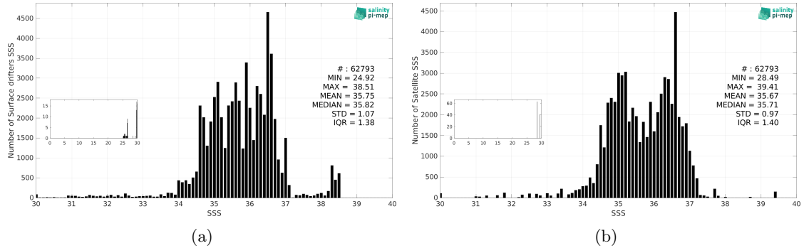
Figure 3: Histograms of SSS from Surface drifters (a) and Aquarius SSS L3 OR v5 - 7-Day running (NASA-GSFC) (b) considering all match-up pairs per bins of 0.1 over the SMOS coastal zone (<800km) 60N-60S Pi-MEP region and for the full satellite product period.
