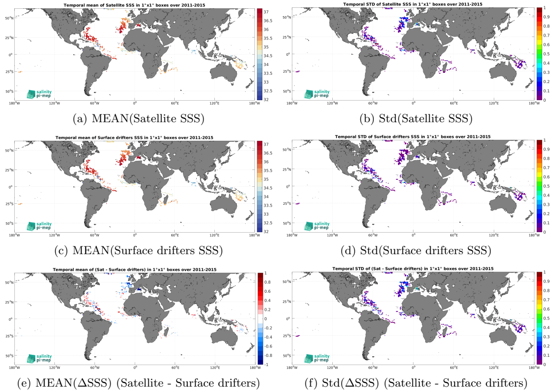
Figure 6: Temporal mean (left) and Std (right) of SSS from Aquarius SSS L3 OR v5 - 7-Day running (NASA-GSFC) (top), Surface drifters (middle), and of \Delta SSS (Satellite - Surface drifters). Only match-up pairs are used to generate these maps.
