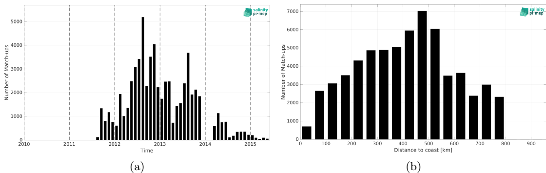
Figure 2: Number of match-ups between Surface drifters and Aquarius SSS L3 OR v5 - 7-Day running (NASA-GSFC) SSS as a function of time (a) and as function of the distance to coast (b) over the SMOS coastal zone (<800km) 60N-60S Pi-MEP region and for the full satellite product period.
