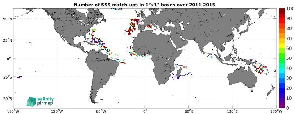
Figure 4: Number of SSS match-ups between Surface drifters SSS and the Aquarius SSS L3 OR v5 - 7-Day running (NASA-GSFC) SSS product for the SMOS coastal zone (<800km) 60N-60S Pi-MEP region over 1^\circ \times 1^\circ boxes and for the full satellite product period.
