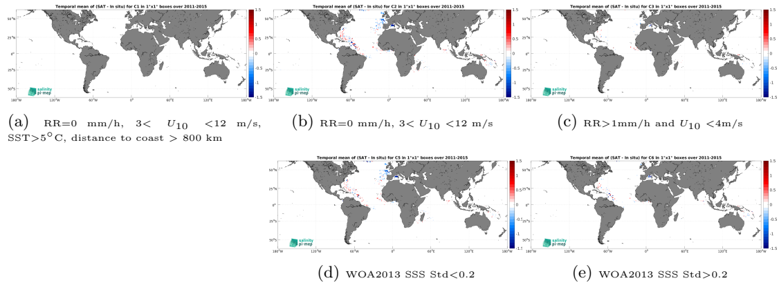
Figure 13: Temporal mean gridded over spatial boxes of size 1^\circ \times 1^\circ of \Delta\text{SSS} (Aquarius SSS L3 OR v5 - 7-Day running (NASA-GSFC) - Surface drifters) for 5 different subdatasets corresponding to:RR=0 mm/h, 3 < U_{10} < 12 m/s, SST >5^\circ\text{C} , distance to coast > 800 km (a), RR=0 mm/h, 3 < U_{10} < 12 m/s (b), RR >1 mm/h and U_{10} < 4 m/s (c), WOA2013 SSS Std <0.2 (d), WOA2013 SSS Std >0.2 (e).
