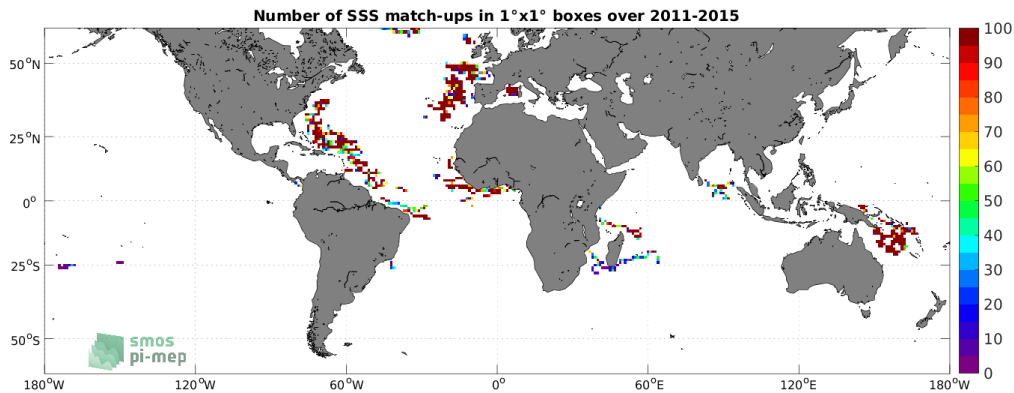
Figure 3: Number of SSS match-ups between Surface drifters SSS and the Aquarius SSS L3 OR v5 - 7-Day running (NASA-GSFC) SSS product for the SMOS coastal zone (<800km) 60N-60S Pi-MEP region over 1^\circ \times 1^\circ boxes and for the full satellite product period.
