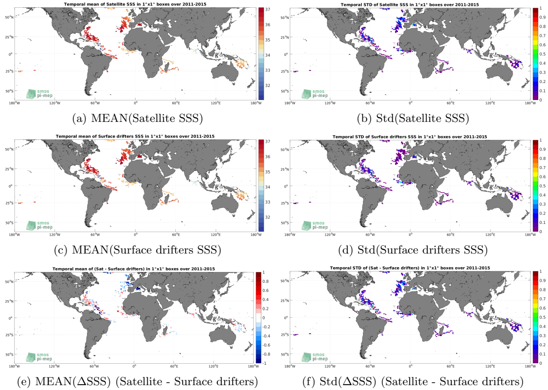
Figure 5: Temporal mean (left) and Std (right) of SSS from Aquarius SSS L3 OR v5 - 7-Day running (NASA-GSFC) (top), Surface drifters (middle), and of \Delta SSS (Satellite - Surface drifters). Only match-up pairs are used to generate these maps.
