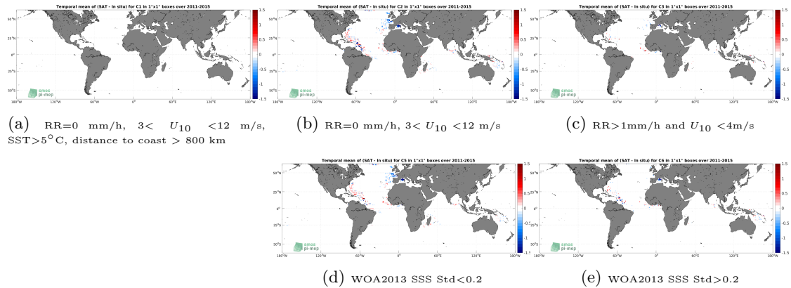
Figure 11: Temporal mean gridded over spatial boxes of size 1^\circ \times 1^\circ of \Delta\text{SSS} (Aquarius SSS L3 OR v5 - 7-Day running (NASA-GSFC) - Surface drifters) for 5 different subdatasets corresponding to:RR=0 mm/h, 3 < U_{10} < 12 m/s, SST >5^\circ\text{C} , distance to coast > 800 km (a), RR=0 mm/h, 3 < U_{10} < 12 m/s (b), RR >1 mm/h and U_{10} < 4 m/s (c), WOA2013 SSS Std <0.2 (d), WOA2013 SSS Std >0.2 (e).
