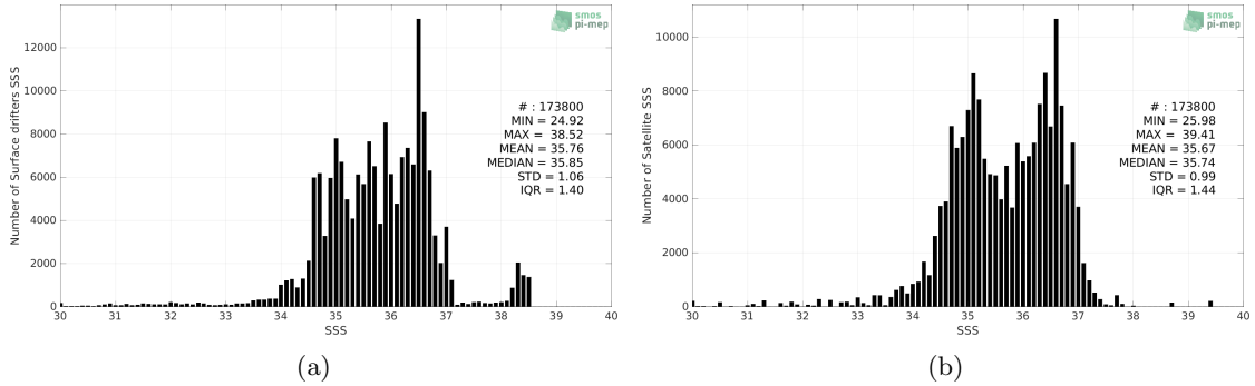
Figure 2: Histograms of SSS from Surface drifters (a) and Aquarius SSS L3 OR v5 - 7-Day running (NASA-GSFC) (b) considering all match-up pairs per bins of 0.1 over the SMOS coastal zone (<800km) 60N-60S Pi-MEP region and for the full satellite product period.
