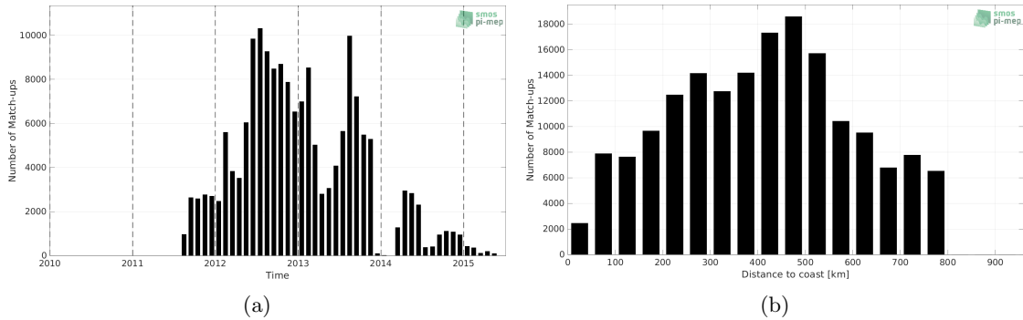
Figure 1: Number of match-ups between Surface drifters and Aquarius SSS L3 OR v5 - 7-Day running (NASA-GSFC) SSS as a function of time (a) and as function of the distance to coast (b) over the SMOS coastal zone (<800km) 60N-60S Pi-MEP region and for the full satellite product period.
