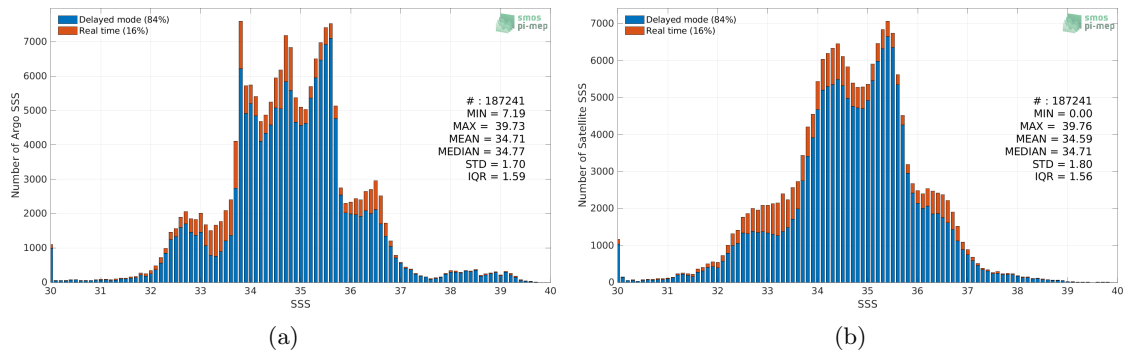
Figure 2: Histograms of SSS from Argo (a) and Aquarius SSS L3 OR v5 - 7-Day running (NASA-GSFC) (b) considering all match-up pairs per bins of 0.1 over the SMOS coastal zone (<800km) 60N-60S Pi-MEP region and for the full satellite product period.
