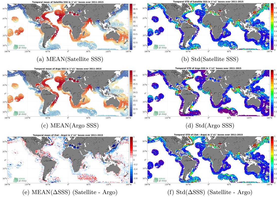
Figure 6: Temporal mean (left) and Std (right) of SSS from Aquarius SSS L3 OR v5 - 7-Day running (NASA-GSFC) (top), Argo (middle), and of \Delta SSS (Satellite - Argo). Only match-up pairs are used to generate these maps.
