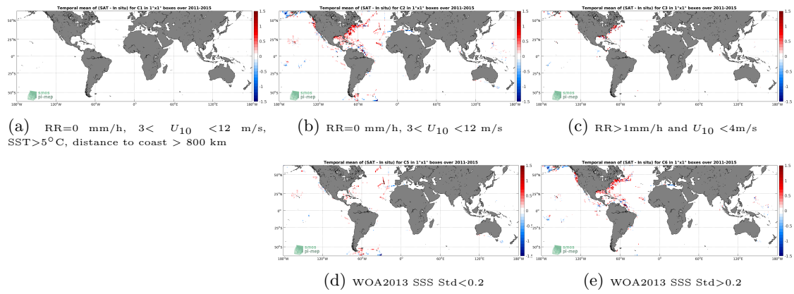
Figure 12: Temporal mean gridded over spatial boxes of size 1^\circ \times 1^\circ of \Delta\text{SSS} (Aquarius SSS L3 OR v5 - 7-Day running - Rain mask (NASA-GSFC) - TSG (SAMOS)) for 5 different subdatasets corresponding to:RR=0 mm/h, 3 < U_{10} < 12 m/s, SST >5^\circ\text{C} , distance to coast > 800 km (a), RR=0 mm/h, 3 < U_{10} < 12 m/s (b), RR >1 mm/h and U_{10} < 4 m/s (c), WOA2013 SSS Std <0.2 (d), WOA2013 SSS Std >0.2 (e).
