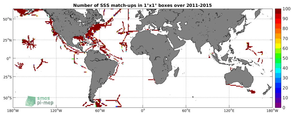
Figure 4: Number of SSS match-ups between TSG-SAMOS SSS and the Aquarius-L3-OR-V5-7DAY-RUNNING-RAIN-MASK-1DEG SSS product for the SMOS coastal zone ( \approx 800\text{km} ) 60N-60S Pi-MEP region over 1^\circ \times 1^\circ boxes and for the full satellite product period.
