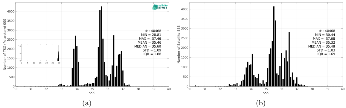
Figure 3: Histograms of SSS from TSG (Polarstern) (a) and Aquarius SSS L3 OR v5 - 7-Day running - Rain mask (NASA-GSFC) (b) considering all match-up pairs per bins of 0.1 over the SMOS coastal zone (<800km) 60N-60S Pi-MEP region and for the full satellite product period.
