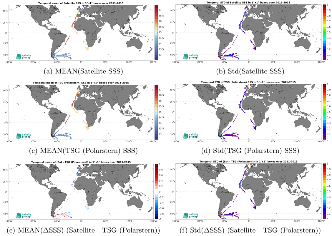
Figure 7: Temporal mean (left) and Std (right) of SSS from Aquarius SSS L3 OR v5 - 7-Day running - Rain mask (NASA-GSFC) (top), TSG (Polarstern) (middle), and of \Delta SSS (Satellite - TSG (Polarstern)). Only match-up pairs are used to generate these maps.
