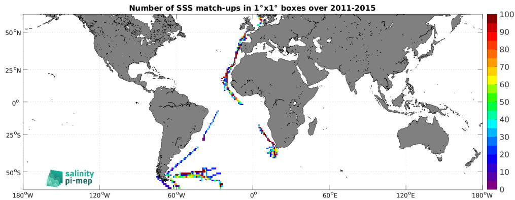
Figure 5: Number of SSS match-ups between TSG (Polarstern) SSS and the Aquarius SSS L3 OR v5 - 7-Day running - Rain mask (NASA-GSFC) SSS product for the SMOS coastal zone (<800km) 60N-60S Pi-MEP region over 1^\circ \times 1^\circ boxes and for the full satellite product period.
