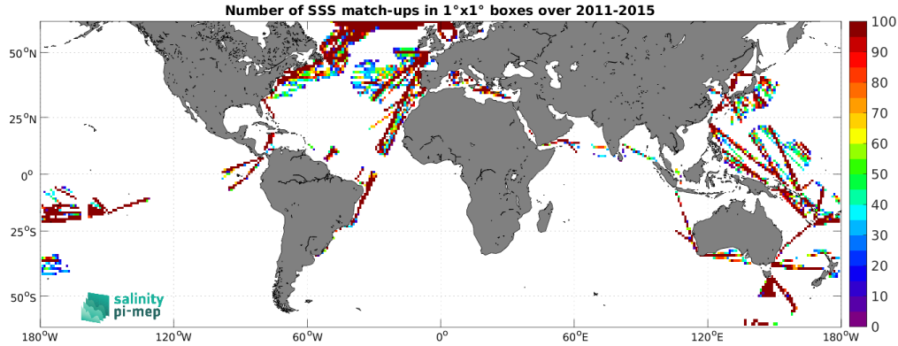
Figure 5: Number of SSS match-ups between TSG (LEGOS-DM) SSS and the Aquarius SSS L3 OR v5 - 7-Day running - Rain mask (NASA-GSFC) SSS product for the SMOS coastal zone (<800km) 60N-60S Pi-MEP region over 1^\circ \times 1^\circ boxes and for the full satellite product period.
