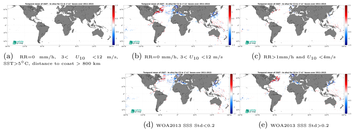
Figure 14: Temporal mean gridded over spatial boxes of size 1^\circ \times 1^\circ of \Delta SSS (Aquarius SSS L3 OR v5 - 7-Day running - Rain mask (NASA-GSFC) - TSG (LEGOS-DM)) for 5 different subdatasets corresponding to:RR=0 mm/h, 3 < U_{10} < 12 m/s, SST >5^\circ\text{C} , distance to coast > 800 km (a), RR=0 mm/h, 3 < U_{10} < 12 m/s (b), RR >1 mm/h and U_{10} < 4 m/s (c), WOA2013 SSS Std <0.2 (d), WOA2013 SSS Std >0.2 (e).
