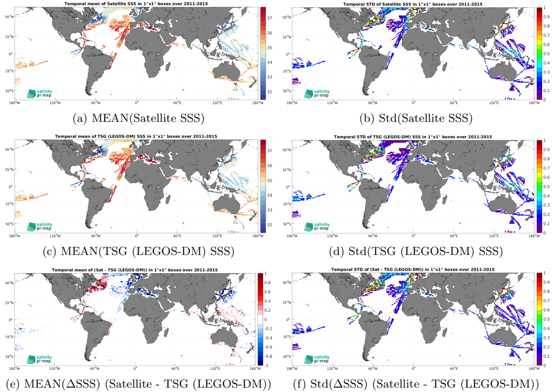
Figure 7: Temporal mean (left) and Std (right) of SSS from Aquarius SSS L3 OR v5 - 7-Day running - Rain mask (NASA-GSFC) (top), TSG (LEGOS-DM) (middle), and of \Delta\text{SSS} (Satellite - TSG (LEGOS-DM)). Only match-up pairs are used to generate these maps.
