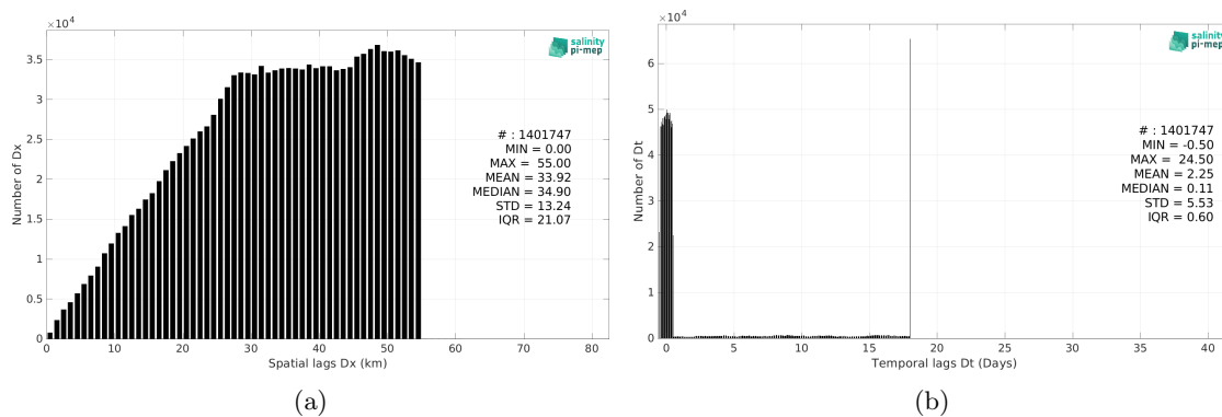
Figure 5: Histograms of the spatial (a) and temporal (b) lags between the location/time of the TSG (LEGOS-DM) measurement and the date of the corresponding Aquarius SSS L3 OR v5 - 7-Day running - Rain mask (NASA-GSFC) SSS pixel.
