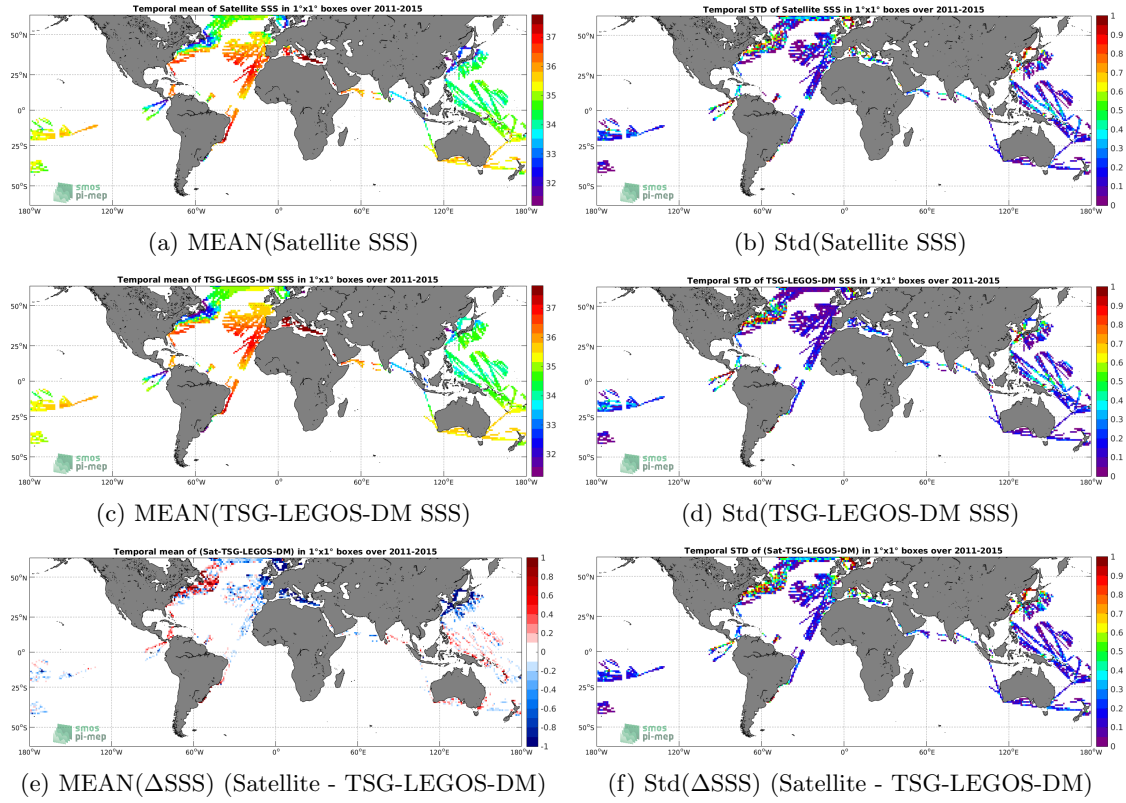
Figure 6: Temporal mean (left) and Std (right) of SSS from Aquarius-L3-OR-V5-7DAY-RUNNING-RAIN-MASK-1DEG (top), TSG-LEGOS-DM (middle), and of \Delta SSS (Satellite - TSG-LEGOS-DM). Only match-up pairs are used to generate these maps.
