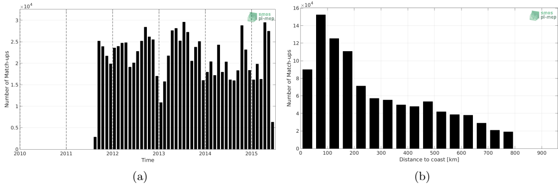
Figure 1: Number of match-ups between TSG-LEGOS-DM and Aquarius-L3-OR-V5-7DAY-RUNNING-RAIN-MASK-1DEG SSS as a function of time (a) and as function of the distance to coast (b) over the SMOS coastal zone ( \approx 800\text{km} ) 60N-60S Pi-MEP region and for the full satellite product period.
