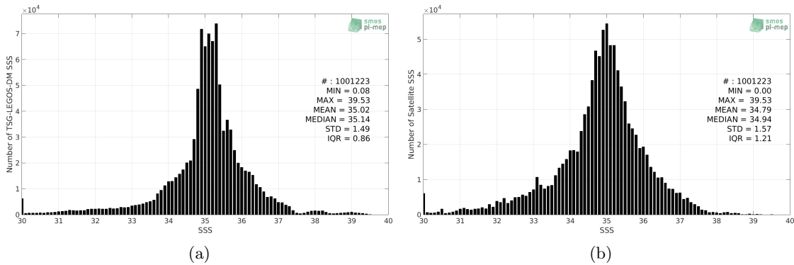
Figure 2: Histograms of SSS from TSG-LEGOS-DM (a) and Aquarius-L3-OR-V5-7DAY-RUNNING-RAIN-MASK-1DEG (b) considering all match-up pairs per bins of 0.1 over the SMOS coastal zone ( \approx 800\text{km} ) 60N-60S Pi-MEP region and for the full satellite product period.
