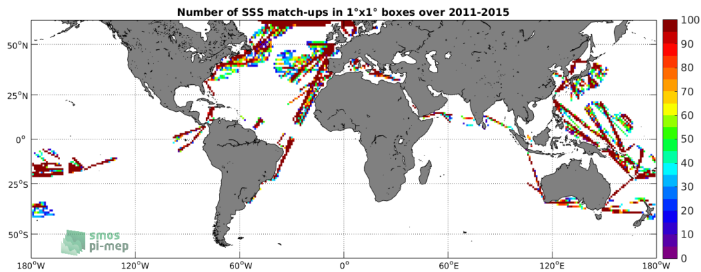
Figure 4: Number of SSS match-ups between TSG-LEGOS-DM SSS and the Aquarius-L3-OR-V5-7DAY-RUNNING-RAIN-MASK-1DEG SSS product for the SMOS coastal zone ( \pm 800\text{km} ) 60N-60S Pi-MEP region over 1^\circ \times 1^\circ boxes and for the full satellite product period.
