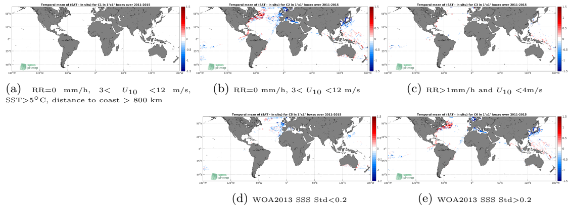
Figure 12: Temporal mean gridded over spatial boxes of size 1^\circ \times 1^\circ of \Delta SSS (Aquarius-L3-OR-V5-7DAY-RUNNING-RAIN-MASK-1DEG - TSG-LEGOS-DM) for 5 different subdatasets corresponding to:RR=0 mm/h, 3 < U_{10} < 12 m/s, SST >5^\circ C, distance to coast > 800 km (a), RR=0 mm/h, 3 < U_{10} < 12 m/s (b), RR >1 mm/h and U_{10} < 4 m/s (c), WOA2013 SSS Std <0.2 (d), WOA2013 SSS Std >0.2 (e).
