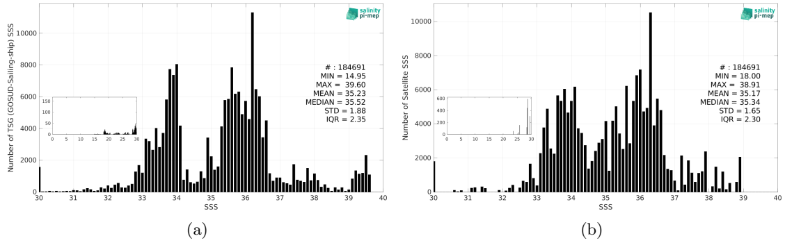
Figure 3: Histograms of SSS from TSG (GOSUD-Sailing-ship) (a) and Aquarius SSS L3 OR v5 - 7-Day running - Rain mask (NASA-GSFC) (b) considering all match-up pairs per bins of 0.1 over the SMOS coastal zone (<800km) 60N-60S Pi-MEP region and for the full satellite product period.
