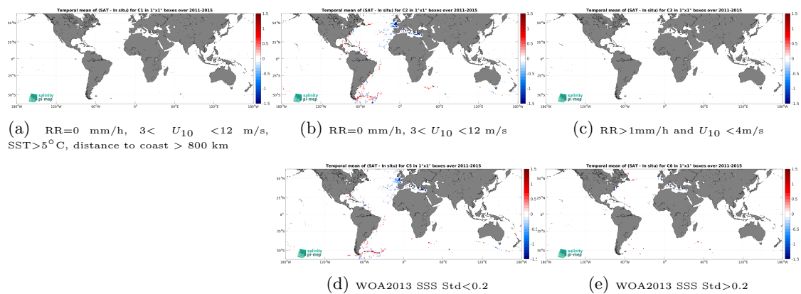
Figure 14: Temporal mean gridded over spatial boxes of size 1^\circ \times 1^\circ of \Delta SSS (Aquarius SSS L3 OR v5 - 7-Day running - Rain mask (NASA-GSFC) - TSG (GOSUD-Sailing-ship)) for 5 different subdatasets corresponding to:RR=0 mm/h, 3 < U_{10} < 12 m/s, SST >5^\circ\text{C} , distance to coast > 800 km (a), RR=0 mm/h, 3 < U_{10} < 12 m/s (b), RR >1 mm/h and U_{10} < 4 m/s (c), WOA2013 SSS Std <0.2 (d), WOA2013 SSS Std >0.2 (e).
