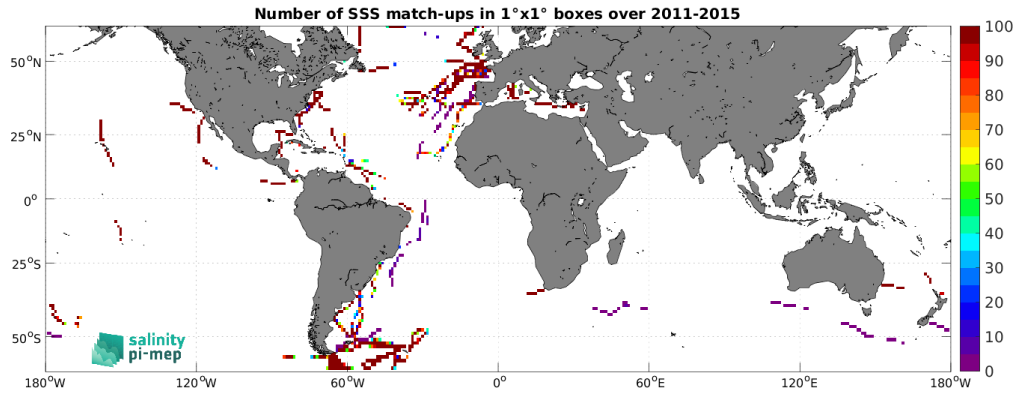
Figure 5: Number of SSS match-ups between TSG (GOSUD-Sailing-ship) SSS and the Aquarius SSS L3 OR v5 - 7-Day running - Rain mask (NASA-GSFC) SSS product for the SMOS coastal zone (<800km) 60N-60S Pi-MEP region over 1^\circ \times 1^\circ boxes and for the full satellite product period.
