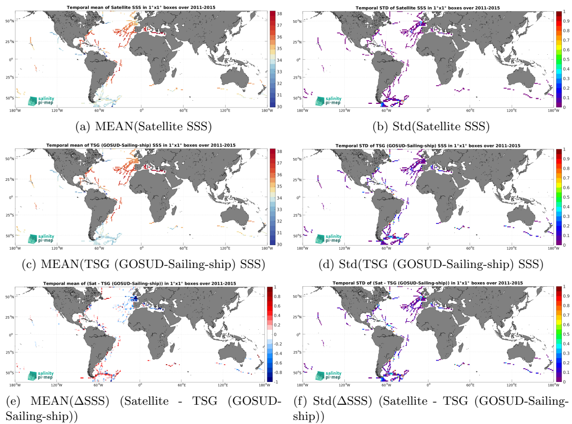
Figure 7: Temporal mean (left) and Std (right) of SSS from Aquarius SSS L3 OR v5 - 7-Day running - Rain mask (NASA-GSFC) (top), TSG (GOSUD-Sailing-ship) (middle), and of \Delta SSS (Satellite - TSG (GOSUD-Sailing-ship)). Only match-up pairs are used to generate these maps.
