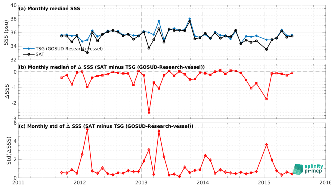
Figure 8: Time series of the monthly median SSS (top), median of \Delta SSS (Satellite - TSG (GOSUD-Research-vessel)) and Std of \Delta SSS (Satellite - TSG (GOSUD-Research-vessel)) over the SMOS coastal zone (<800km) 60N-60S Pi-MEP region considering all match-ups collected by the Pi-MEP.
