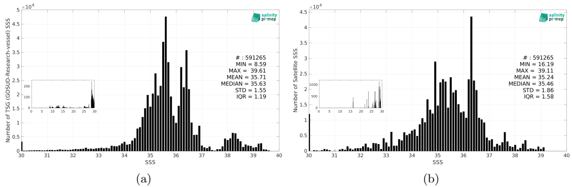
Figure 3: Histograms of SSS from TSG (GOSUD-Research-vessel) (a) and Aquarius SSS L3 OR v5 - 7-Day running - Rain mask (NASA-GSFC) (b) considering all match-up pairs per bins of 0.1 over the SMOS coastal zone (<800km) 60N-60S Pi-MEP region and for the full satellite product period.
