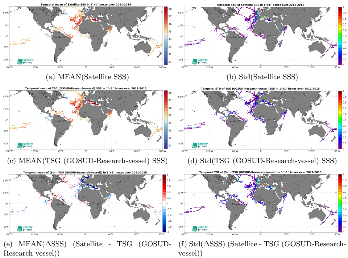
Figure 7: Temporal mean (left) and Std (right) of SSS from Aquarius SSS L3 OR v5 - 7-Day running - Rain mask (NASA-GSFC) (top), TSG (GOSUD-Research-vessel) (middle), and of \Delta SSS (Satellite - TSG (GOSUD-Research-vessel)). Only match-up pairs are used to generate these maps.
