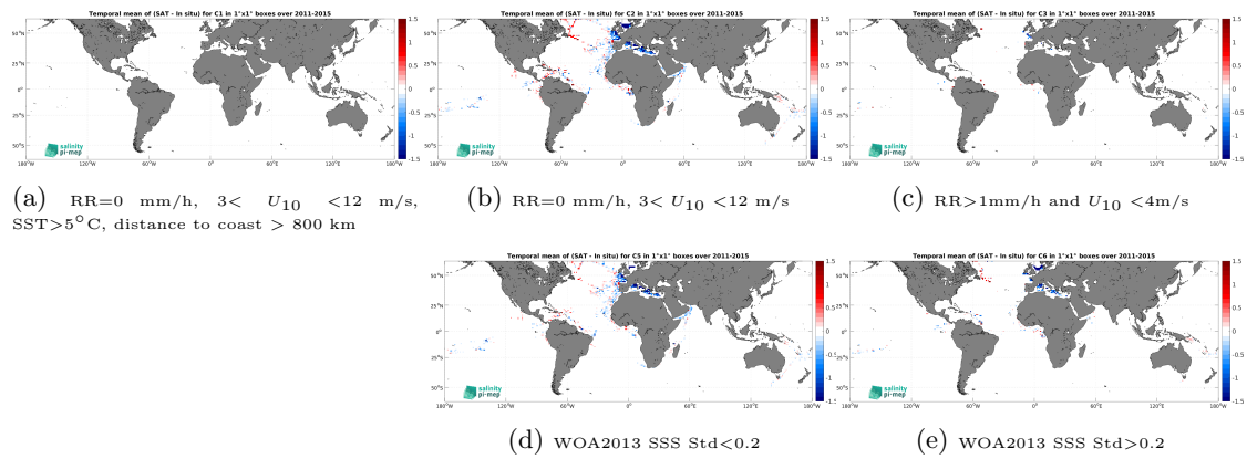
Figure 14: Temporal mean gridded over spatial boxes of size 1^\circ \times 1^\circ of \Delta\text{SSS} (Aquarius SSS L3 OR v5 - 7-Day running - Rain mask (NASA-GSFC) - TSG (GOSUD-Research-vessel)) for 5 different subdatasets corresponding to: RR=0 mm/h, 3 < U_{10} < 12 m/s, SST > 5^\circ\text{C} , distance to coast > 800 km (a), RR=0 mm/h, 3 < U_{10} < 12 m/s (b), RR > 1 mm/h and U_{10} < 4 m/s (c), WOA2013 SSS Std < 0.2 (d), WOA2013 SSS Std > 0.2 (e).
