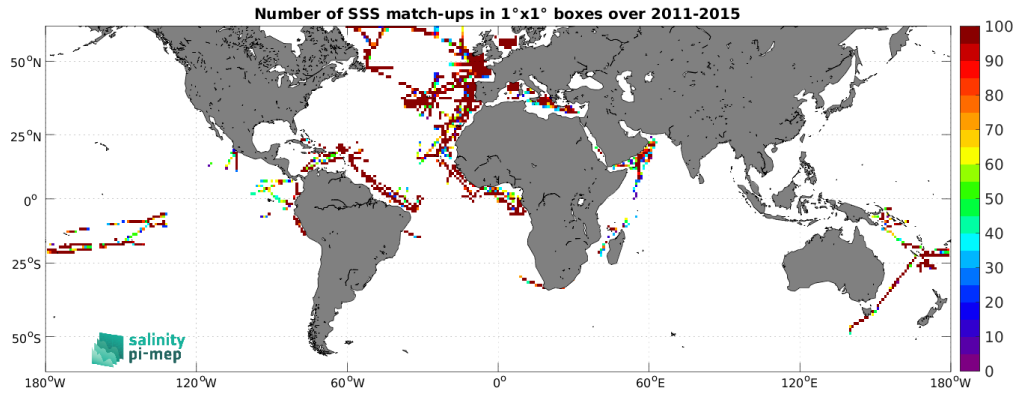
Figure 5: Number of SSS match-ups between TSG (GOSUD-Research-vessel) SSS and the Aquarius SSS L3 OR v5 - 7-Day running - Rain mask (NASA-GSFC) SSS product for the SMOS coastal zone (<800km) 60N-60S Pi-MEP region over 1^\circ \times 1^\circ boxes and for the full satellite product period.
