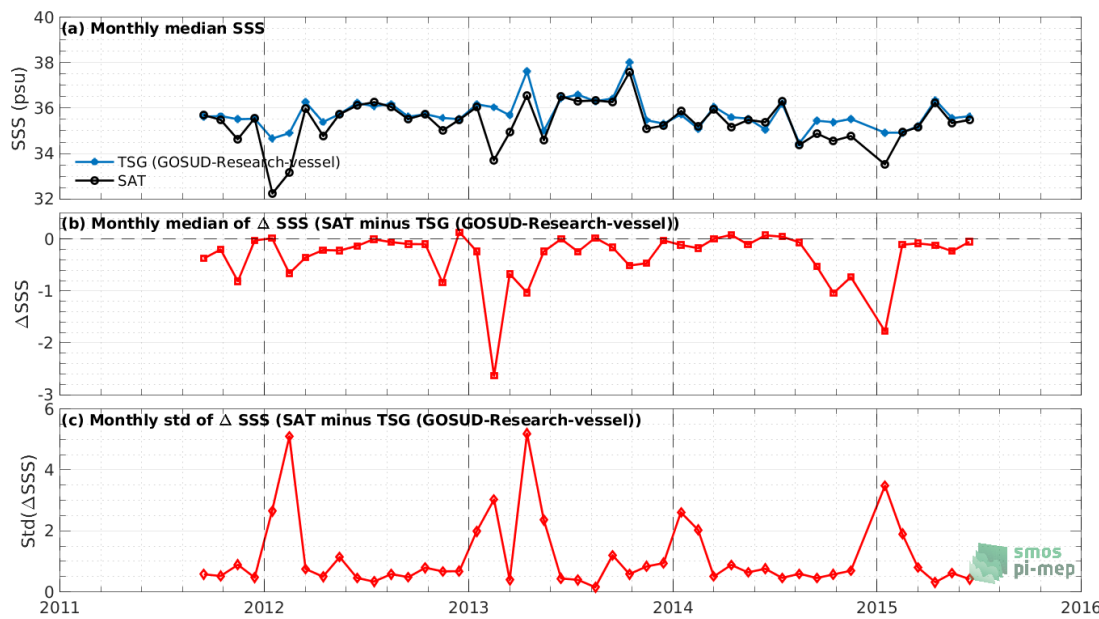
Figure 7: Time series of the monthly median SSS (top), median of \Delta SSS (Satellite - TSG (GOSUD-Research-vessel)) and Std of \Delta SSS (Satellite - TSG (GOSUD-Research-vessel)) over the SMOS coastal zone (<800km) 60N-60S Pi-MEP region considering all match-ups collected by the Pi-MEP.
