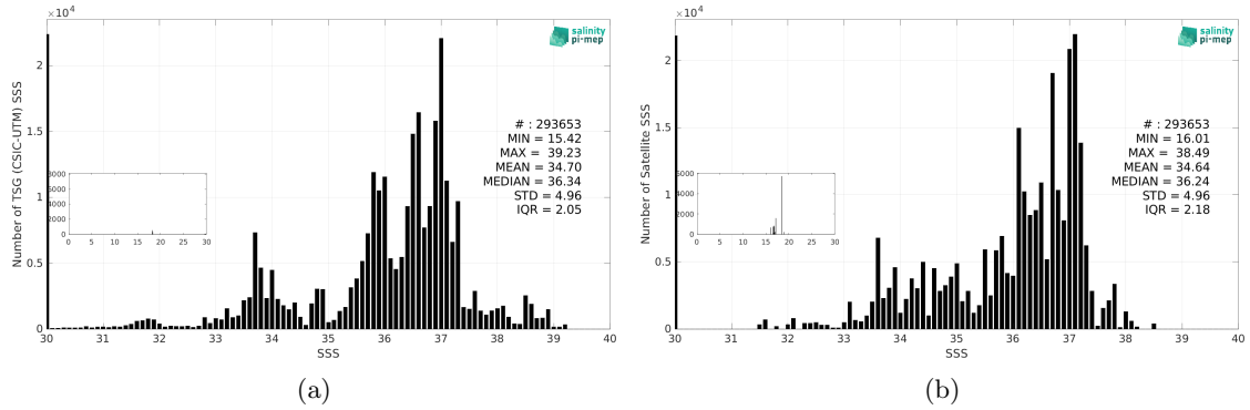
Figure 3: Histograms of SSS from TSG (CSIC-UTM) (a) and Aquarius SSS L3 OR v5 - 7-Day running - Rain mask (NASA-GSFC) (b) considering all match-up pairs per bins of 0.1 over the SMOS coastal zone (<800km) 60N-60S Pi-MEP region and for the full satellite product period.
