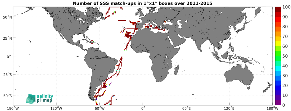
Figure 5: Number of SSS match-ups between TSG (CSIC-UTM) SSS and the Aquarius SSS L3 OR v5 - 7-Day running - Rain mask (NASA-GSFC) SSS product for the SMOS coastal zone (<800km) 60N-60S Pi-MEP region over 1^\circ \times 1^\circ boxes and for the full satellite product period.
