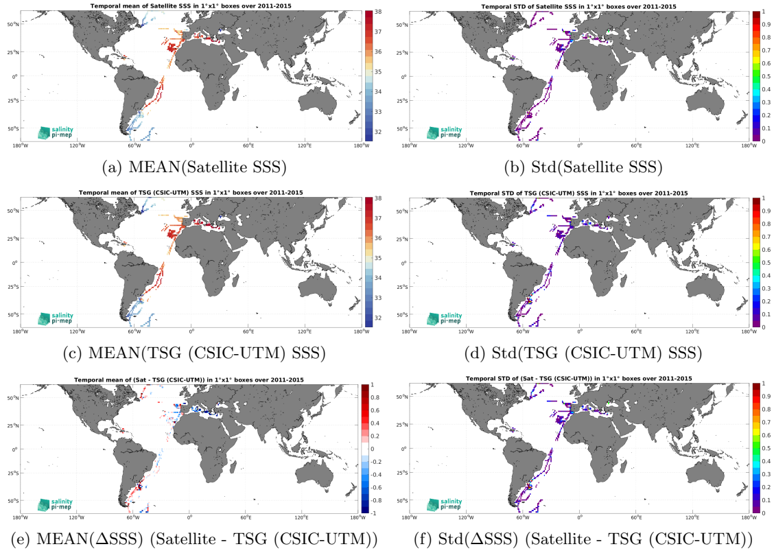
Figure 7: Temporal mean (left) and Std (right) of SSS from Aquarius SSS L3 OR v5 - 7-Day running - Rain mask (NASA-GSFC) (top), TSG (CSIC-UTM) (middle), and of \Delta\text{SSS} (Satellite - TSG (CSIC-UTM)). Only match-up pairs are used to generate these maps.
