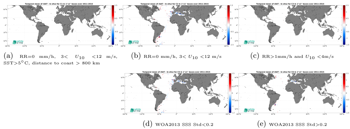
Figure 14: Temporal mean gridded over spatial boxes of size 1^\circ \times 1^\circ of \Delta SSS (Aquarius SSS L3 OR v5 - 7-Day running - Rain mask (NASA-GSFC) - TSG (CSIC-UTM)) for 5 different subdatasets corresponding to: RR=0 mm/h, 3 < U_{10} < 12 m/s, SST > 5^\circ\text{C} , distance to coast > 800 km (a), RR=0 mm/h, 3 < U_{10} < 12 m/s (b), RR > 1 mm/h and U_{10} < 4 m/s (c), WOA2013 SSS Std < 0.2 (d), WOA2013 SSS Std > 0.2 (e).
