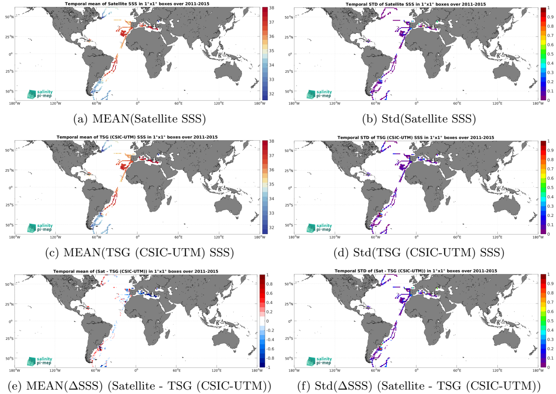
Figure 6: Temporal mean (left) and Std (right) of SSS from Aquarius SSS L3 OR v5 - 7-Day running - Rain mask (NASA-GSFC) (top), TSG (CSIC-UTM) (middle), and of \Delta\text{SSS} (Satellite - TSG (CSIC-UTM)). Only match-up pairs are used to generate these maps.
