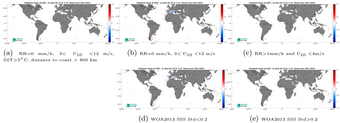
Figure 12: Temporal mean gridded over spatial boxes of size 1^\circ \times 1^\circ of \Delta SSS (Aquarius SSS L3 OR v5 - 7-Day running - Rain mask (NASA-GSFC) - TSG (CSIC-UTM)) for 5 different subdatasets corresponding to:RR=0 mm/h, 3 < U_{10} < 12 m/s, SST >5^\circ C, distance to coast > 800 km (a), RR=0 mm/h, 3 < U_{10} < 12 m/s (b), RR >1 mm/h and U_{10} < 4 m/s (c), WOA2013 SSS Std <0.2 (d), WOA2013 SSS Std >0.2 (e).
