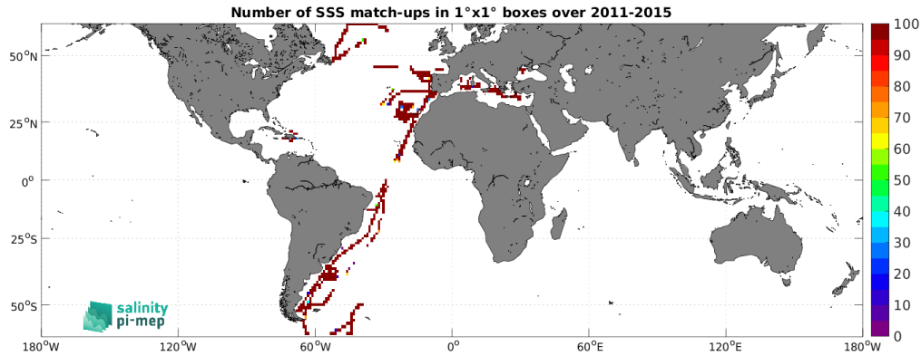
Figure 4: Number of SSS match-ups between TSG (CSIC-UTM) SSS and the Aquarius SSS L3 OR v5 - 7-Day running - Rain mask (NASA-GSFC) SSS product for the SMOS coastal zone (<800km) 60N-60S Pi-MEP region over 1^\circ \times 1^\circ boxes and for the full satellite product period.
