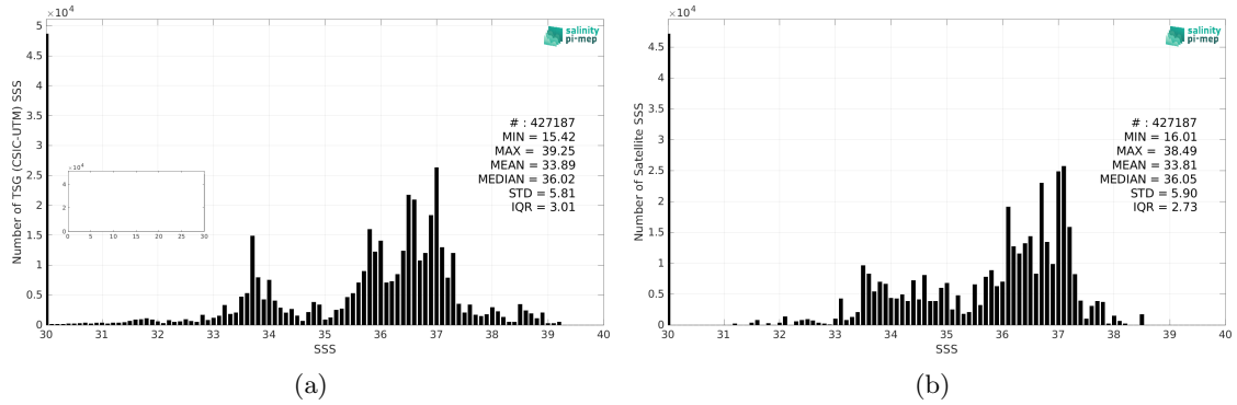
Figure 2: Histograms of SSS from TSG (CSIC-UTM) (a) and Aquarius SSS L3 OR v5 - 7-Day running - Rain mask (NASA-GSFC) (b) considering all match-up pairs per bins of 0.1 over the SMOS coastal zone (<800km) 60N-60S Pi-MEP region and for the full satellite product period.
