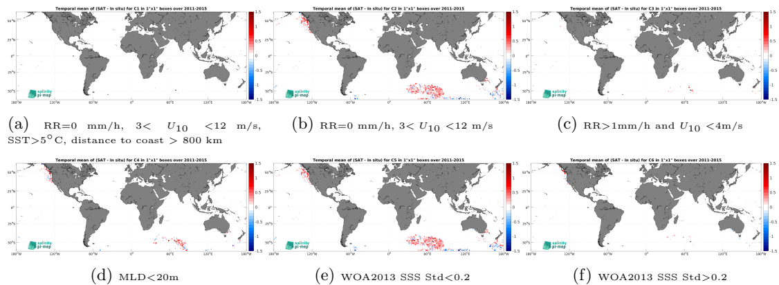
Figure 14: Temporal mean gridded over spatial boxes of size 1^\circ \times 1^\circ of \Delta SSS (Aquarius SSS L3 OR v5 - 7-Day running - Rain mask (NASA-GSFC) - Marine mammals) for 6 different subdatasets corresponding to:RR=0 mm/h, 3 < U_{10} < 12 m/s, SST > 5^\circ\text{C} , distance to coast > 800 km (a), RR=0 mm/h, 3 < U_{10} < 12 m/s (b), RR > 1 mm/h and U_{10} < 4 m/s (c),MLD < 20 m (d),WOA2013 SSS Std < 0.2 (e),WOA2013 SSS Std > 0.2 (f).
