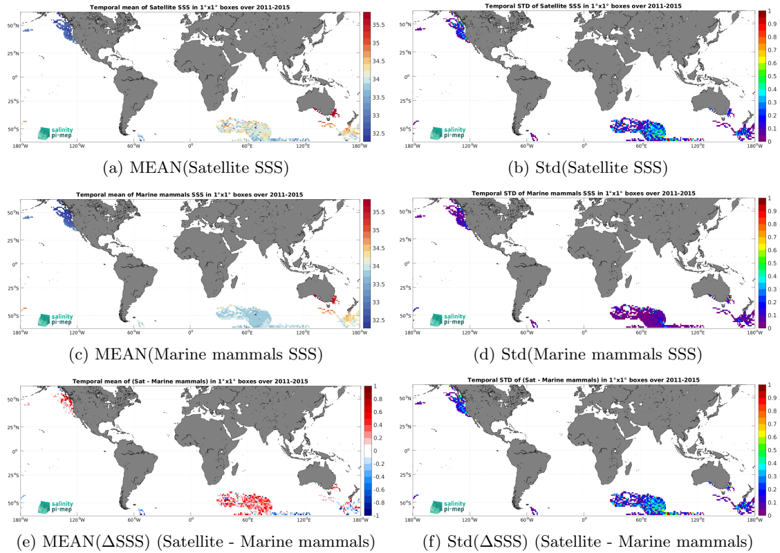
Figure 7: Temporal mean (left) and Std (right) of SSS from Aquarius SSS L3 OR v5 - 7-Day running - Rain mask (NASA-GSFC) (top), Marine mammals (middle), and of \Delta SSS (Satellite - Marine mammals). Only match-up pairs are used to generate these maps.
