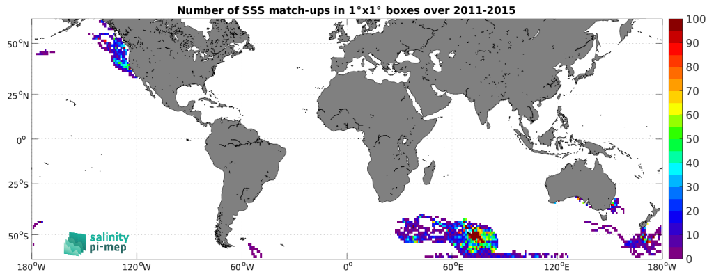
Figure 5: Number of SSS match-ups between Marine mammals SSS and the Aquarius SSS L3 OR v5 - 7-Day running - Rain mask (NASA-GSFC) SSS product for the SMOS coastal zone (<800km) 60N-60S Pi-MEP region over 1°x1° boxes and for the full satellite product period.
