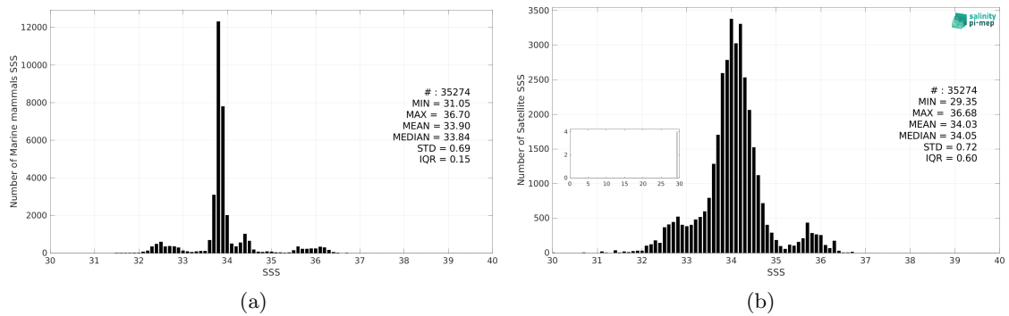
Figure 3: Histograms of SSS from Marine mammals (a) and Aquarius SSS L3 OR v5 - 7-Day running - Rain mask (NASA-GSFC) (b) considering all match-up pairs per bins of 0.1 over the SMOS coastal zone (<800km) 60N-60S Pi-MEP region and for the full satellite product period.
